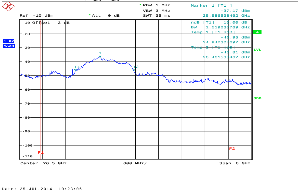
Plot 1: 10 dB emission bandwidth, T_{\text{nom}} / V_{\text{nom}}
