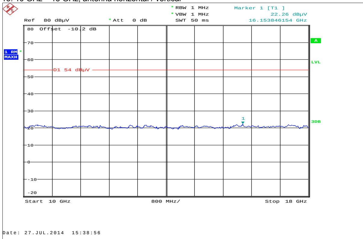
Plot 13: 10 GHz – 18 GHz, antenna horizontal / vertical
