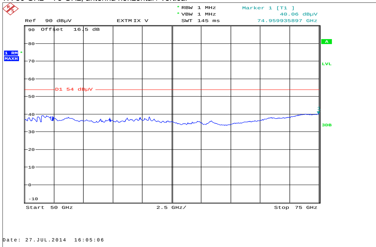
Plot 17: 50 GHz – 75 GHz, antenna horizontal / vertical
