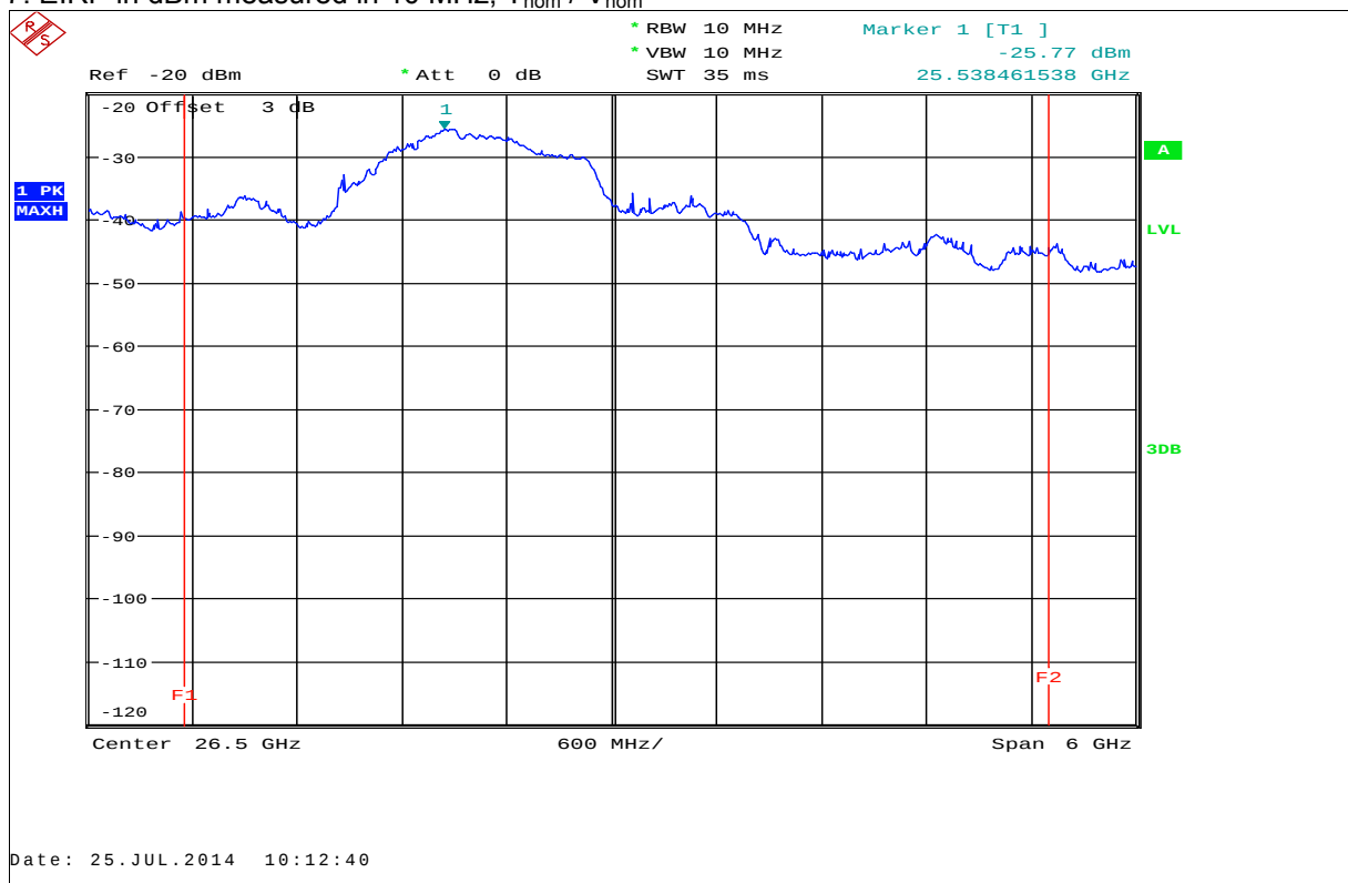
Plot 7: EIRP in dBm measured in 10 MHz, T_{\text{nom}} / V_{\text{nom}}
