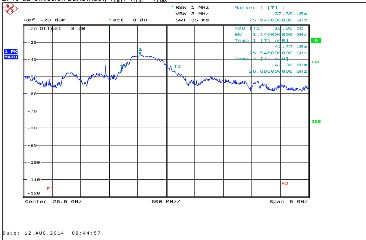
Plot 2: 10 dB emission bandwidth, T_{\text{min}} / V_{\text{min}} - V_{\text{max}}
