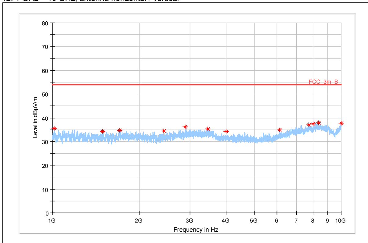
Plot 12: 1 GHz – 10 GHz, antenna horizontal / vertical
