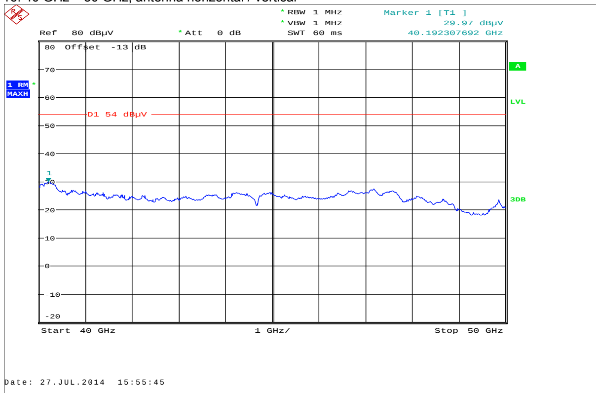
Plot 16: 40 GHz – 50 GHz, antenna horizontal / vertical
