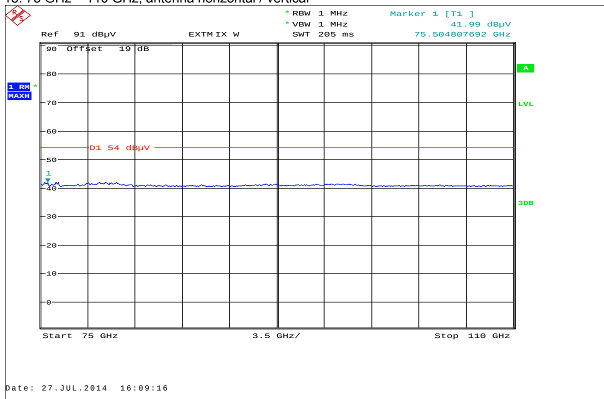
Plot 18: 75 GHz – 110 GHz, antenna horizontal / vertical
