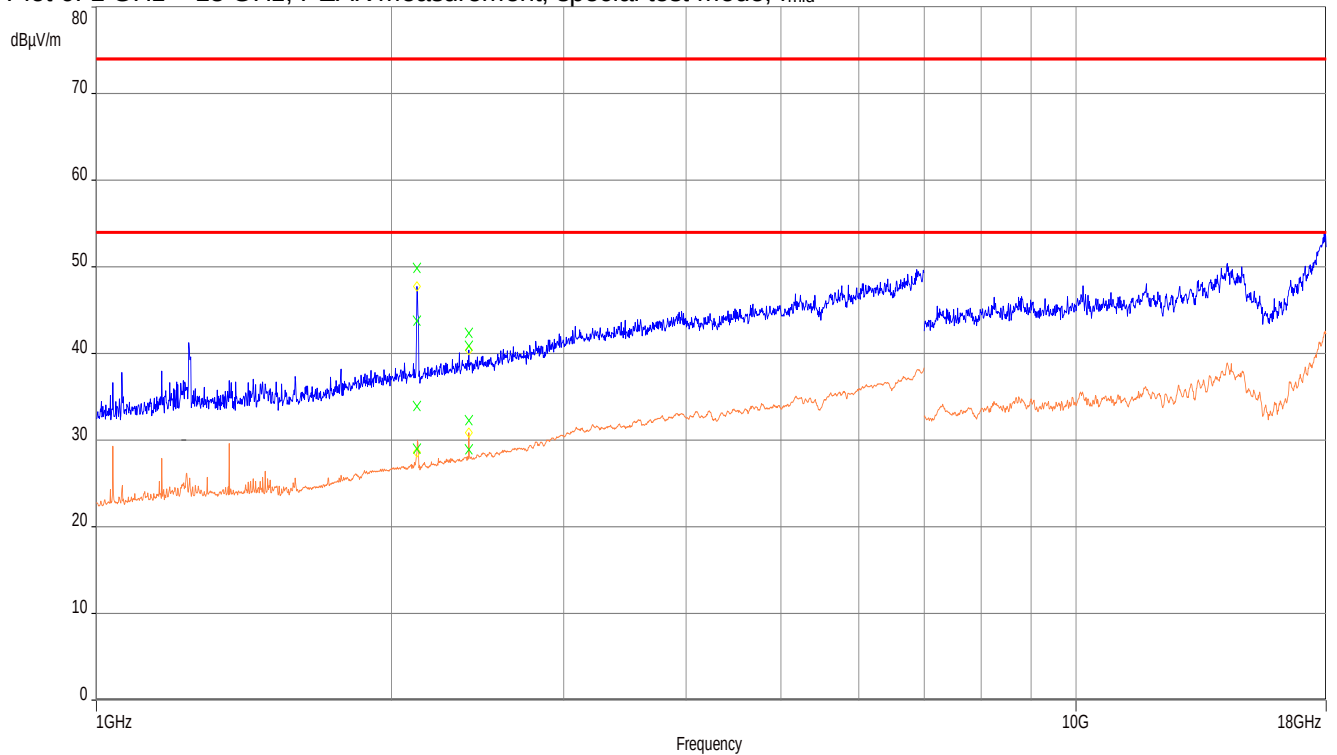
Plot 6: 1 GHz – 18 GHz, PEAK measurement, special test mode, f_{mid}
