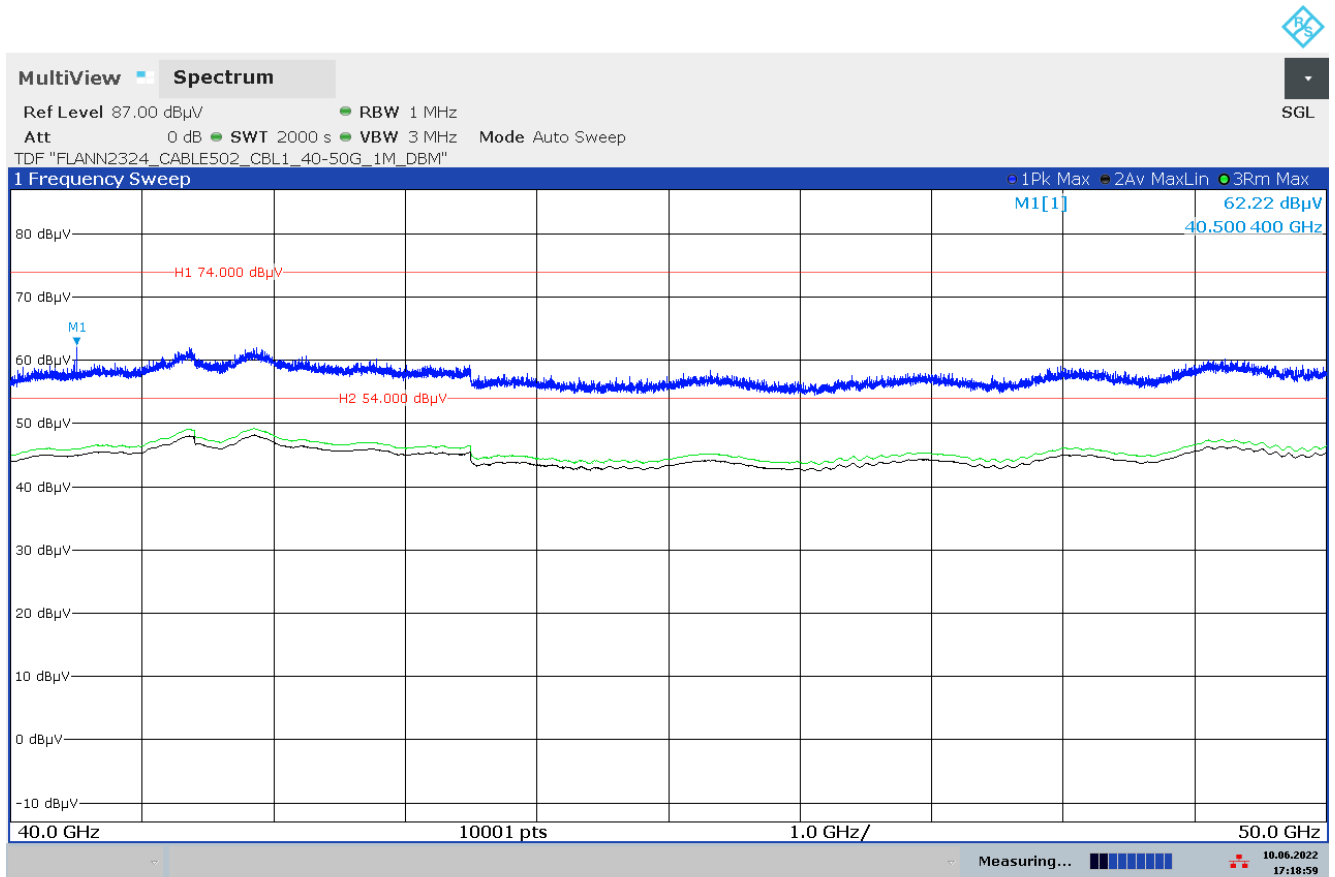
Plot 9: 40 GHz – 50 GHz, PEAK/RMS-measurement, f_{\text{low}}/f_{\text{mid}}/f_{\text{high}}
