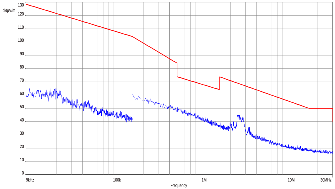
Plot 1: 9 kHz – 30 MHz, special test mode, f_{low}/f_{mid}/f_{high}
