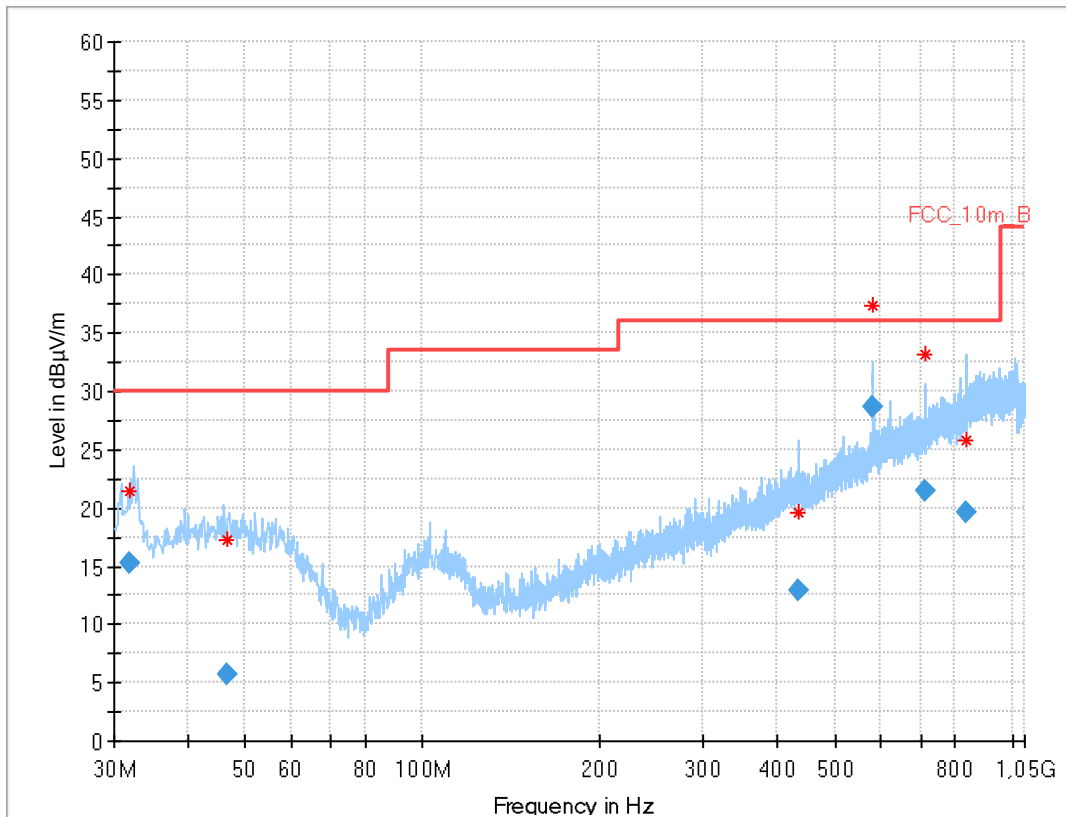
Plot 4: 30 MHz – 1000 MHz, special test mode, f_{\text{high}}
