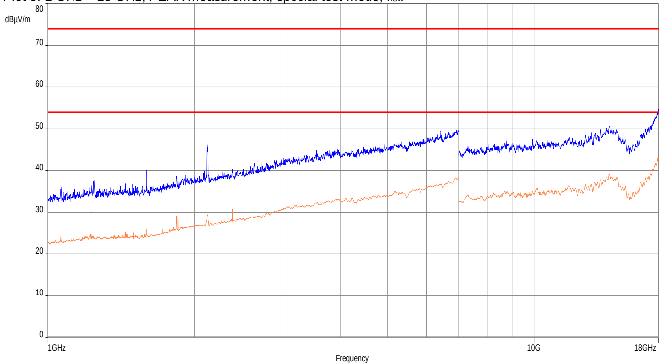
Plot 5: 1 GHz – 18 GHz, PEAK measurement, special test mode, f_{low}
