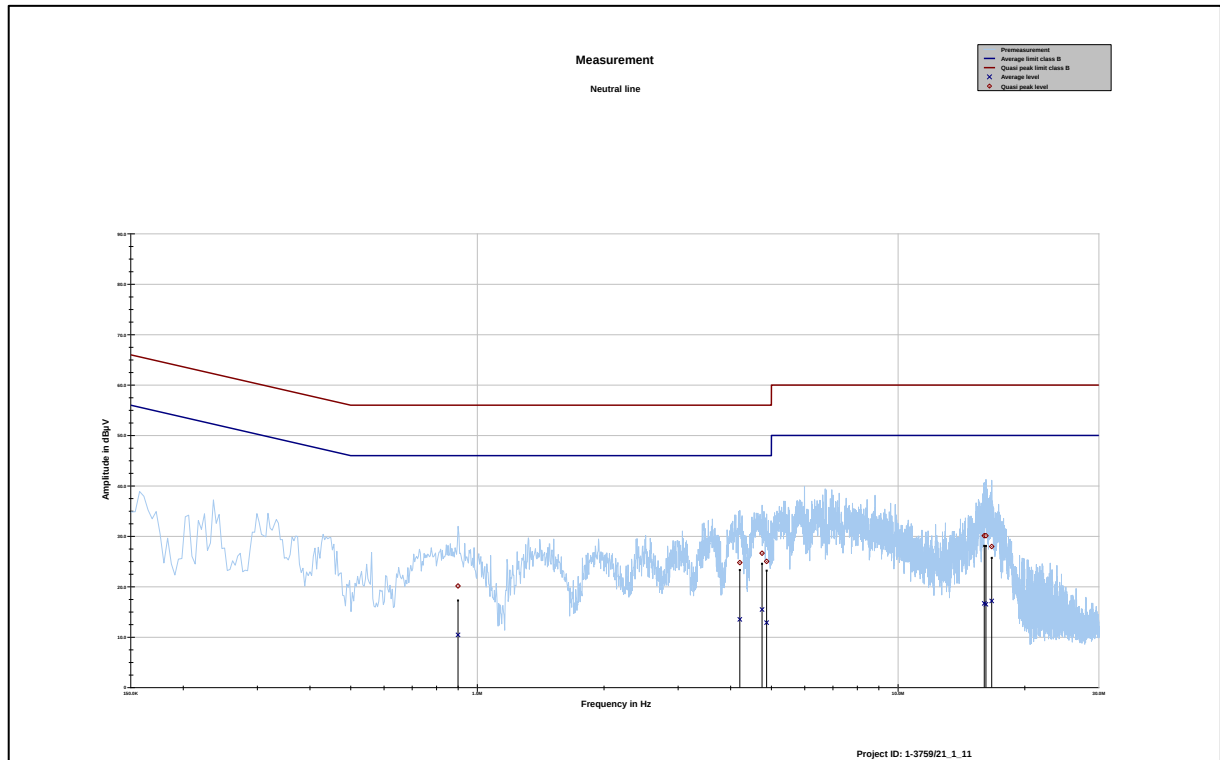
Plot 18: Neutral line
