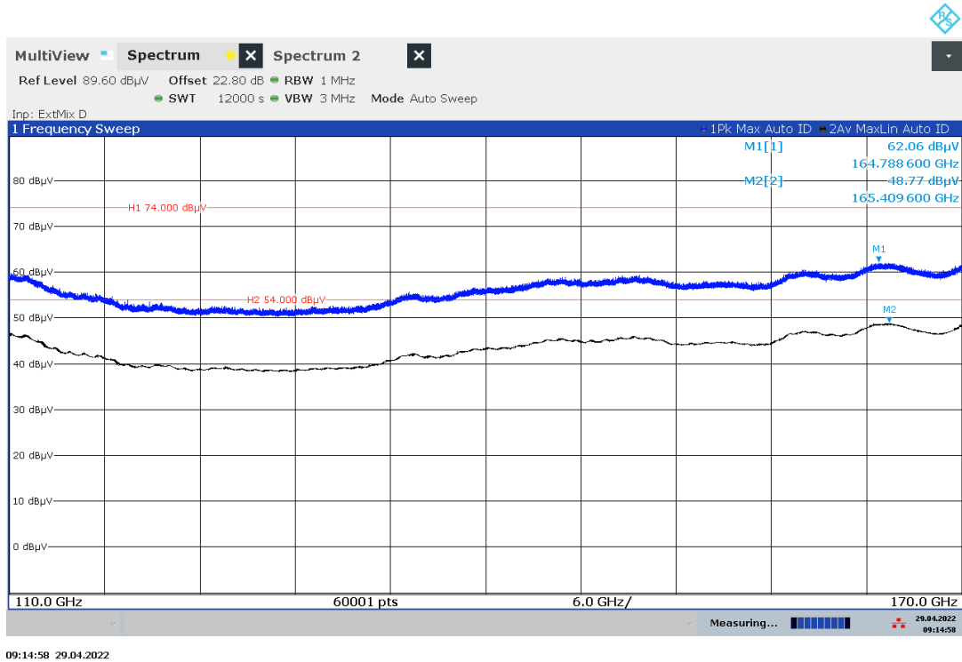
Plot 15: 110 GHz – 170 GHz, PEAK/RMS-measurement, f_{\text{low}}/f_{\text{mid}}/f_{\text{high}}
