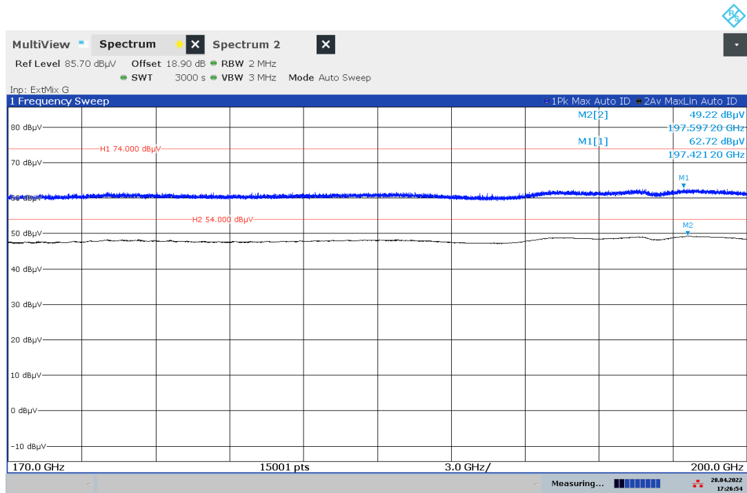
Plot 16: 170 GHz – 200 GHz, PEAK/RMS-measurement, f_{low}/f_{mid}/f_{high}
