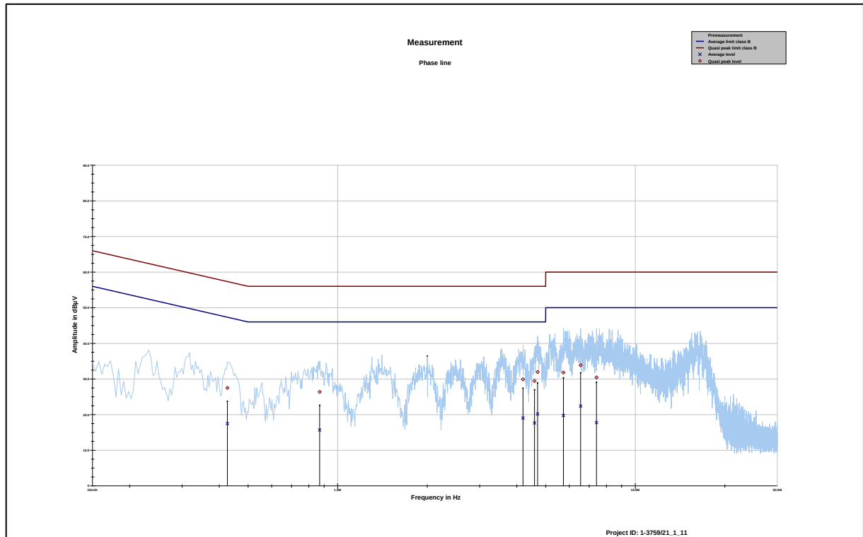
Plot 17: Phase line
