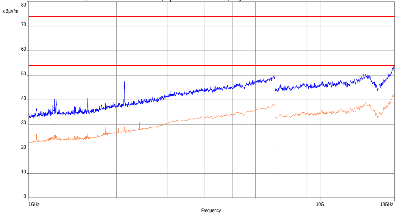
Plot 7: 1 GHz – 18 GHz, PEAK measurement, special test mode, f_{high}
