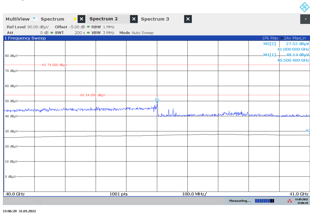
Plot 10: 40 GHz, PEAK/RMS-measurement
