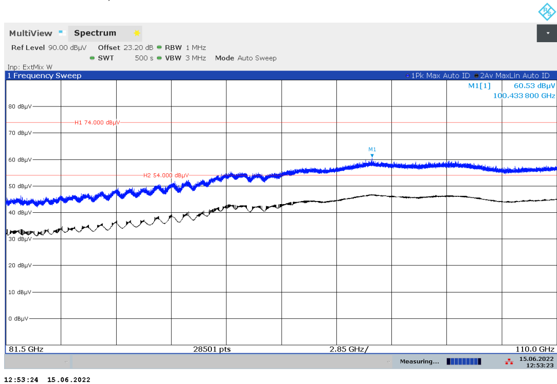
Plot 13: 81 GHz – 110 GHz, PEAK/RMS-measurement
