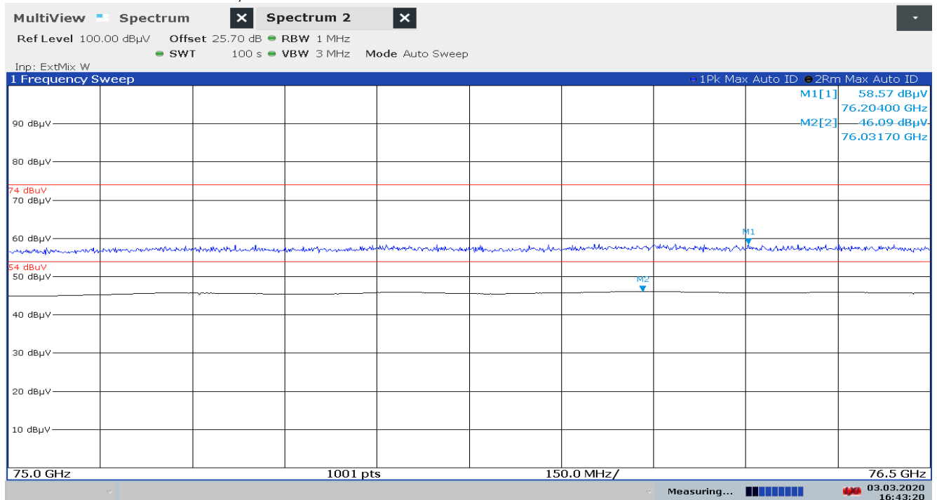
Plot 11: 75 GHz – 76.5 GHz, PEAK/RMS-measurement
