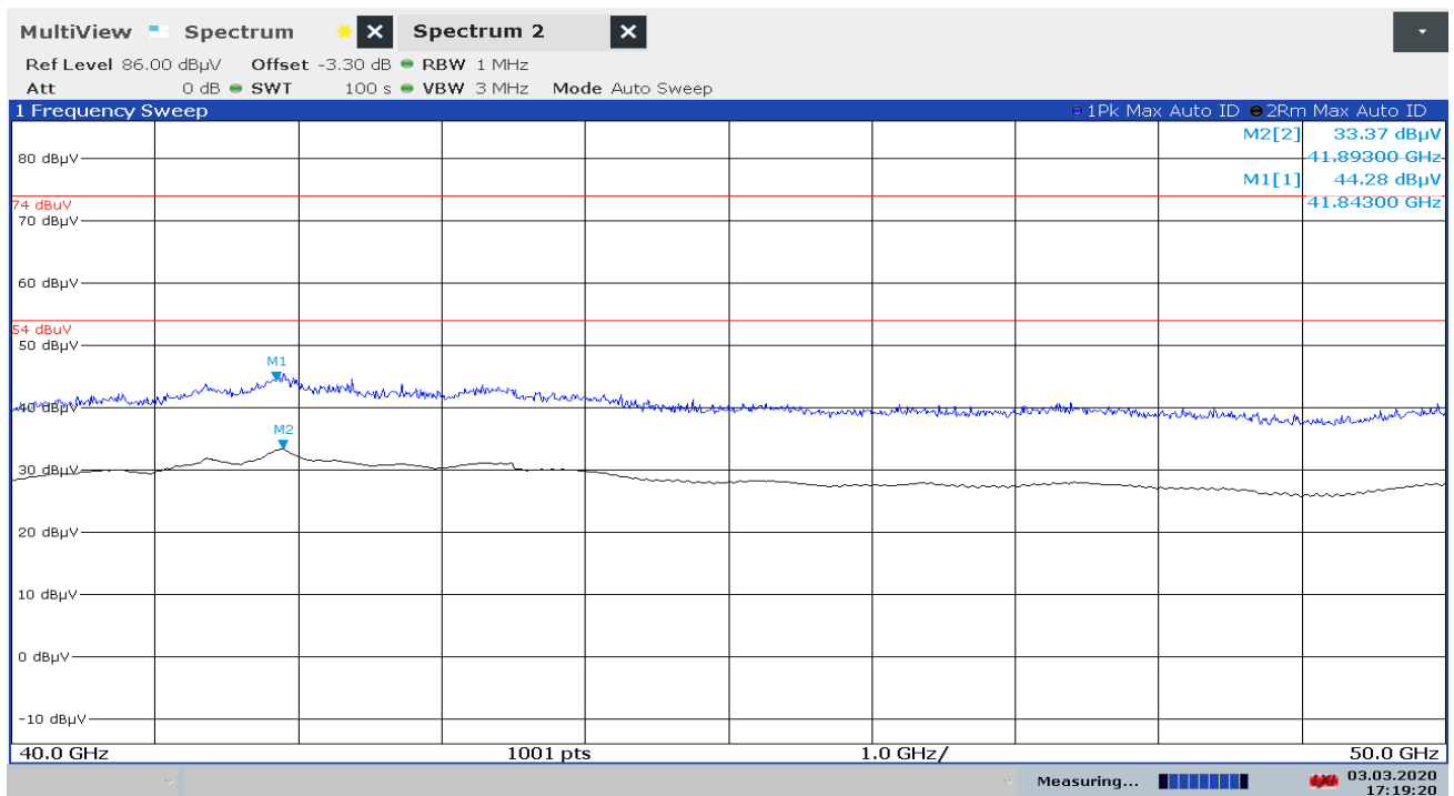
Plot 9: 40 GHz – 50 GHz, PEAK/RMS-measurement
