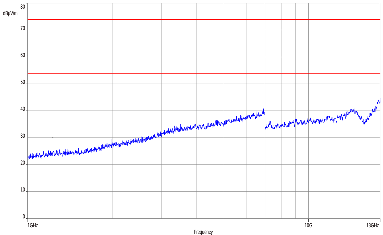
Plot 6: 1 GHz – 18 GHz, PEAK-measurement
