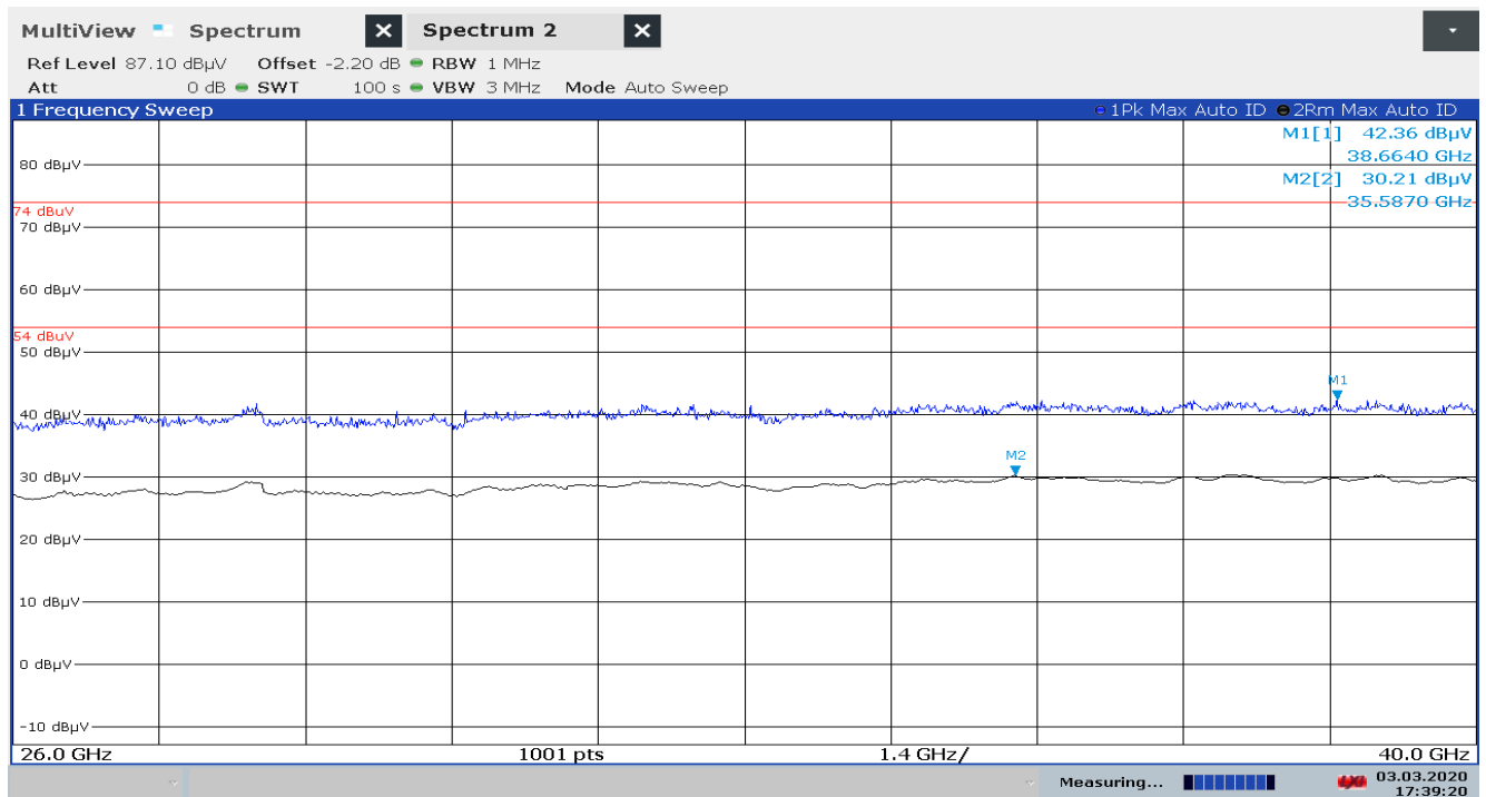
Plot 8: 26 GHz – 40 GHz, PEAK/RMS-measurement
