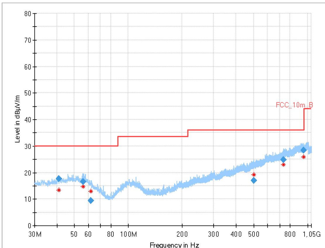
Plot 5: 30 MHz – 1000 MHz
