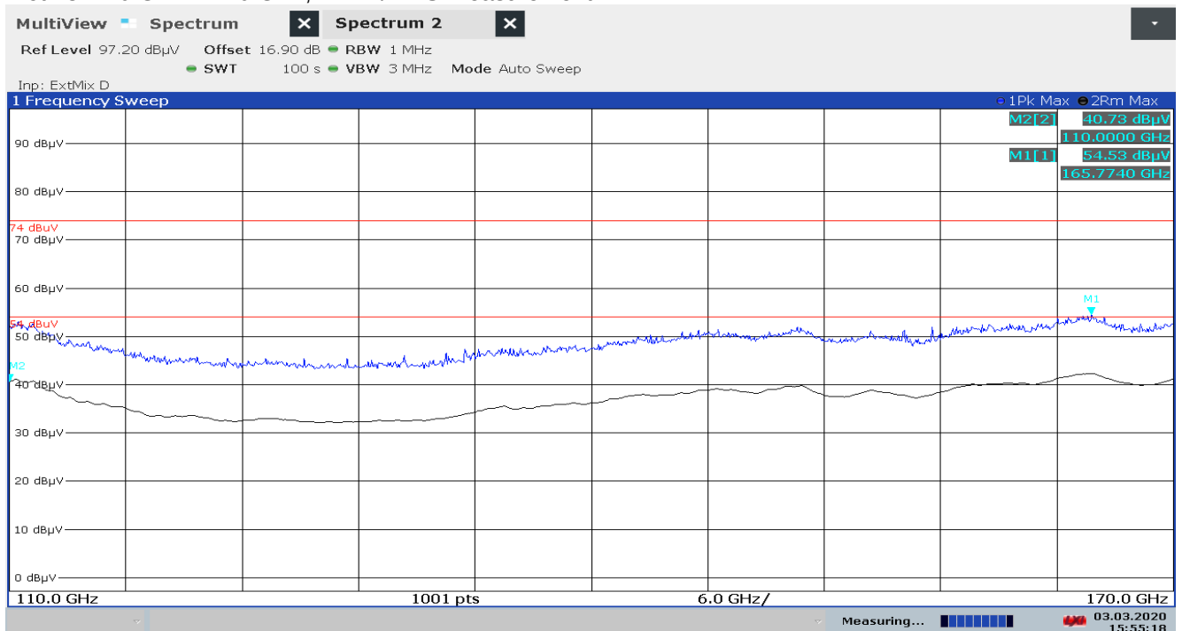
Plot 13: 110 GHz – 170 GHz, PEAK/RMS-measurement
