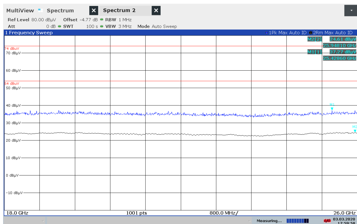
Plot 7: 18 GHz – 26 GHz, PEAK/RMS-measurement
