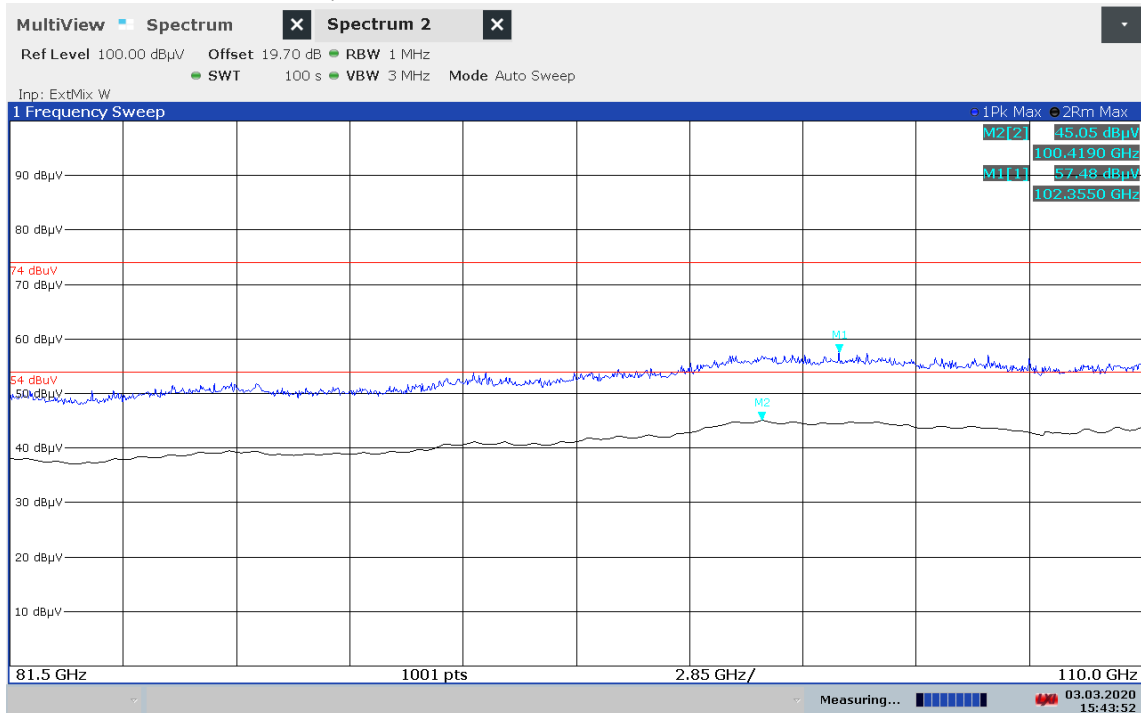
Plot 12: 81 GHz – 110 GHz, PEAK/RMS-measurement
