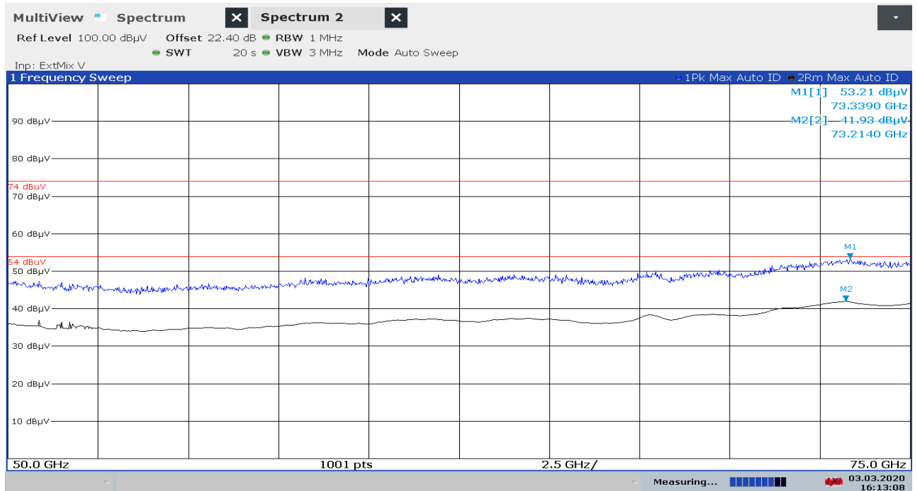
Plot 10: 50 GHz – 75 GHz, PEAK/RMS-measurement
