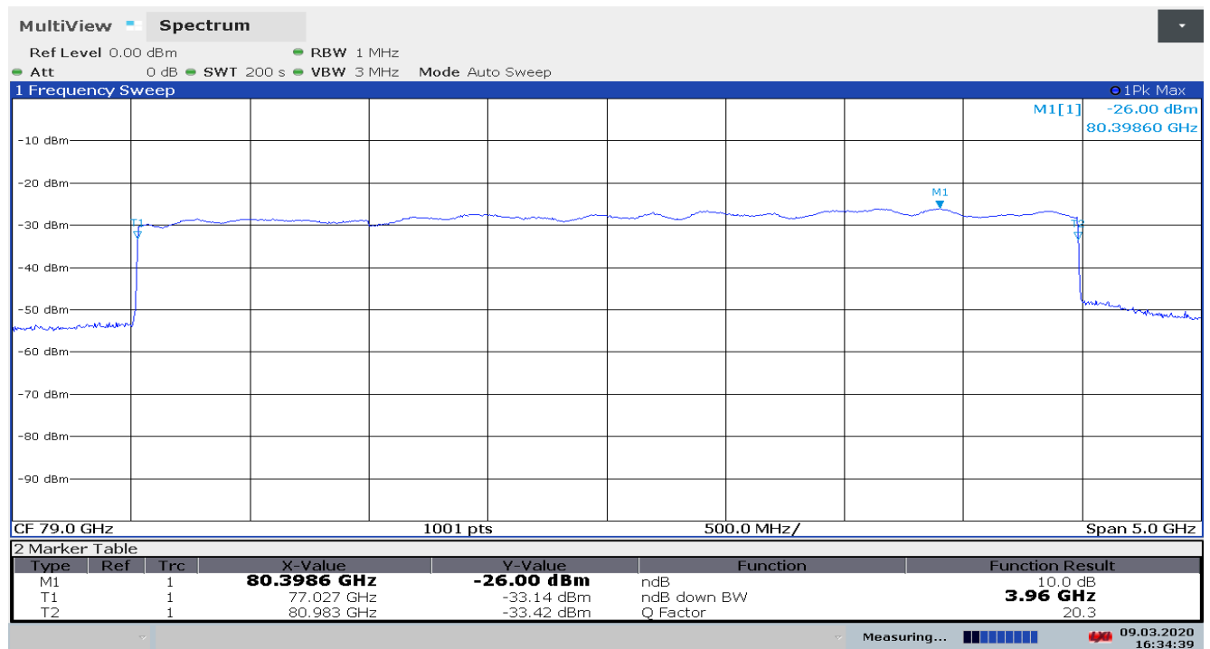
Plot 1: 10 dB bandwidth, Pos-Peak measurement, reference at 20°C
