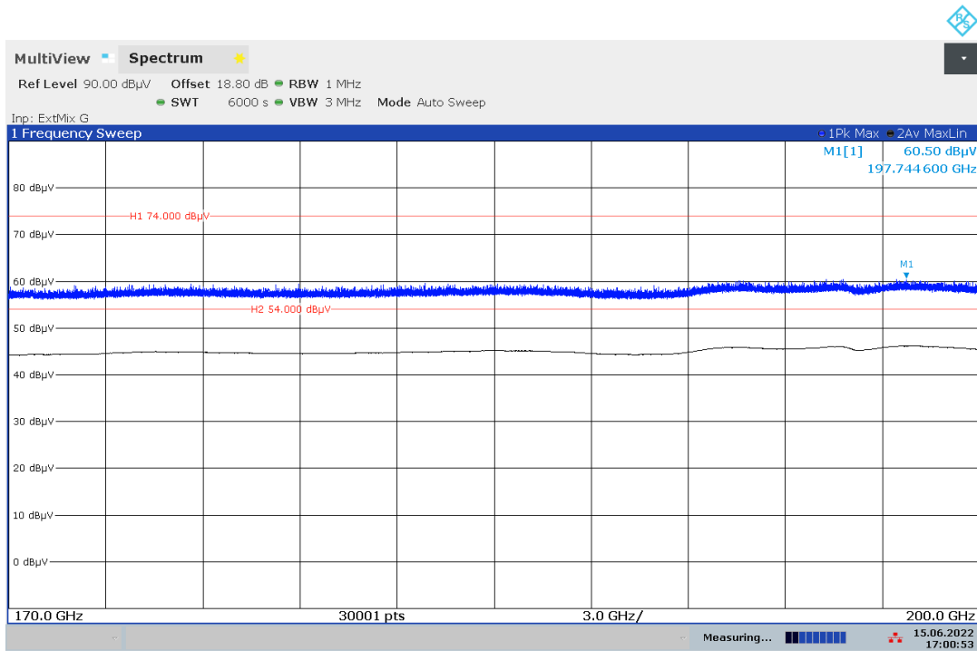
Plot 13: 170 GHz – 200 GHz, PEAK/RMS-measurement
