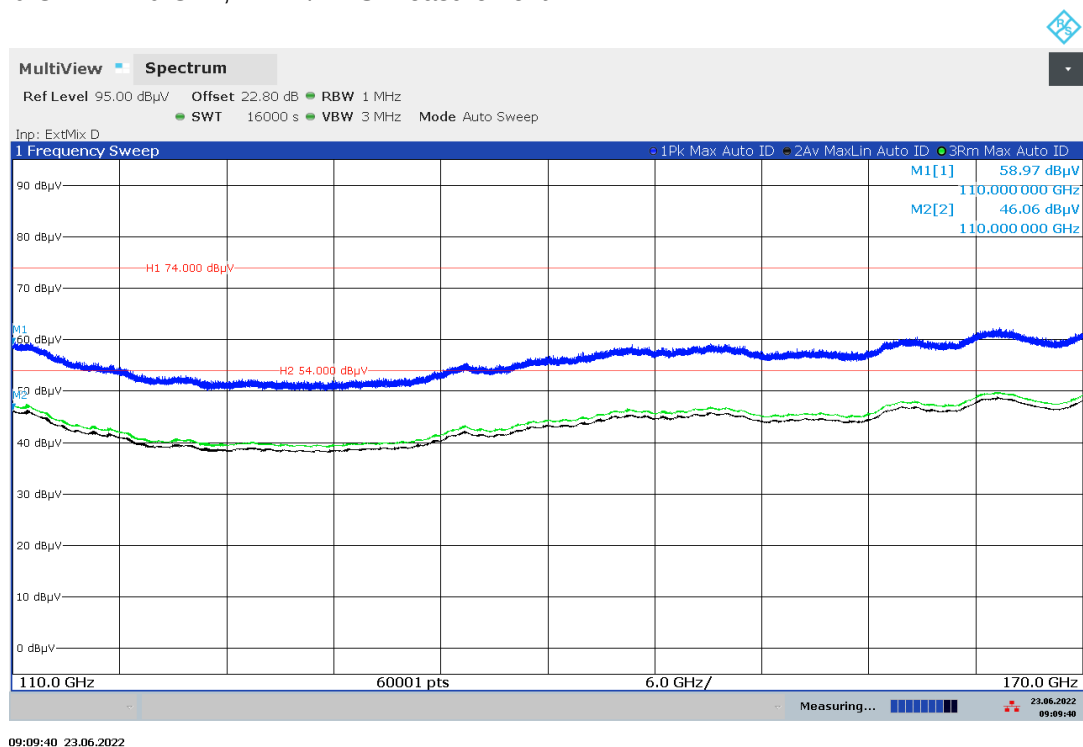
Plot 12: 110 GHz – 170 GHz, PEAK/RMS-measurement
