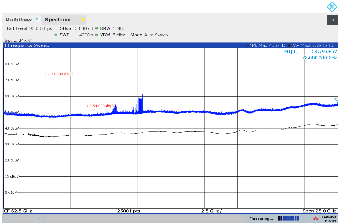
Plot 9: 50 GHz – 75 GHz, PEAK/RMS-measurement
