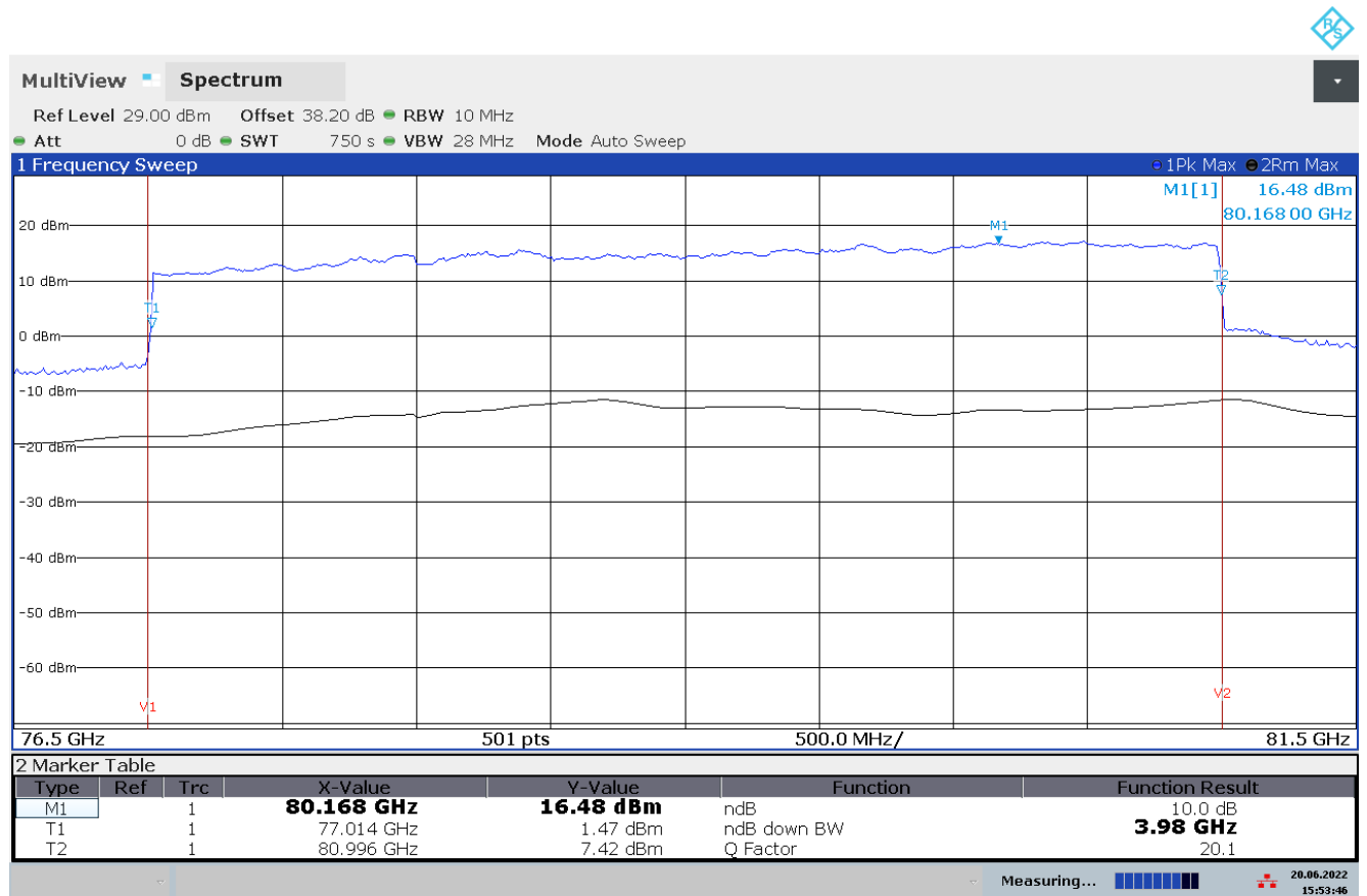
Plot 1: 10 dB bandwidth, Pos-Peak measurement, reference at 20°
