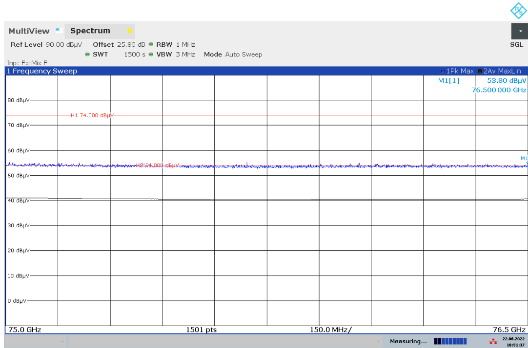
Plot 10: 75 GHz – 76.5 GHz, PEAK/RMS-measurement
