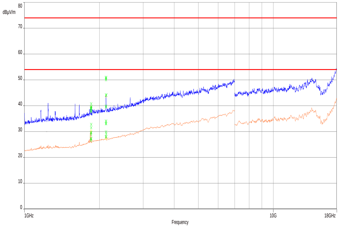
Plot 6: 1 GHz – 18 GHz, PEAK/RMS-measurement
