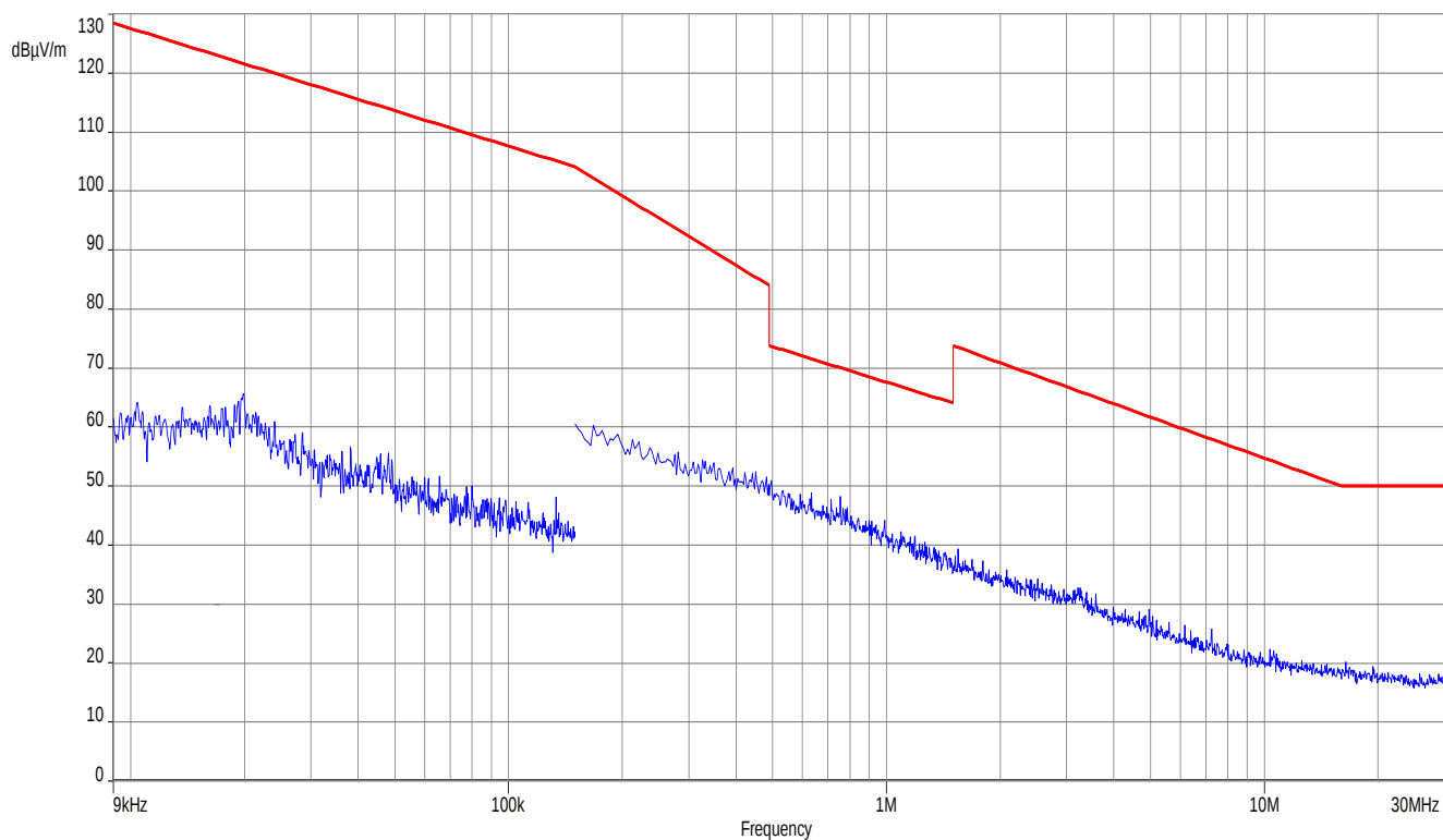
Plot 4: 9 kHz – 30 MHz
