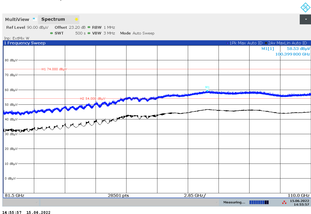
Plot 11: 81 GHz – 110 GHz, PEAK/RMS-measurement
