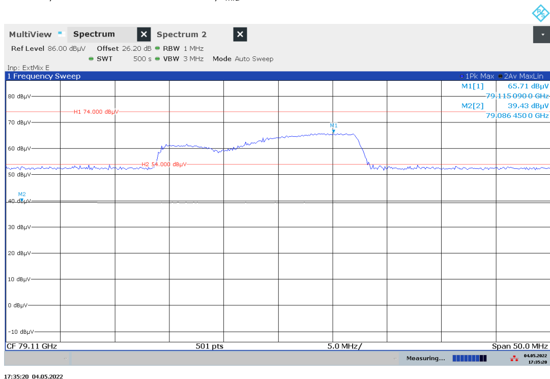
Plot 14: 79.1 GHz, PEAK/RMS-measurement, f_{mid}
