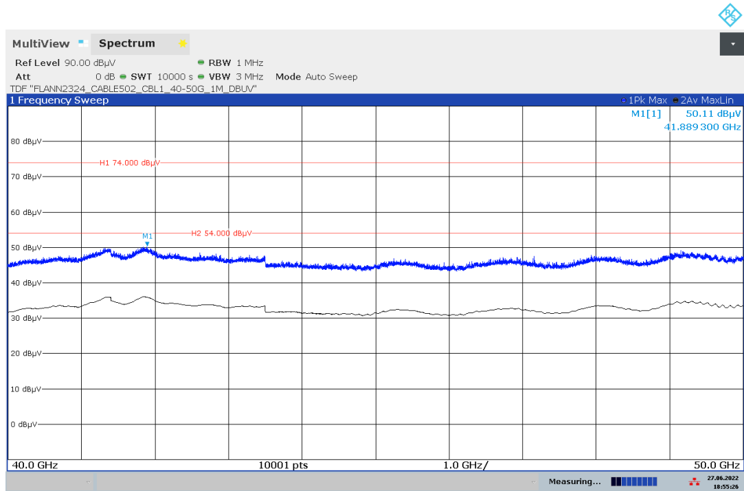
Plot 9: 40 GHz – 50 GHz, PEAK/RMS-measurement, f_{\text{low}}/f_{\text{mid}}/f_{\text{high}}
