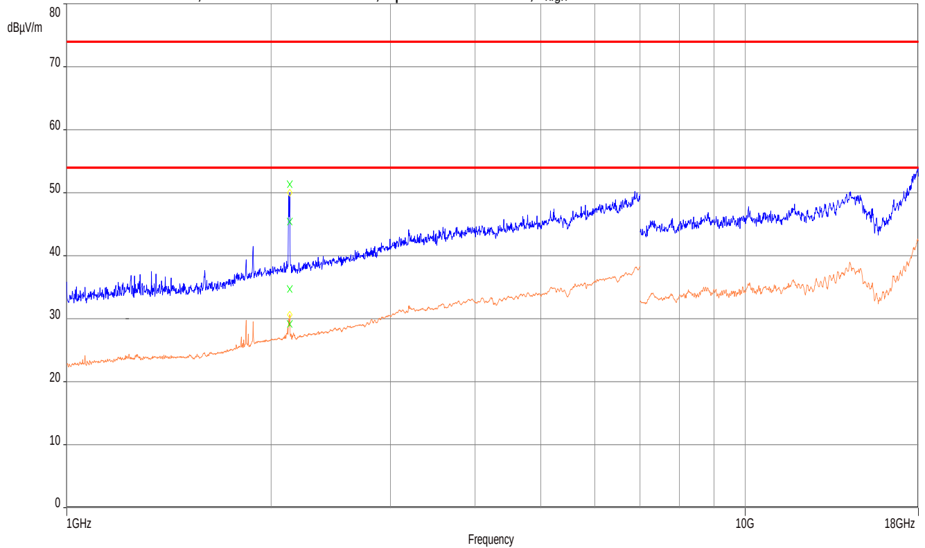
Plot 7: 1 GHz – 18 GHz, PEAK measurement, special test mode, f_{\text{high}}
