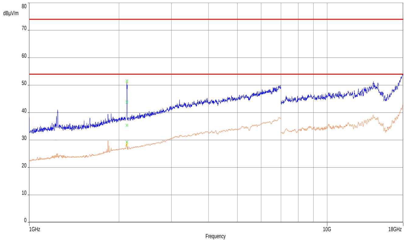
Plot 5: 1 GHz – 18 GHz, PEAK measurement, special test mode, f_{low}
