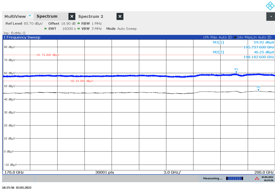
Plot 18: 170 GHz – 200 GHz, PEAK/RMS-measurement, f_{low}/f_{mid}/f_{high}
