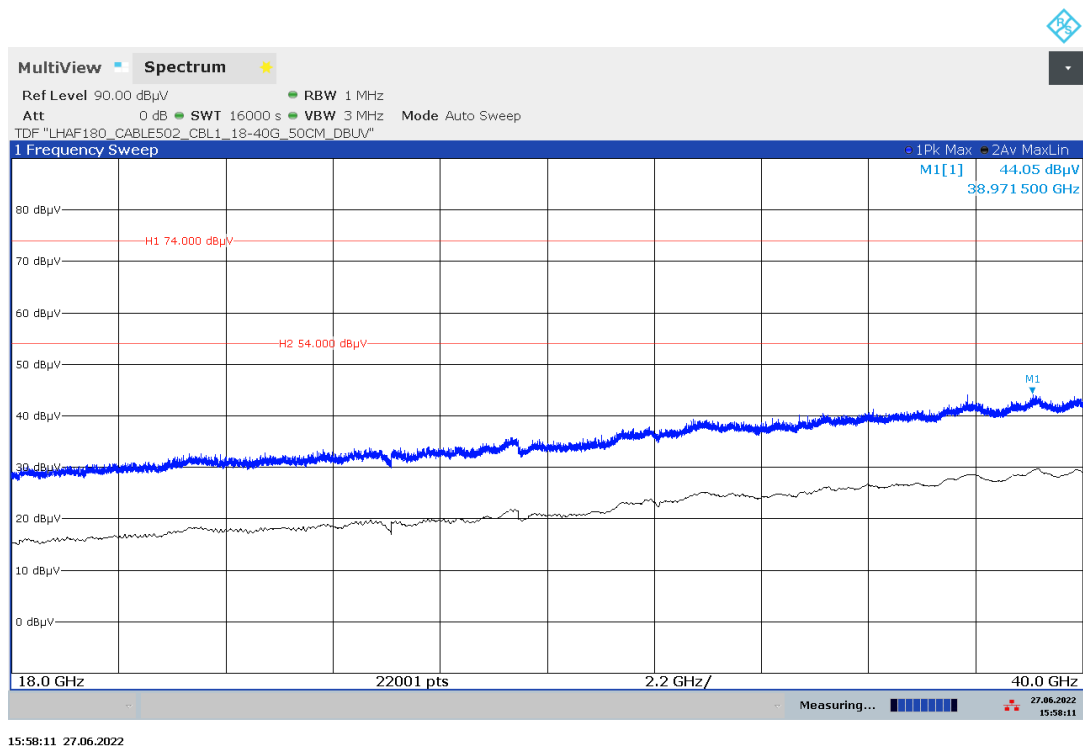
Plot 8: 18 GHz – 40 GHz, PEAK/RMS-measurement, f_{\text{low}}/f_{\text{mid}}/f_{\text{high}}
