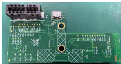
Figure 6: Adapter board - bottom side
