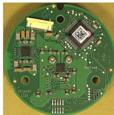
Figure 1: PMW board - primary side
