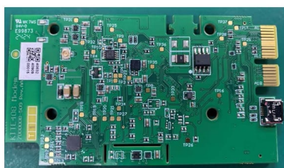
Figure 3: Modem board - top side
