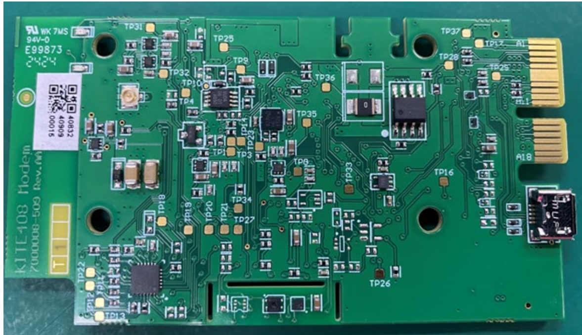
Figure 3: Modem board - top side
