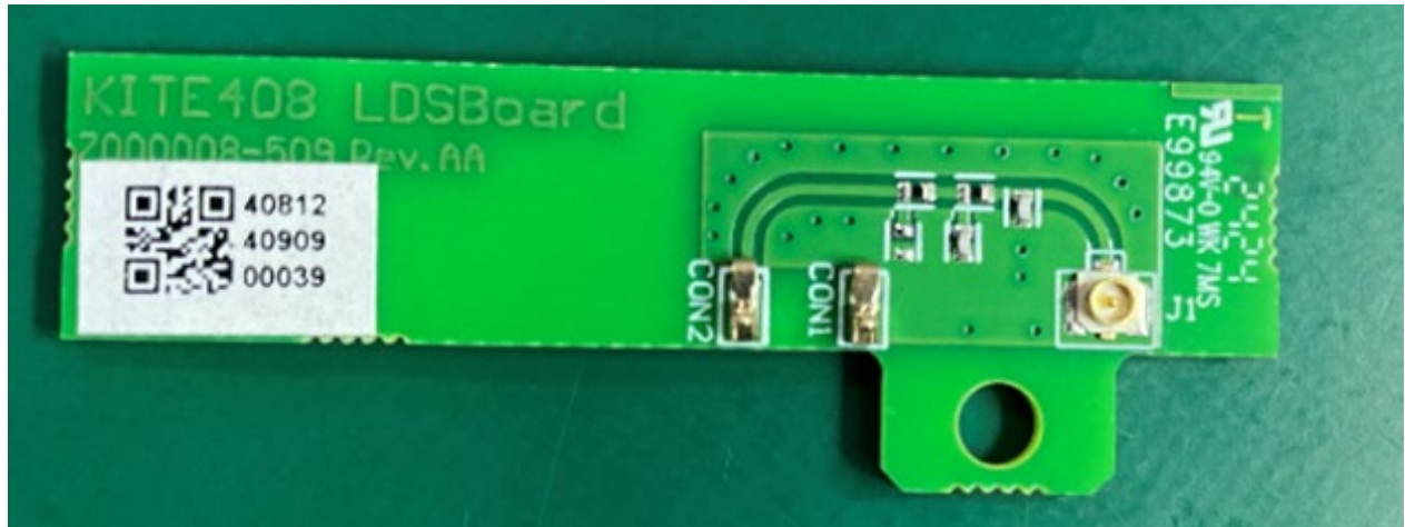
Figure 7: LDS board - top side
