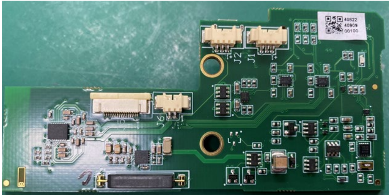
Figure 5: Adapter board - top side
