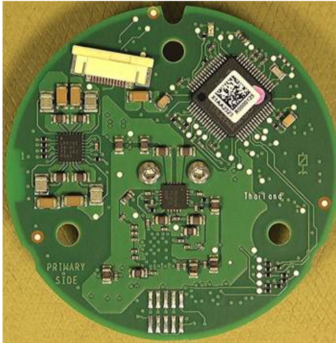
Figure 1: PMW board -primary side
