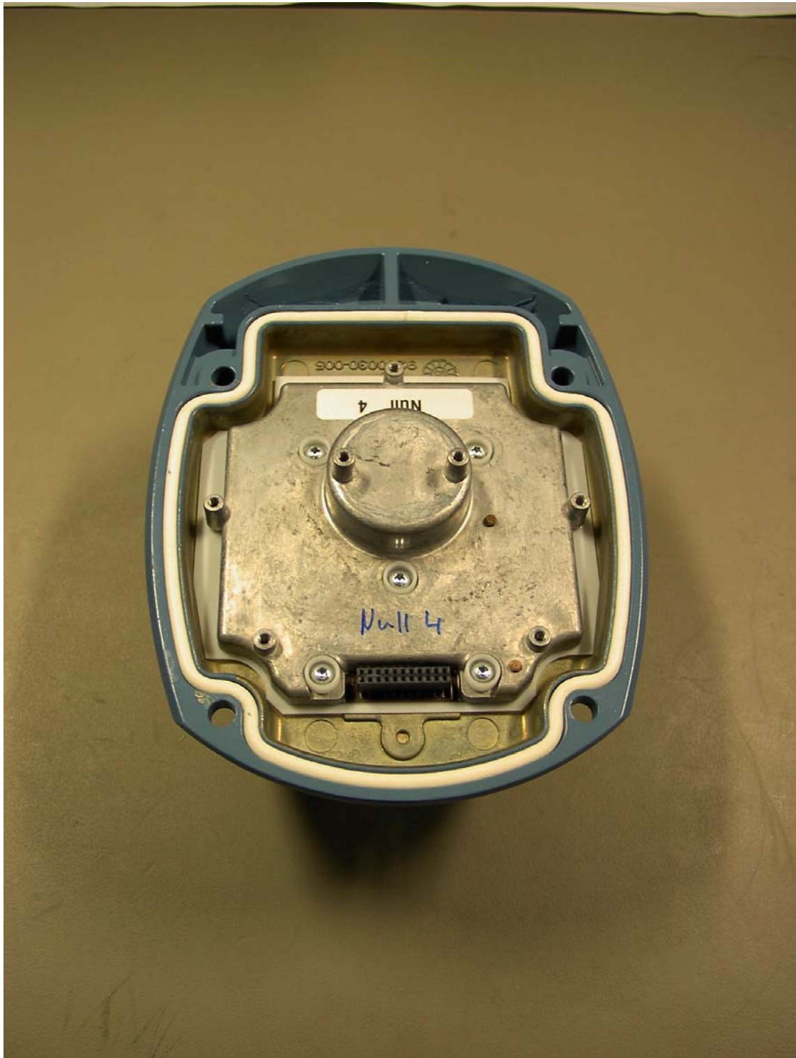
5. Assembly 3
