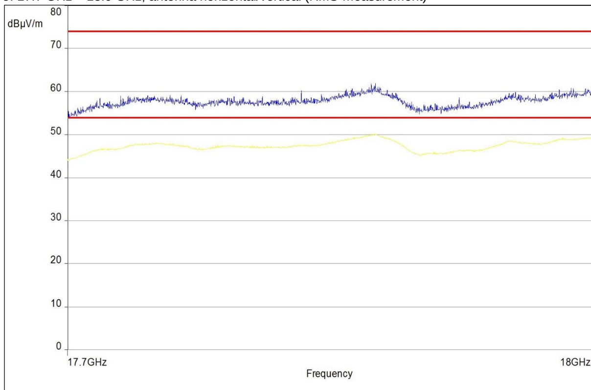
Plot 5: 17.7 GHz – 18.0 GHz, antenna horizontal/vertical (RMS-measurement)
