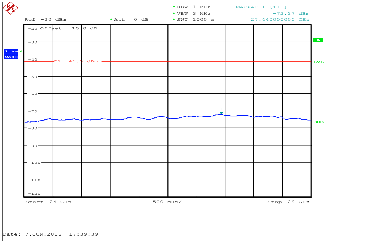
Plot 1: EIRP Emissions for TLPR devices, RMS detector, antenna horizontal/vertical
