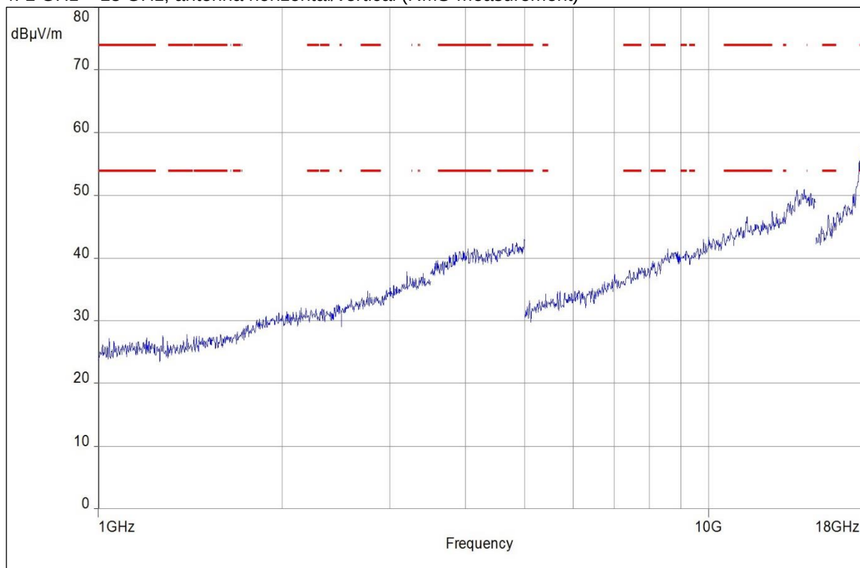
Plot 4: 1 GHz – 18 GHz, antenna horizontal/vertical (RMS-measurement)
