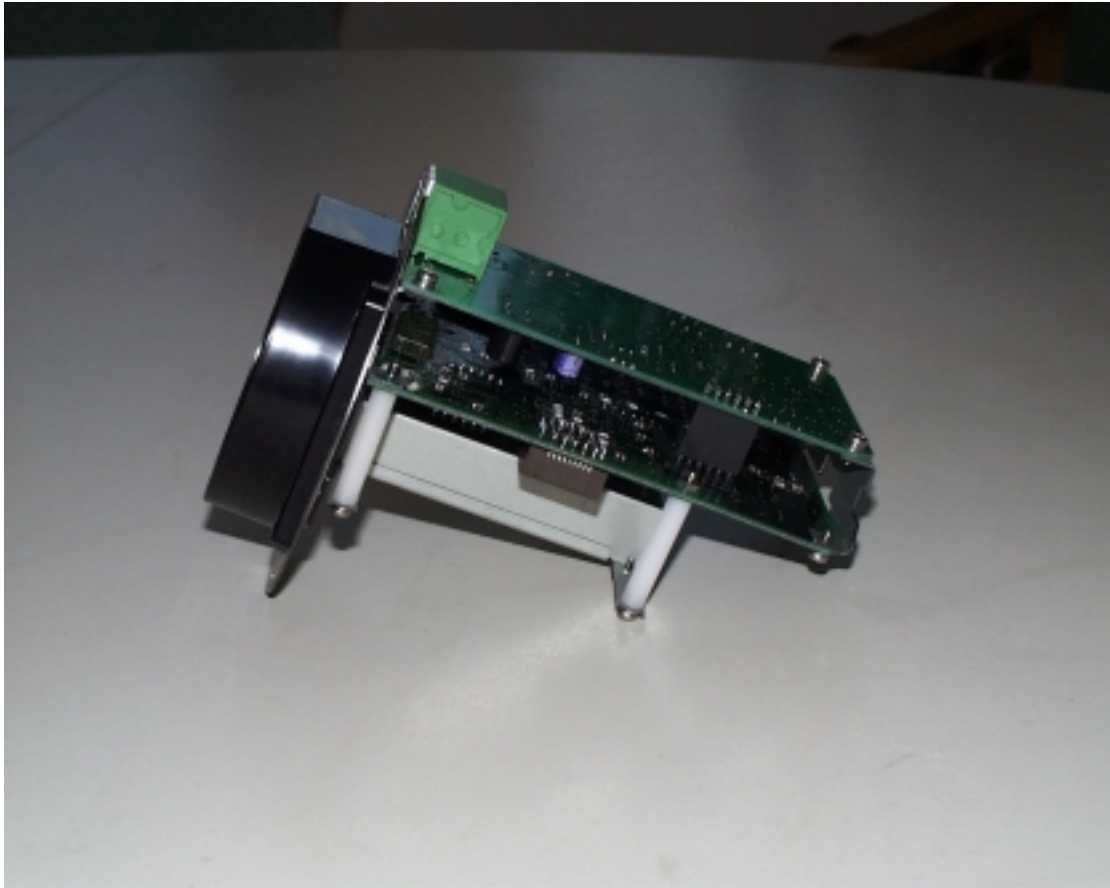
Chassis assembly top view
