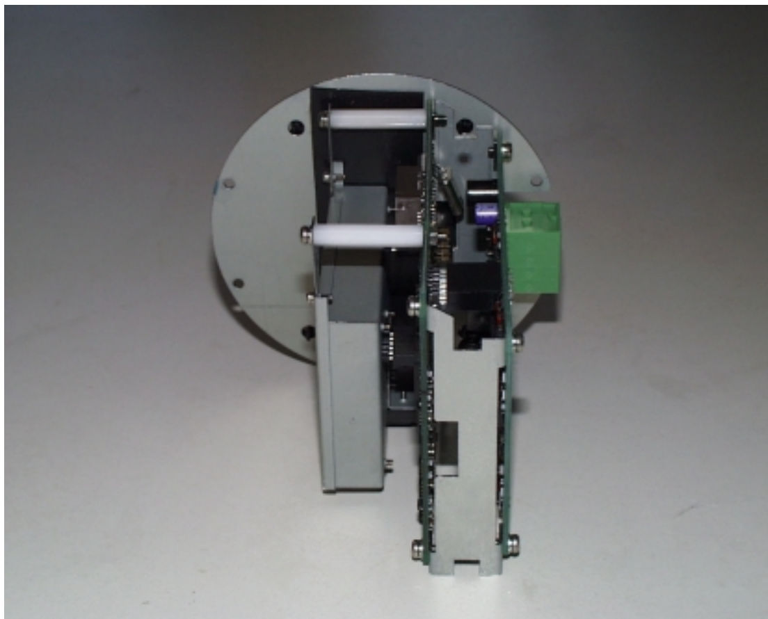
Chassi assembly back view
