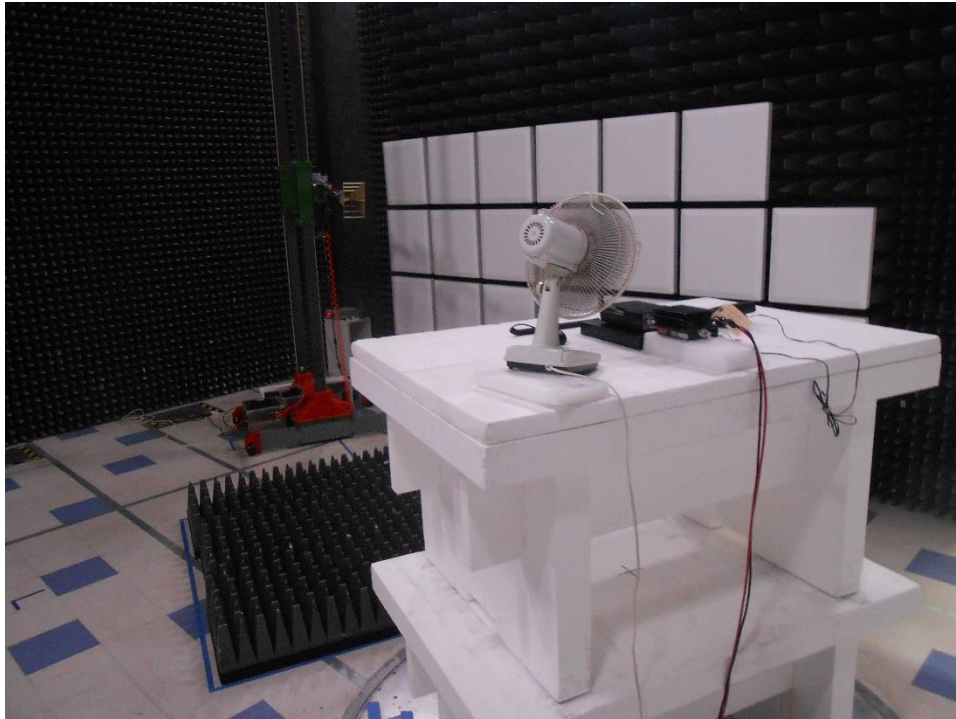
Radiated Emissions_1-5GHz (1)
