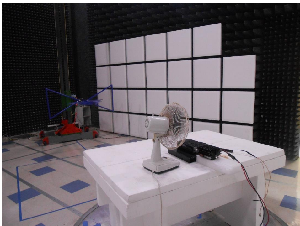
Radiated Emissions_30-1000MHz (2)
