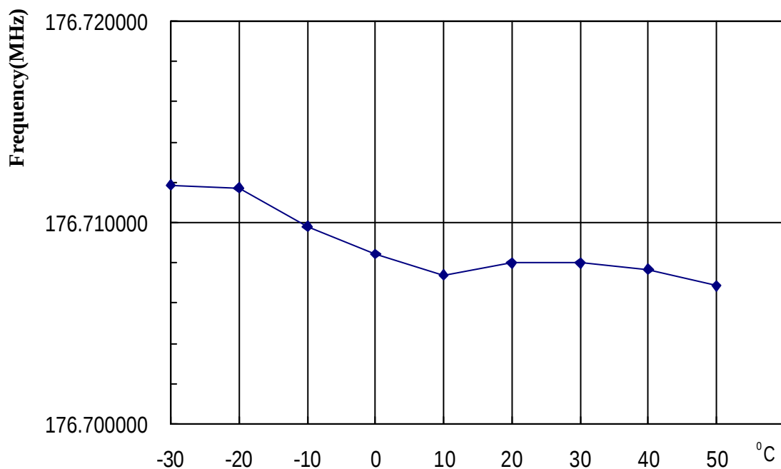
Temperatuer Variation Vs. Frequency Chart
