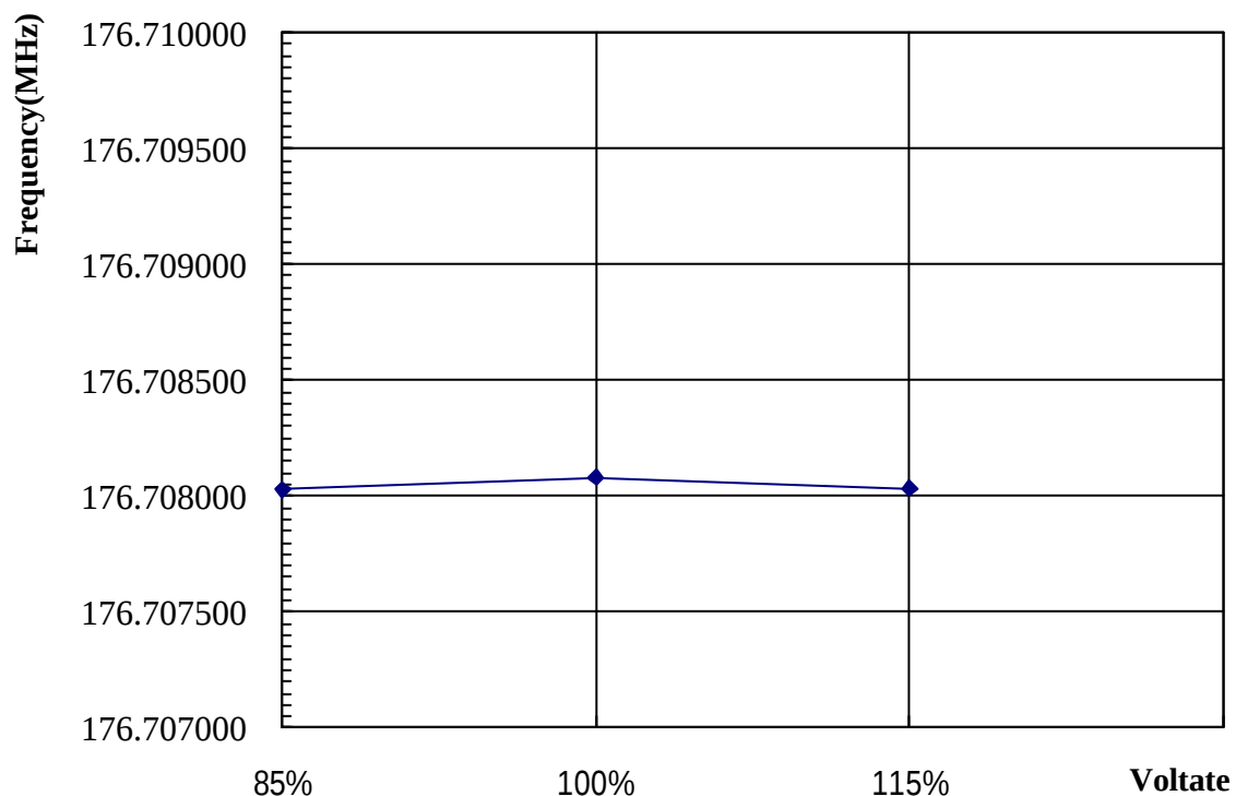
Voltage Variation Vs. Frequency Chart
