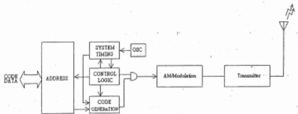
TX-1001-2T/4T BLOCK DIAGRAM
