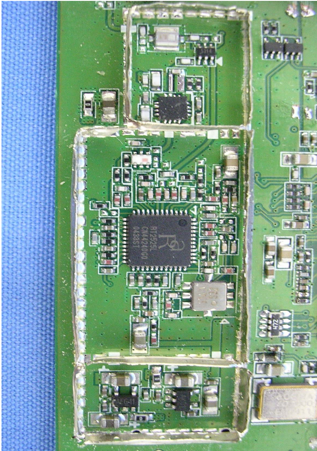
(11) EUT Photo
