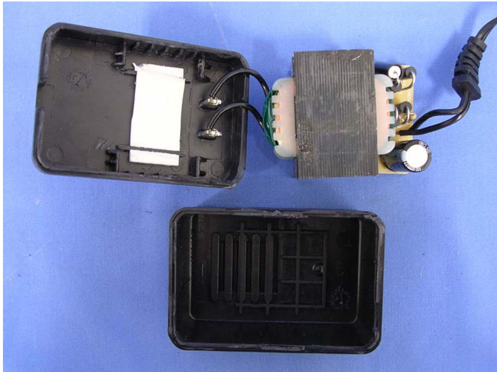
(13) EUT Photo(AD-071A5)
