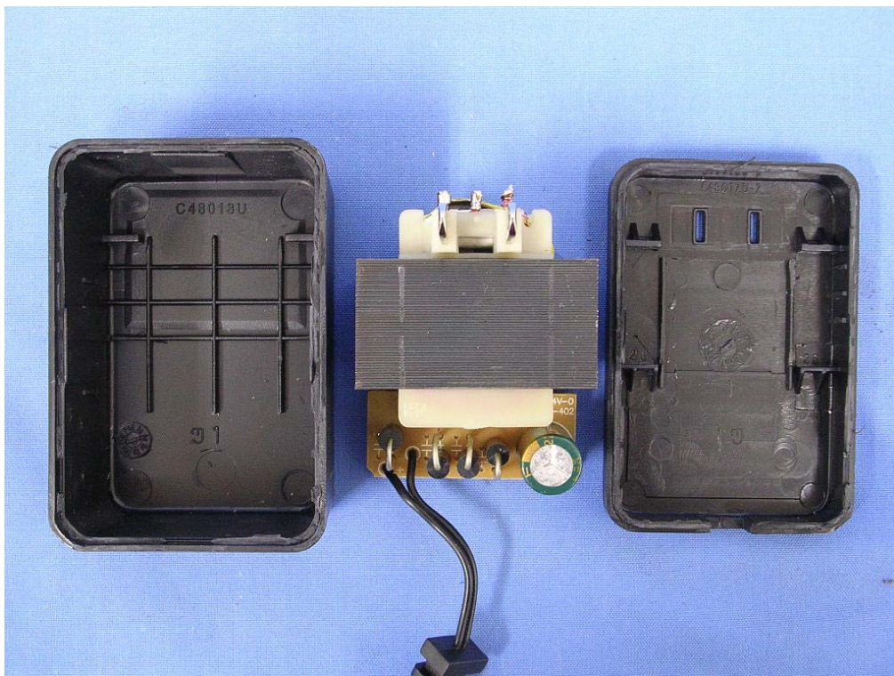
(16) EUT Photo(AM-0751500D)
