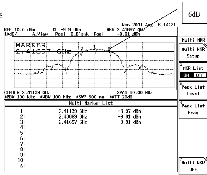
Figure Channel 1: 1Mbps
