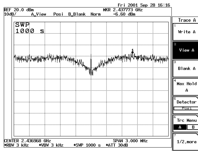
Figure Channel 6:1Mbps
