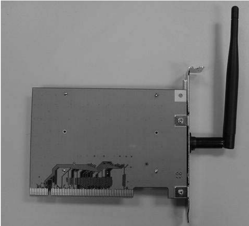
Back side of card showing the solder points for cover shield
