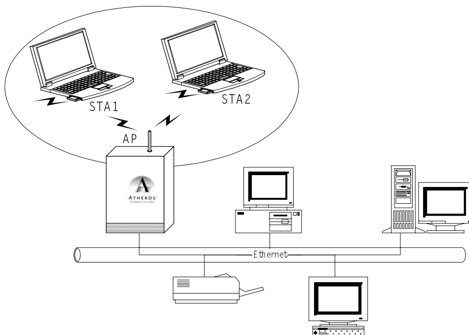
Figure 2-1. Infrastructure Mode
