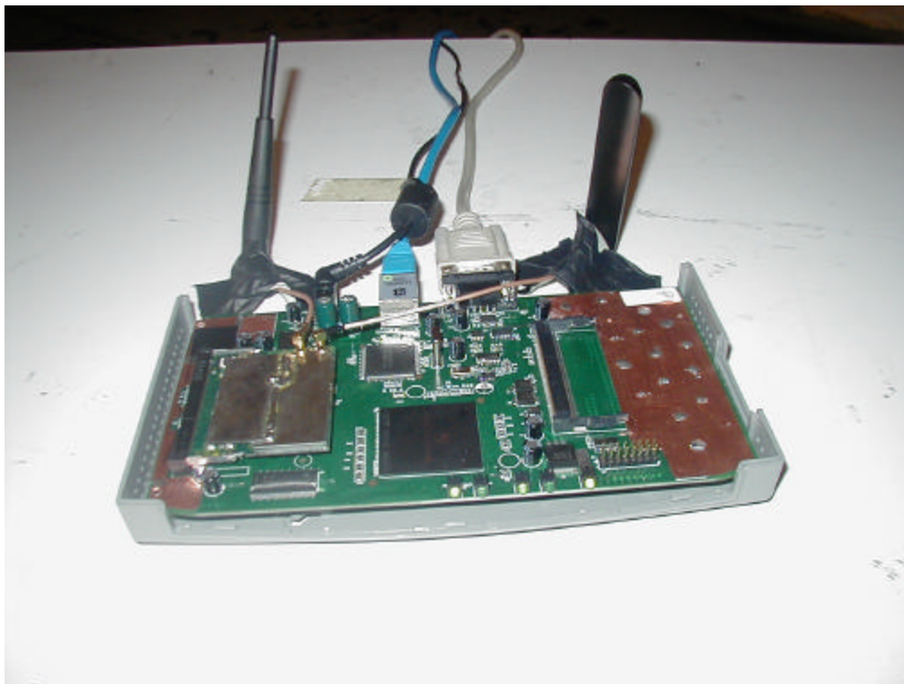
Radiated Emission with Atheros antennas
