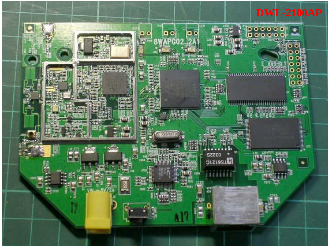
Photo 3: Interior photo of EUT
