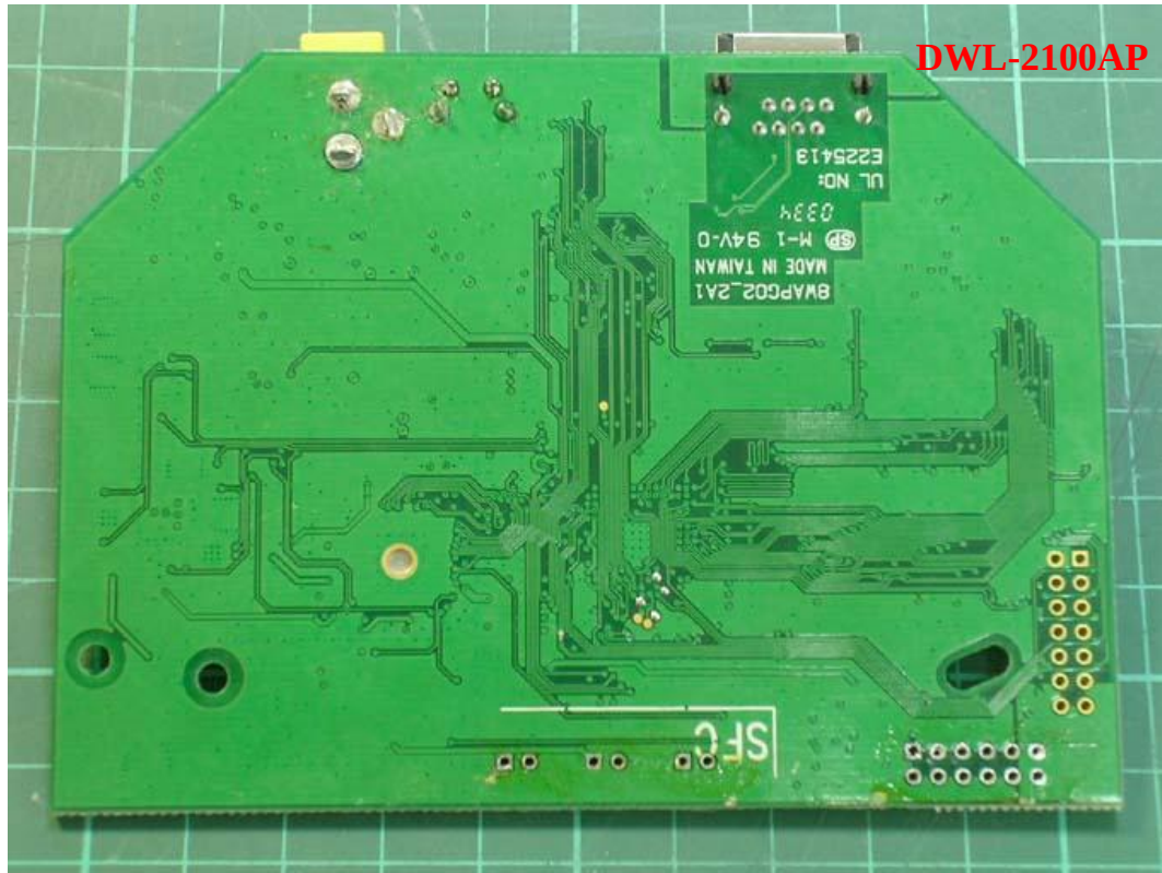
Photo 4: Interior photo of EUT
