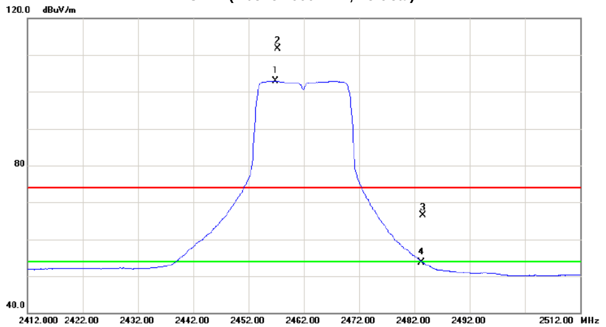
TX CH11 (Above 1000 MHz, Vertical)
