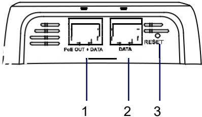
Figure 2: Bottom Connectors
