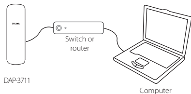
Figure 4: Indirect Connection
