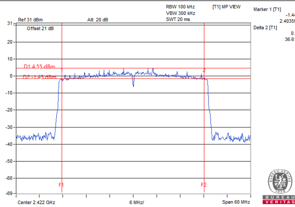
802.11ax (HE40) / Chain 1 : CH3
