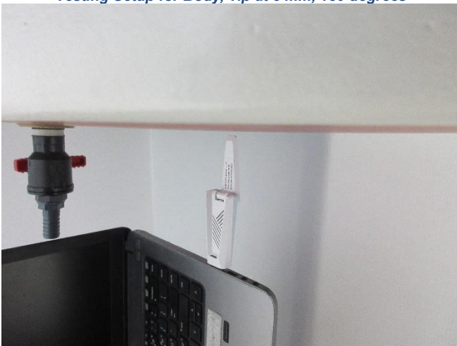
Testing Setup for Body, Tip at 5 mm, 180 degrees
