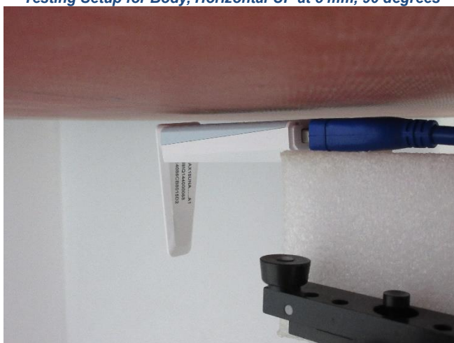
Testing Setup for Body, Horizontal-UP at 5 mm, 90 degrees
