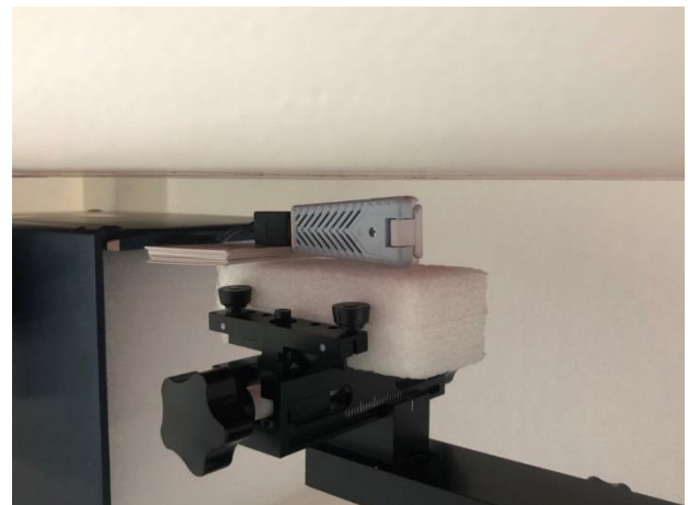
Testing Setup for Body, Vertical-Back at 5 mm, 0 degrees
