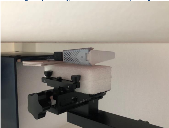
Testing Setup for Body, Vertical-Back at 5 mm, 90 degrees
