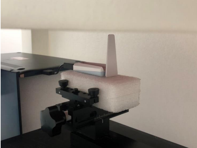
Testing Setup for Body, Horizontal-Down at 5 mm, 90 degrees
