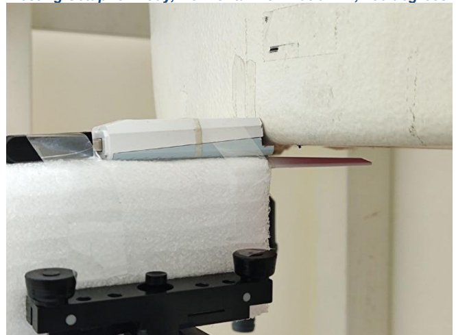
Testing Setup for Body, Horizontal-Down at 5 mm, 180 degrees
