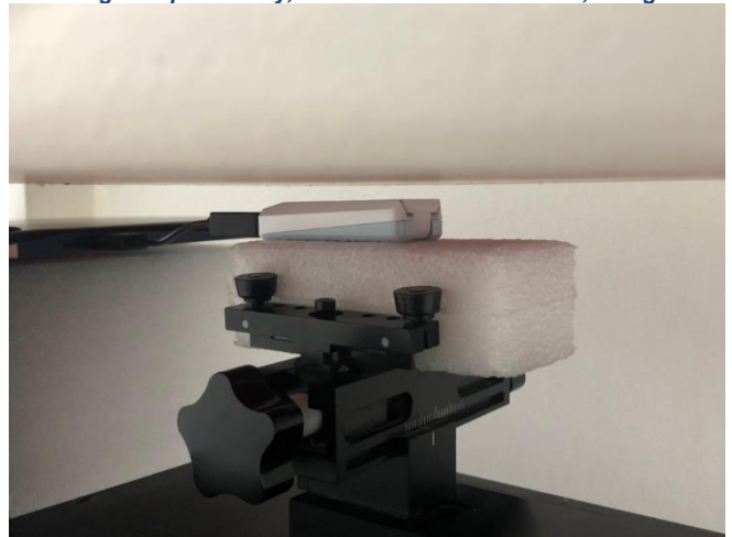
Testing Setup for Body, Horizontal-Down at 5 mm, 0 degrees
