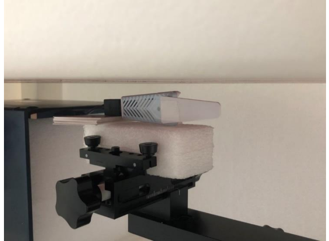
Testing Setup for Body, Vertical-Back at 5 mm, 180 degrees
