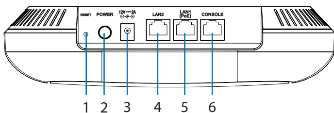
Figure 2: Rear Connectors
