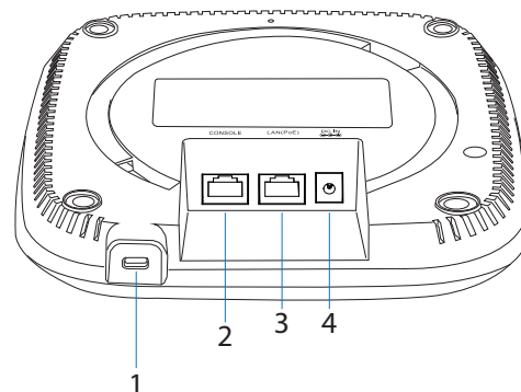
Figure 2: Rear Connectors
