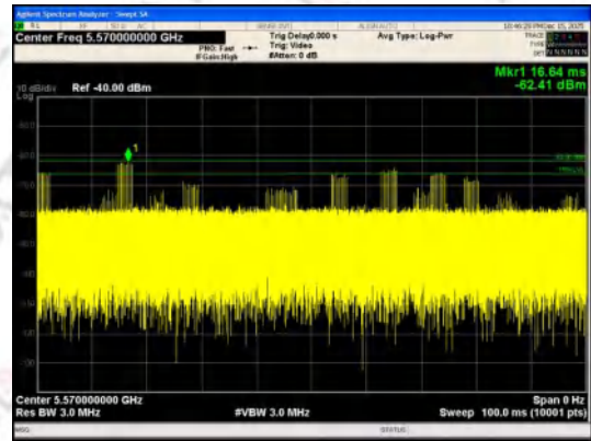
FCC radar test signal Type 6 5570MHz/160MHz
