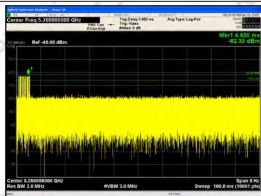
FCC radar test signal Type 2 5260MHz/20MHz
