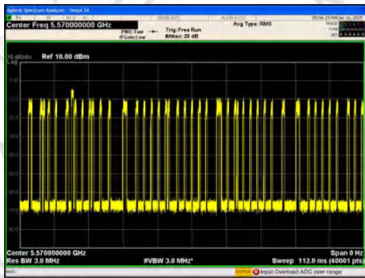
Data Traffic Plot(35.25%)
