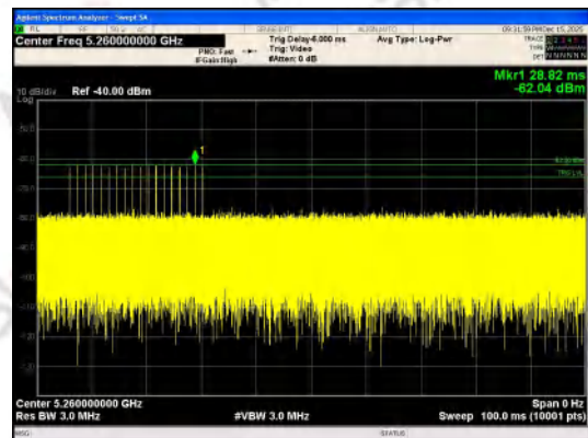
FCC radar test signal Type 0 5260MHz/20MHz
