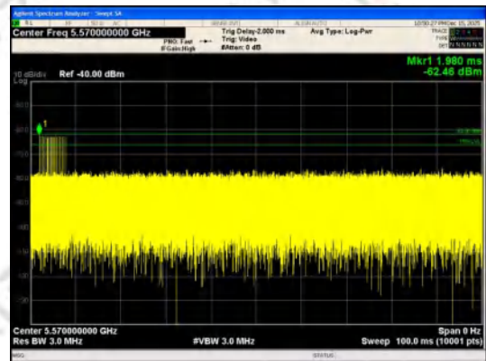
FCC radar test signal Type 3 5570MHz/160MHz
