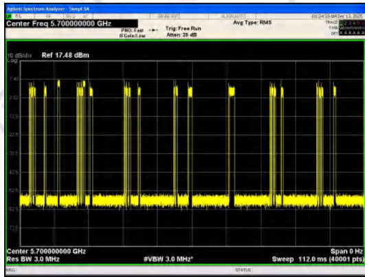
Data Traffic Plot(33.25%)
