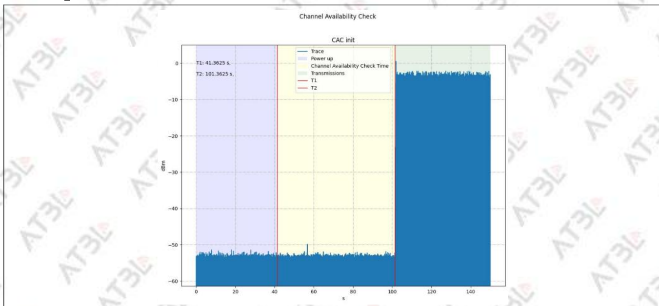
EUT Power up and Initial Channel Availability Check Time
