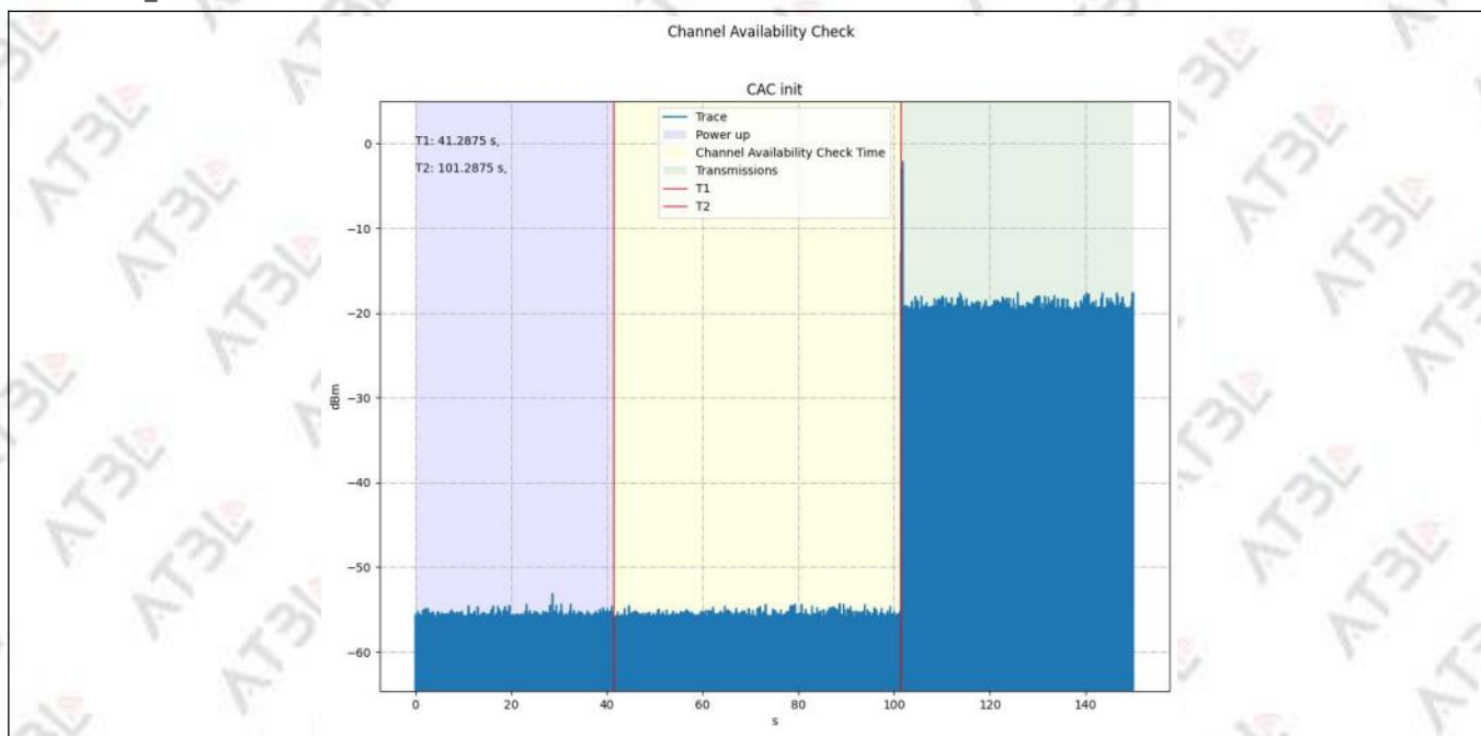
EUT Power up and Initial Channel Availability Check Time
