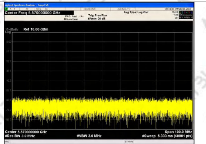
Noise Floor(No transmission)
