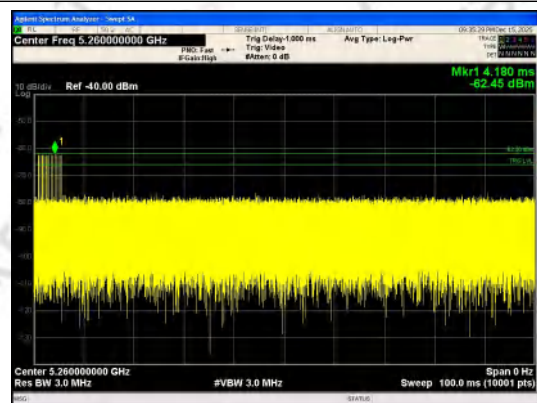
FCC radar test signal Type 4 5260MHz/20MHz
