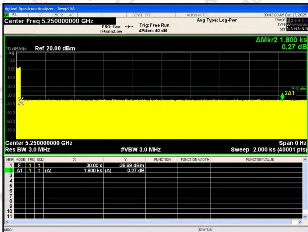
Non-Occupancy Period IEEE 802.11be_160 Channel 50
