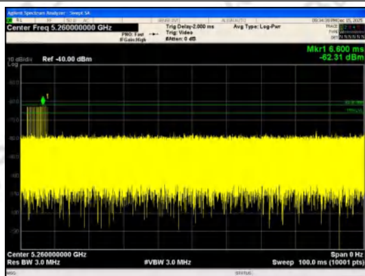
FCC radar test signal Type 3 5260MHz/20MHz
