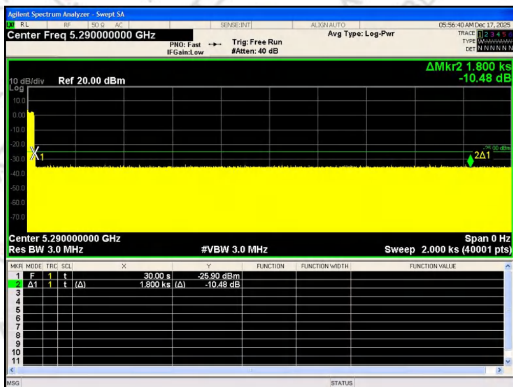
Non-Occupancy Period IEEE 802.11be_80 Channel 58
