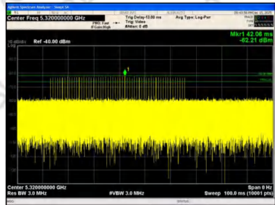
FCC radar test signal Type 1 5320MHz/20MHz
