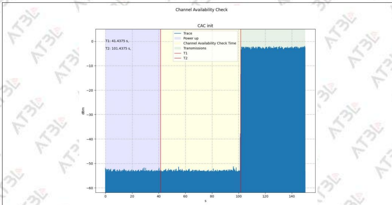
EUT Power up and Initial Channel Availability Check Time
