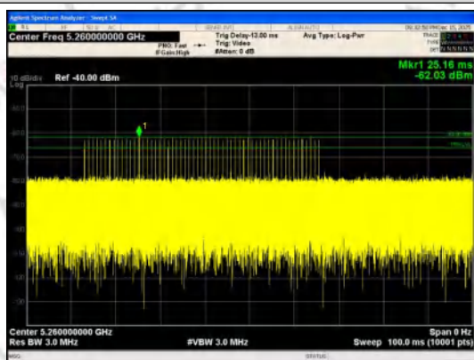
FCC radar test signal Type 1 5260MHz/20MHz
