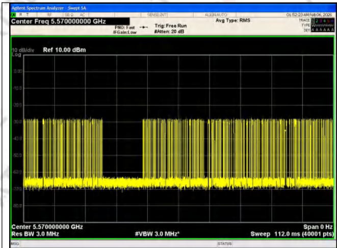
Data Traffic Plot(22.29%)
