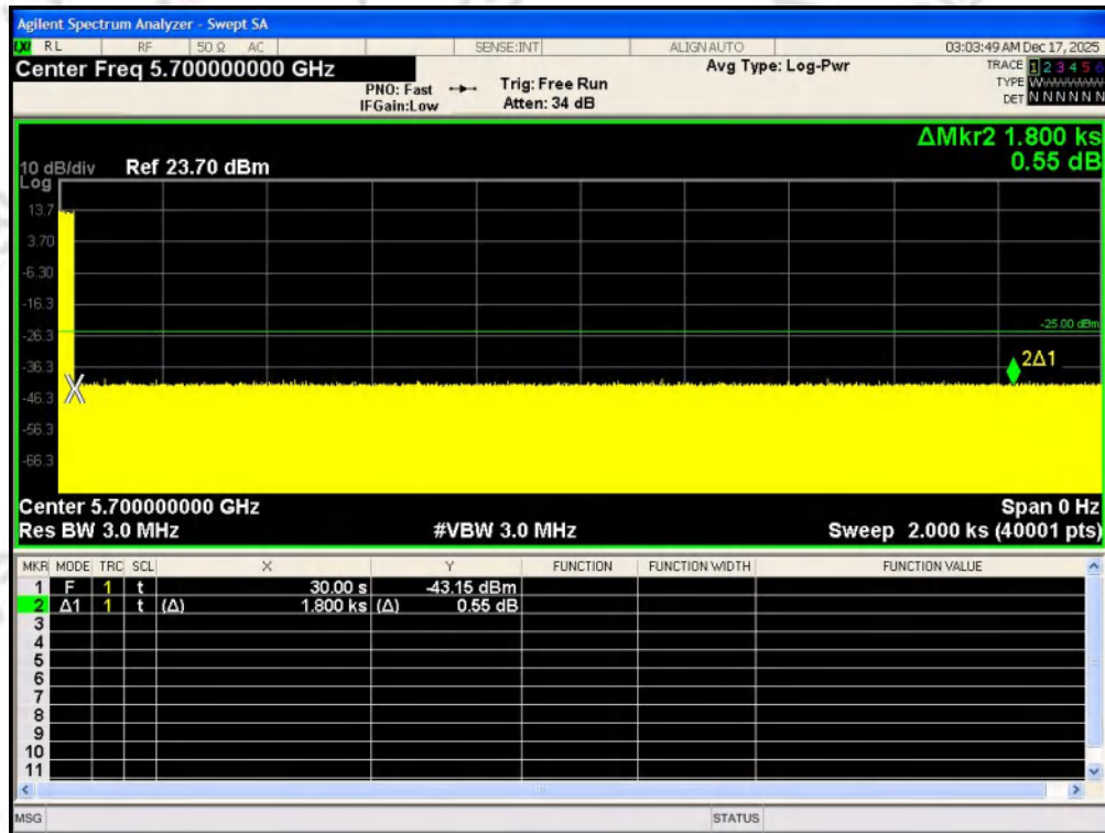
Non-Occupancy Period IEEE 802.11be_20 Channel 140
