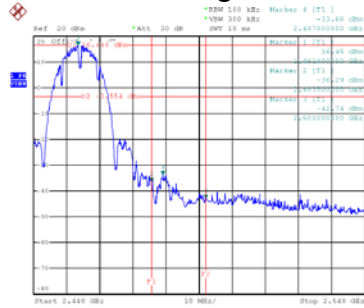
Bandedge-CH11
