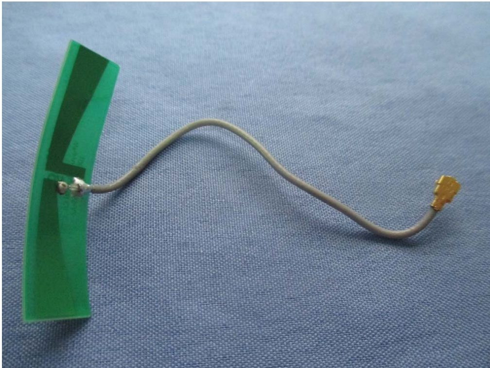
(29) EUT Photo (Antenna (2.4G))
