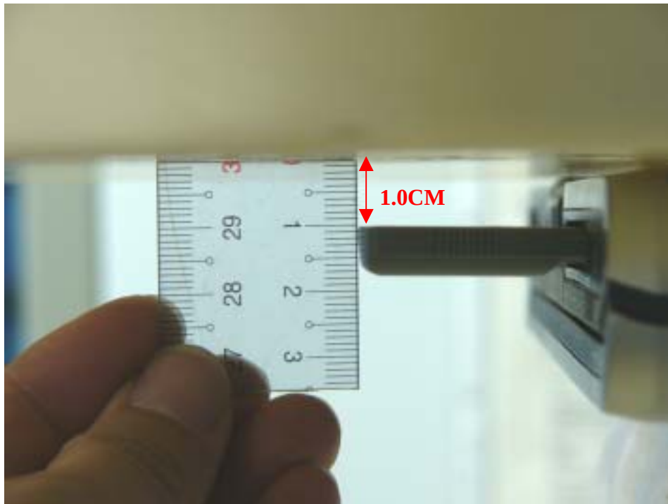
Fig.7 Photograph of the Bottom of the Pc is paralleled and at a distance of 0.0 cm from the base of the phantom, but 1.0 cm Spacing between EUT & Planar Phantom
