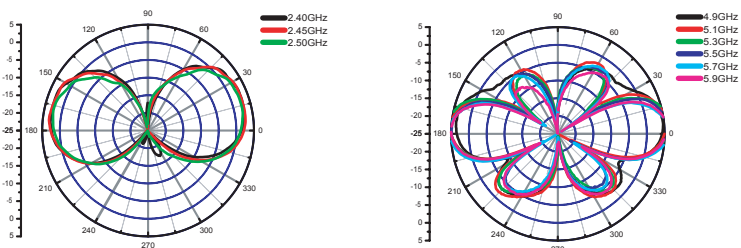
V-plane Co-polarization Pattern
