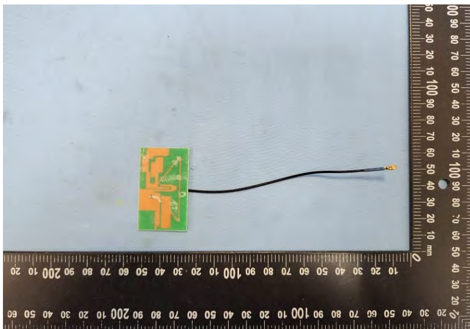
EUT Photo (32)
