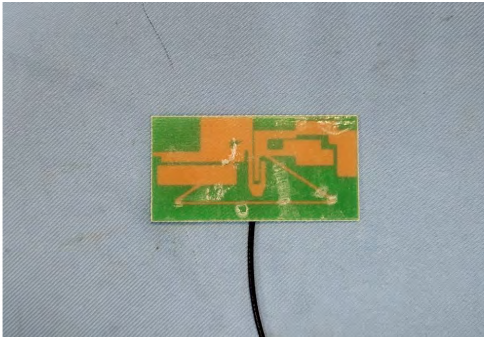
EUT Photo (34)
