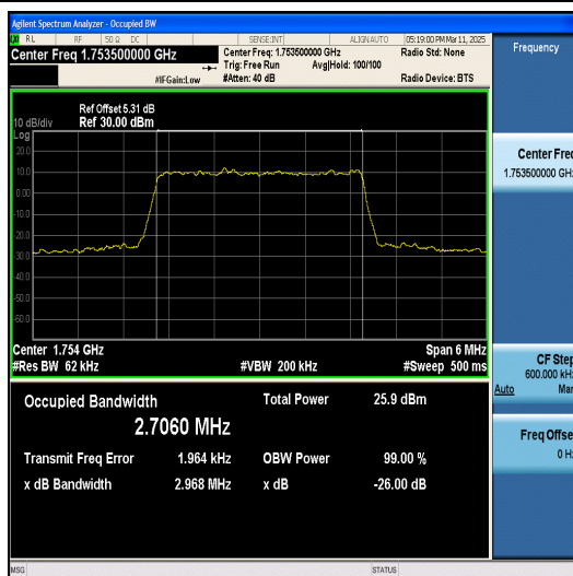
Band4-3MHz-QPSK-20385-15RB#0-PASS
