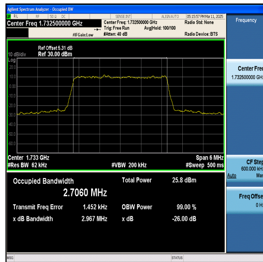
Band4-3MHz-64QAM-20175-15RB#0-PASS
