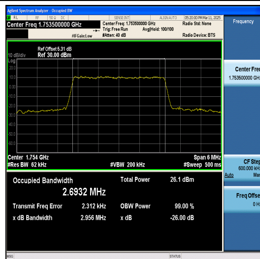
Band4-3MHz-16QAM-20385-15RB#0-PASS
