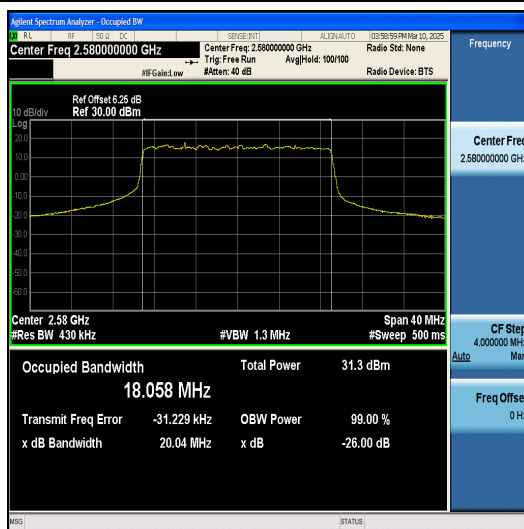
Band38-20MHz-QPSK-37850-100RB#0-PASS
