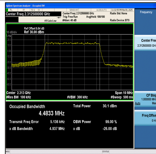
Band40(2305-2320)-5MHz-QPSK-38775-25RB#0- PASS
