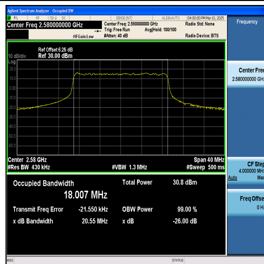
Band38-20MHz-16QAM-37850-100RB#0-PASS
