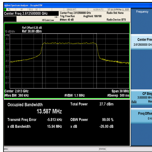
Band38-15MHz-64QAM-38175-75RB#0-PASS
