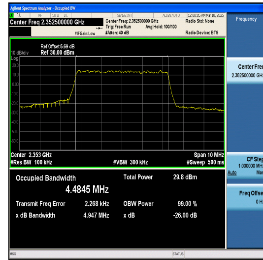
Band40(2345-2360)-5MHz-QPSK-39175-25RB#0- PASS
