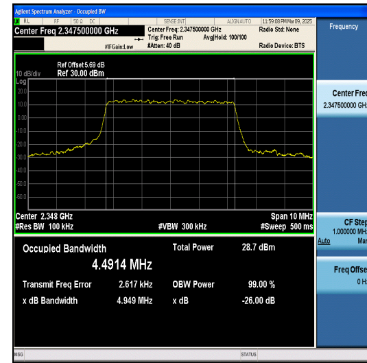
Band40(2345-2360)-5MHz-64QAM-39125-25RB# 0-PASS
