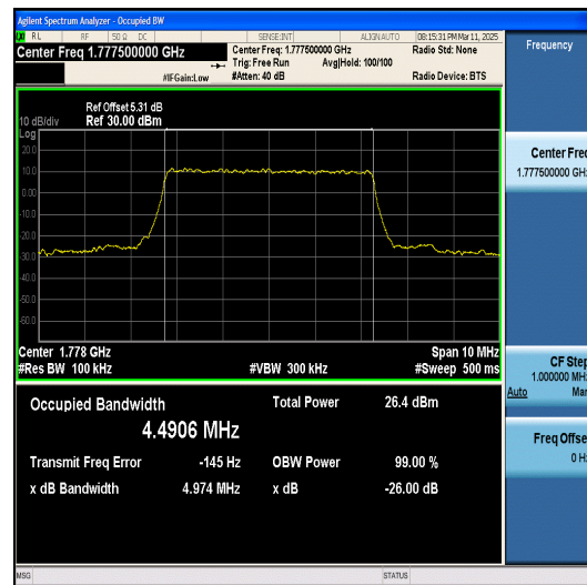
Band66-5MHz-64QAM-132647-25RB#0-PASS
