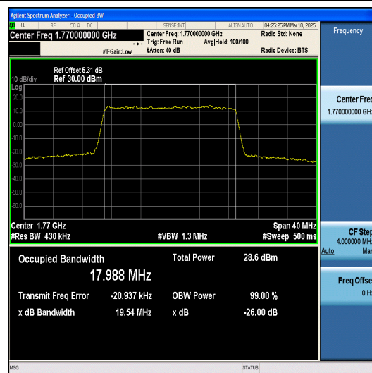
Band66-20MHz-16QAM-132572-100RB#0-PASS
