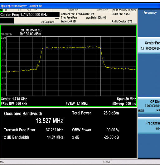
Band66-15MHz-64QAM-132047-75RB#0-PASS
