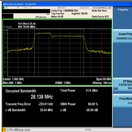
CA_2C-10MHz+20MHz-16QAM-18655+18799- 50RB#0+100RB#0-PASS
