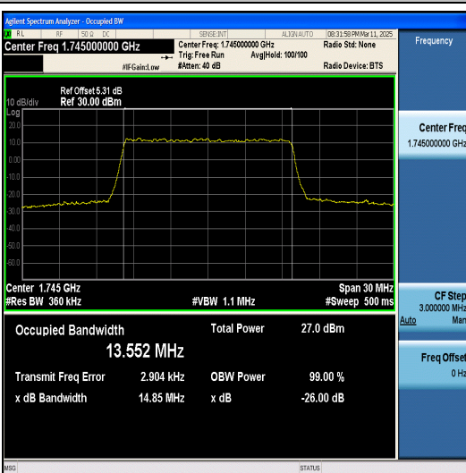
Band66-15MHz-QPSK-132322-75RB#0-PASS
