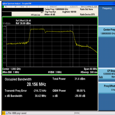
CA_2C-10MHz+20MHz-16QAM-18956+19100- 50RB#0+100RB#0-PASS
