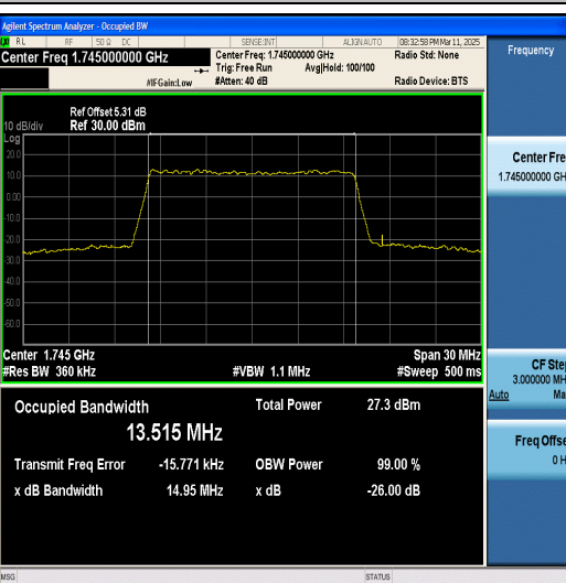
Band66-15MHz-16QAM-132322-75RB#0-PASS
