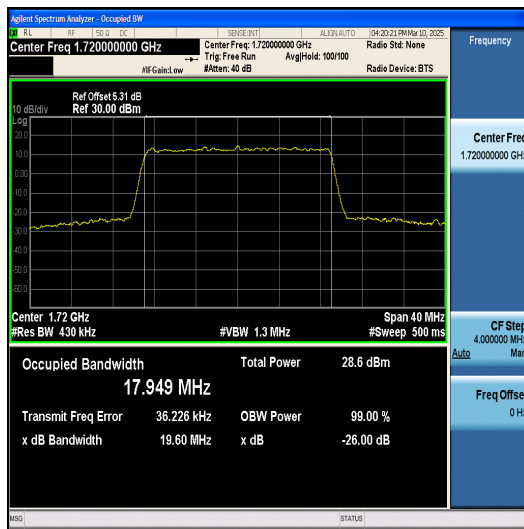
Band66-20MHz-16QAM-132322-100RB#0-PASS
