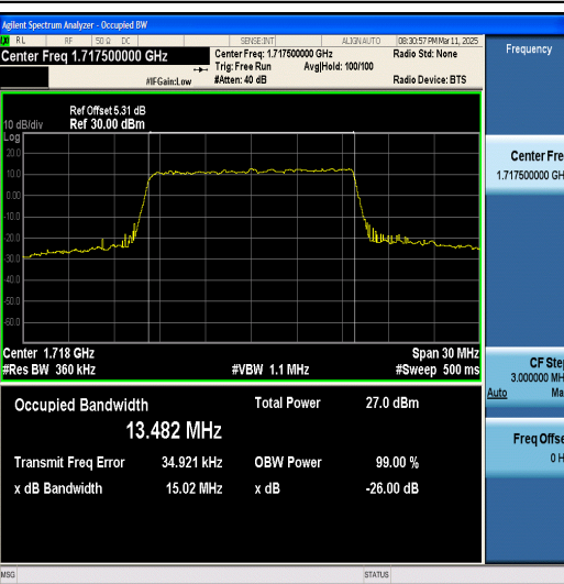
Band66-15MHz-16QAM-132322-75RB#0-PASS
