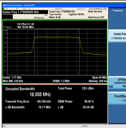
Band66-20MHz-QPSK-132572-100RB#0-PASS
