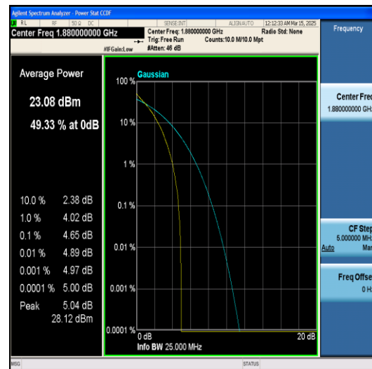
Band2-1.4MHz-64QAM-18900-1RB#0-PASS
