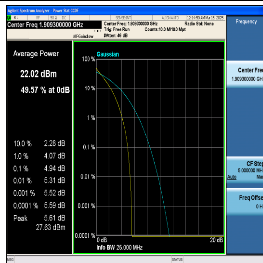
Band2-1.4MHz-QPSK-19193-6RB#0-PASS
