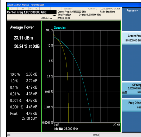
Band2-3MHz-64QAM-18615-1RB#0-PASS
