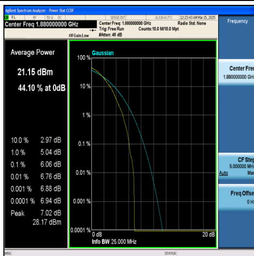
Band2-3MHz-64QAM-18900-1RB#0-PASS
