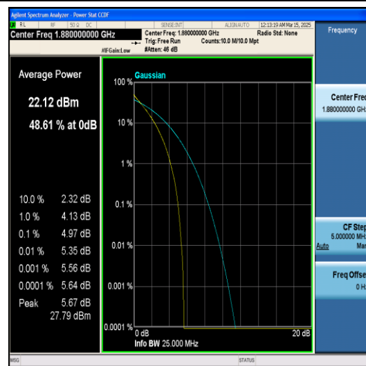
Band2-1.4MHz-QPSK-18900-6RB#0-PASS
