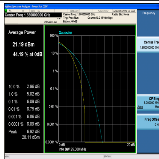
Band2-1.4MHz-64QAM-18900-1RB#0-PASS
