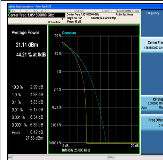
Band2-3MHz-64QAM-18615-1RB#0-PASS
