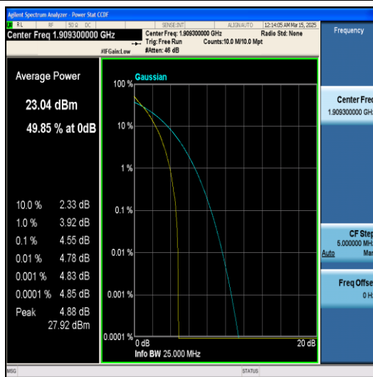
Band2-1.4MHz-64QAM-19193-1RB#0-PASS
