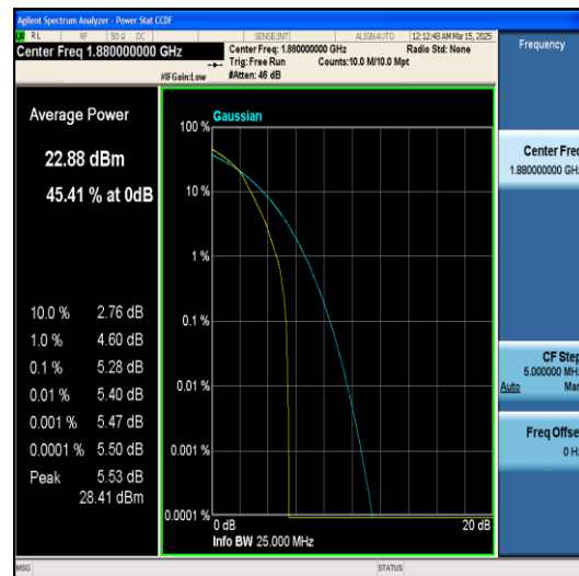
Band2-1.4MHz-QPSK-18900-6RB#0-PASS
