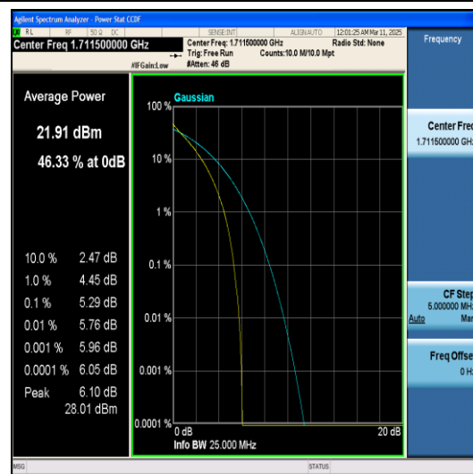
Band66-3MHz-QPSK-131987-15RB#0-PASS
