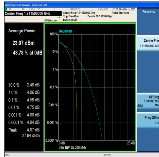
Band66-3MHz-64QAM-131987-1RB#0-PASS
