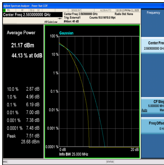
Band41-15MHz-QPSK-41515-1RB#0-PASS
