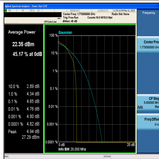
Band66-1.4MHz-QPSK-132665-6RB#0-PASS
