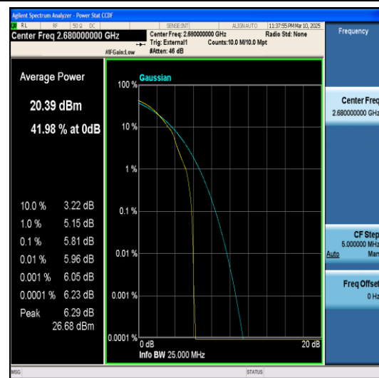
Band41-20MHz-64QAM-41490-1RB#0-PASS
