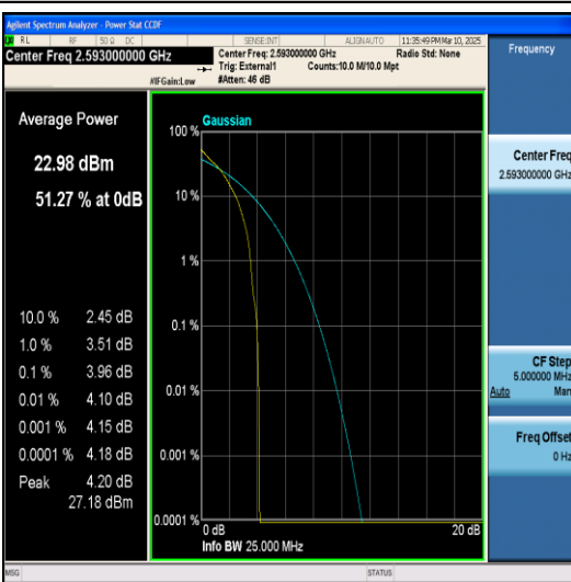
Band41-20MHz-64QAM-40620-1RB#0-PASS
