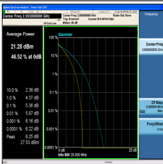
Band41-20MHz-QPSK-40620-100RB#0-PASS
