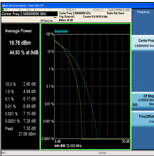
Band41-20MHz-QPSK-40620-1RB#0-PASS
