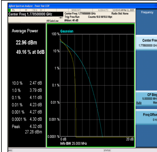
Band66-3MHz-64QAM-132657-1RB#0-PASS
