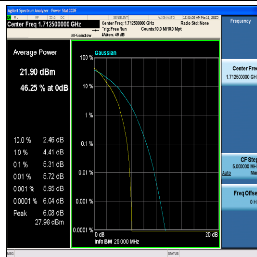
Band66-5MHz-QPSK-131997-25RB#0-PASS
