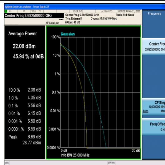
Band41-15MHz-QPSK-41515-75RB#0-PASS
