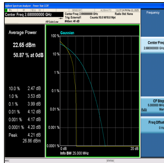
Band41-20MHz-64QAM-41490-1RB#0-PASS
