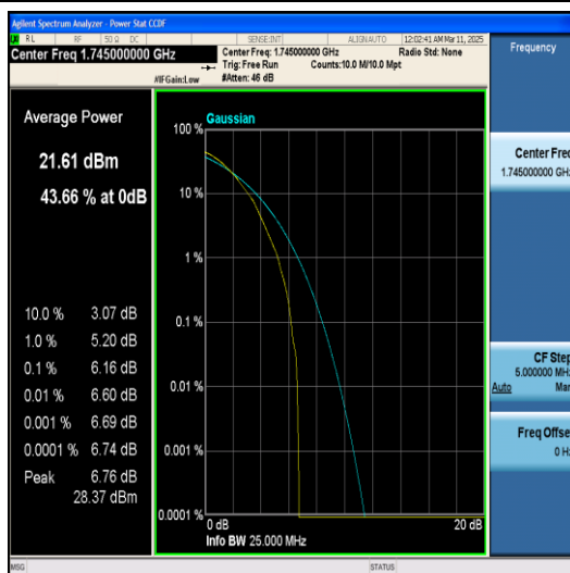
Band66-3MHz-64QAM-132322-1RB#0-PASS
