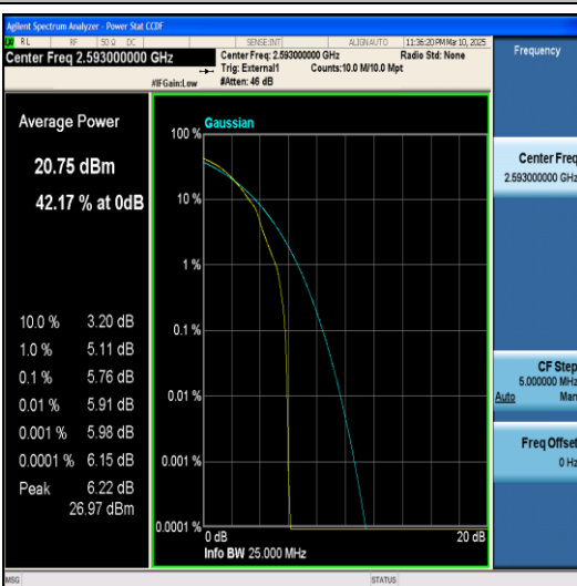
Band41-20MHz-64QAM-40620-1RB#0-PASS
