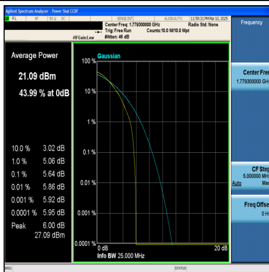
Band66-1.4MHz-64QAM-132665-1RB#0-PASS
