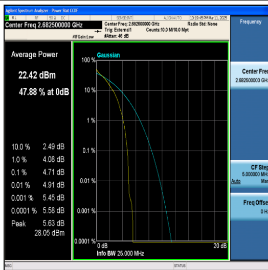
Band41-15MHz-64QAM-41515-1RB#0-PASS
