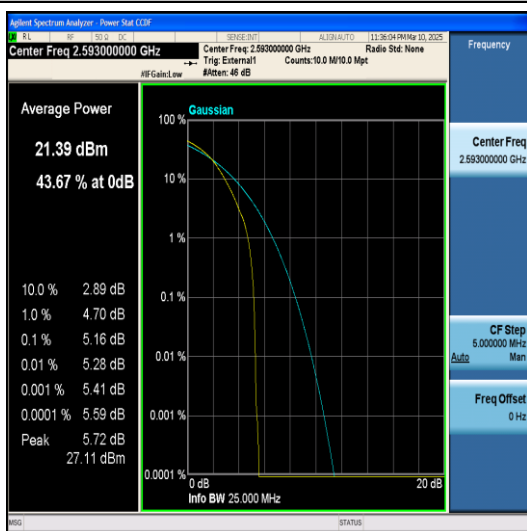
Band41-20MHz-QPSK-40620-100RB#0-PASS
