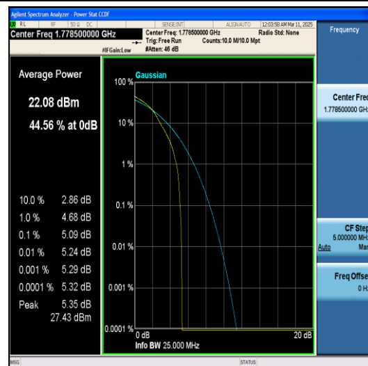
Band66-3MHz-QPSK-132657-15RB#0-PASS
