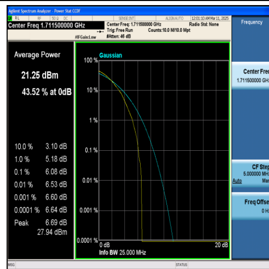
Band66-3MHz-64QAM-131987-1RB#0-PASS
