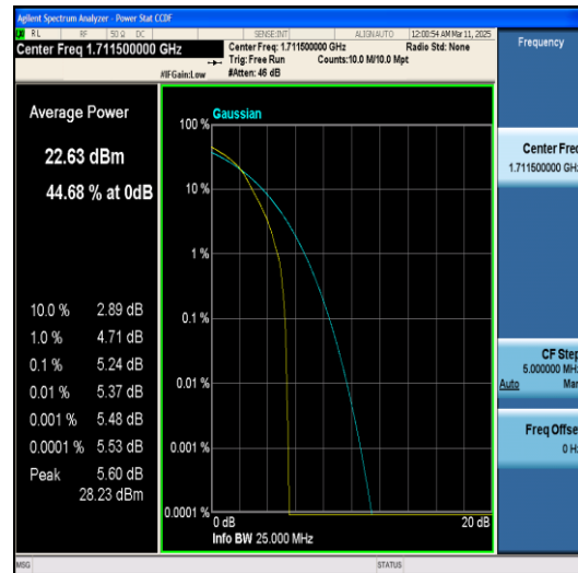
Band66-3MHz-QPSK-131987-15RB#0-PASS
