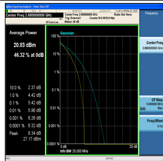
Band41-20MHz-QPSK-41490-100RB#0-PASS
