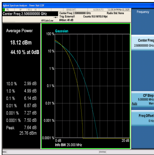
Band41-20MHz-16QAM-40620-1RB#0-PASS
