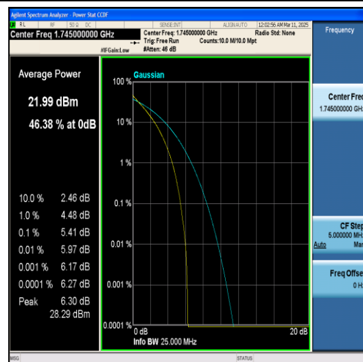
Band66-3MHz-QPSK-132322-15RB#0-PASS
