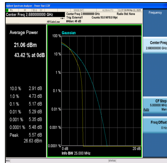
Band41-20MHz-QPSK-41490-100RB#0-PASS
