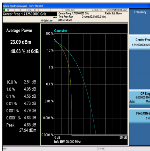
Band66-5MHz-64QAM-131997-1RB#0-PASS
