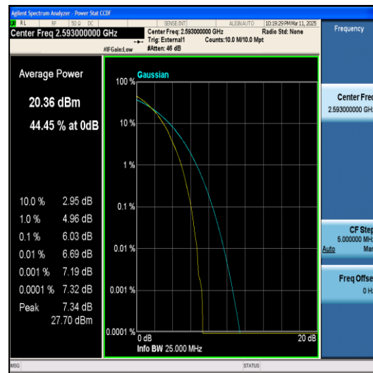
Band41-15MHz-16QAM-41515-1RB#0-PASS
