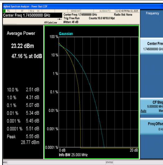
Band66-20MHz-64QAM-132322-1RB#0-PASS
