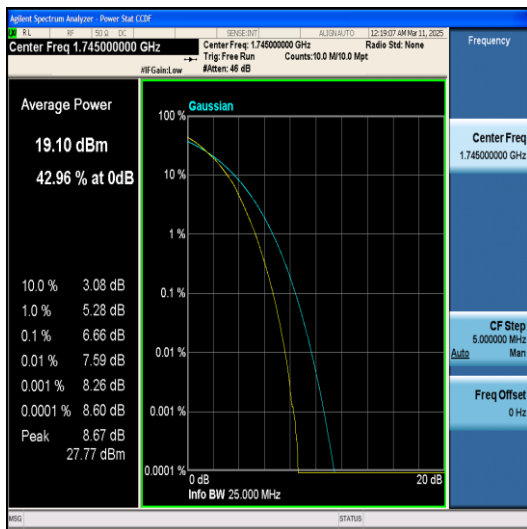
Band66-15MHz-16QAM-132597-1RB#0-PASS
