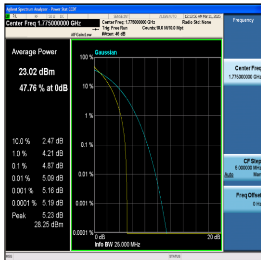
Band66-10MHz-64QAM-132622-1RB#0-PASS
