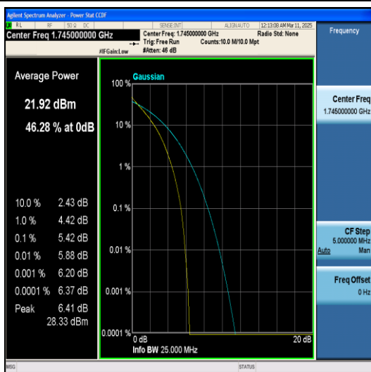
Band66-10MHz-QPSK-132322-50RB#0-PASS
