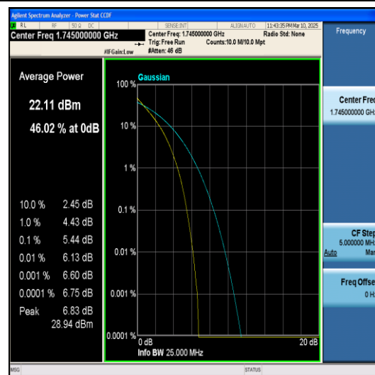
Band66-20MHz-QPSK-132322-100RB#0-PASS
