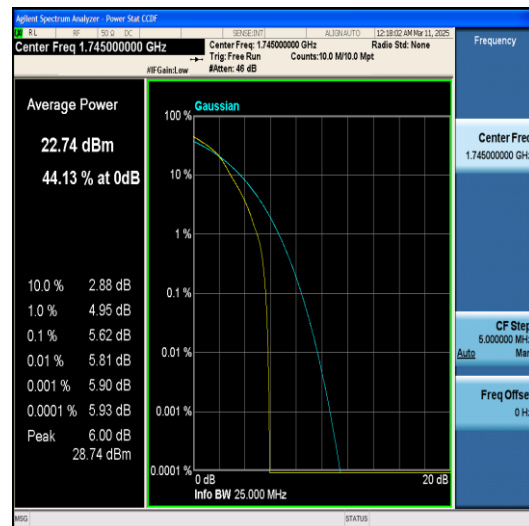
Band66-15MHz-QPSK-132322-75RB#0-PASS
