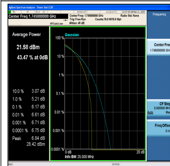
Band66-5MHz-64QAM-132322-1RB#0-PASS
