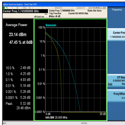
Band66-15MHz-64QAM-132322-1RB#0-PASS
