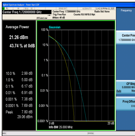
Band66-20MHz-QPSK-132322-1RB#0-PASS
