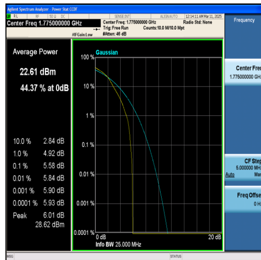
Band66-10MHz-QPSK-132622-50RB#0-PASS
