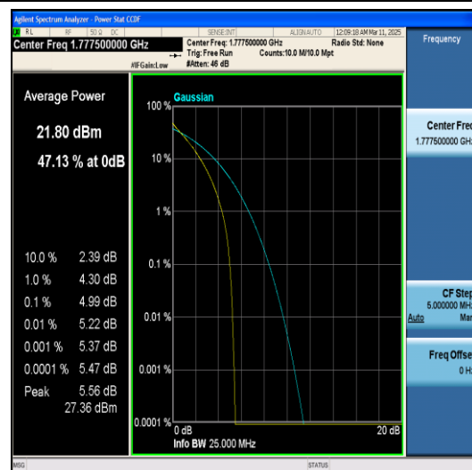
Band66-5MHz-QPSK-132647-25RB#0-PASS
