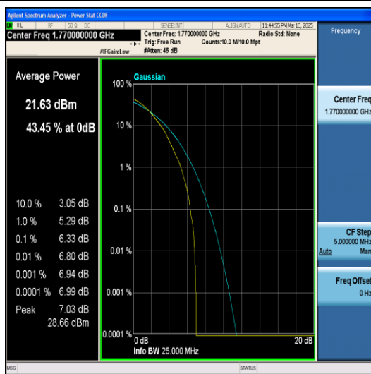
Band66-20MHz-64QAM-132572-1RB#0-PASS
