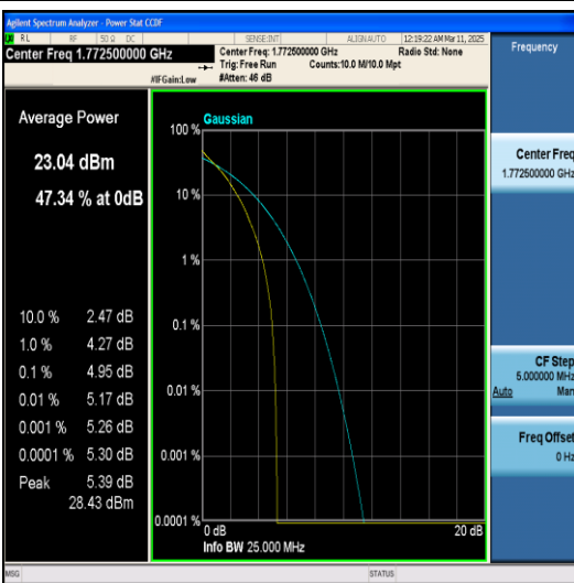
Band66-15MHz-64QAM-132597-1RB#0-PASS
