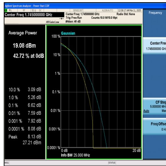
Band66-5MHz-16QAM-132647-1RB#0-PASS
