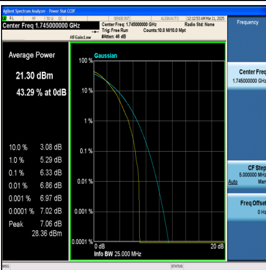
Band66-10MHz-64QAM-132322-1RB#0-PASS
