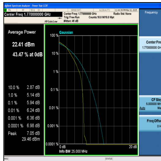
Band66-20MHz-QPSK-132572-100RB#0-PASS
