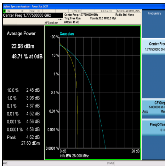
Band66-5MHz-64QAM-132647-1RB#0-PASS
