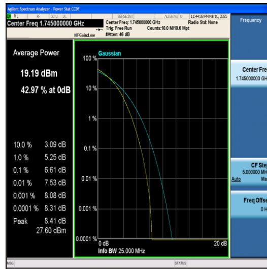
Band66-20MHz-16QAM-132572-1RB#0-PASS
