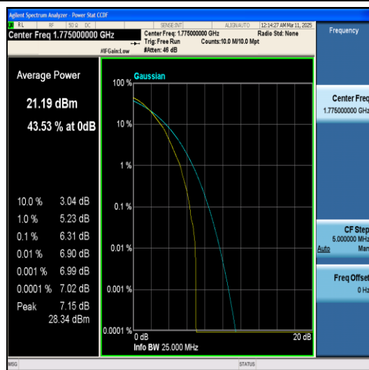
Band66-10MHz-64QAM-132622-1RB#0-PASS
