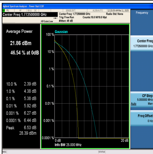
Band66-15MHz-QPSK-132597-75RB#0-PASS
