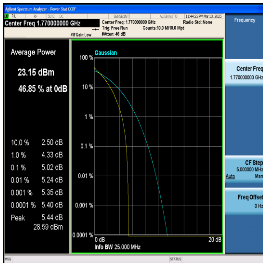
Band66-20MHz-64QAM-132572-1RB#0-PASS
