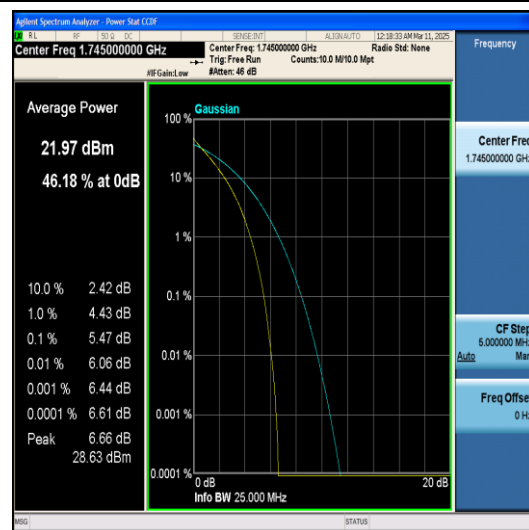
Band66-15MHz-QPSK-132322-75RB#0-PASS
