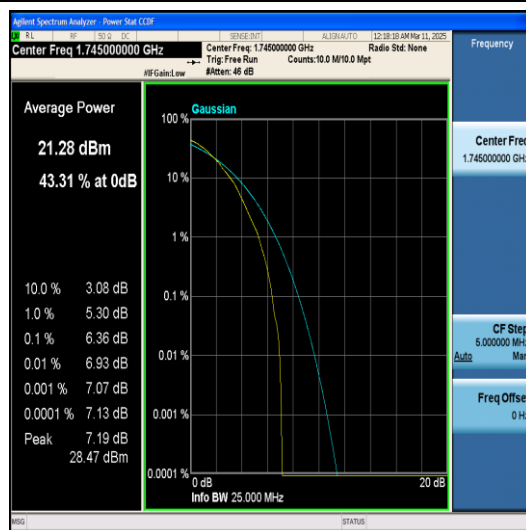
Band66-15MHz-64QAM-132322-1RB#0-PASS
