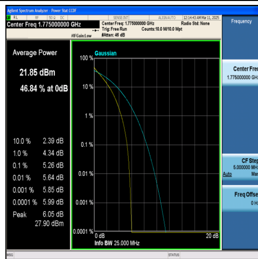
Band66-10MHz-QPSK-132622-50RB#0-PASS
