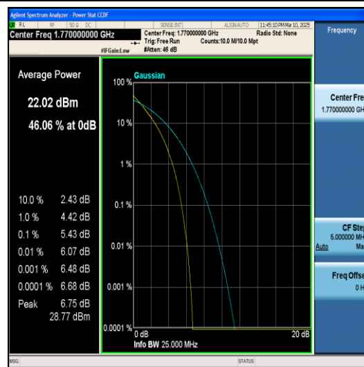
Band66-20MHz-QPSK-132572-100RB#0-PASS
