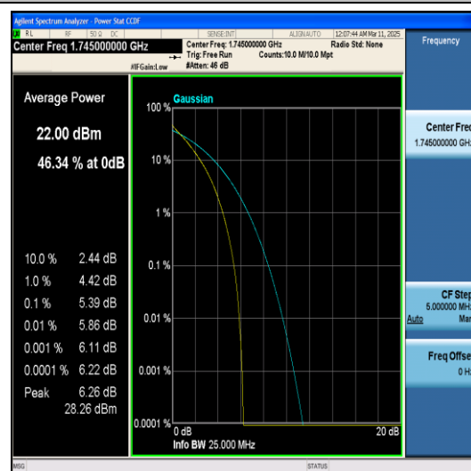
Band66-5MHz-QPSK-132322-25RB#0-PASS
