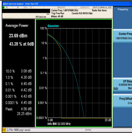
CA_2C-15MHz+20MHz-64QAM-18678+18849- 1RB#74+1RB#0-PASS
