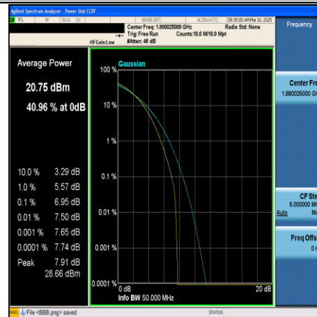
CA_2C-5MHz+20MHz-64QAM-18808+18925- 25RB#0+100RB#0-PASS
