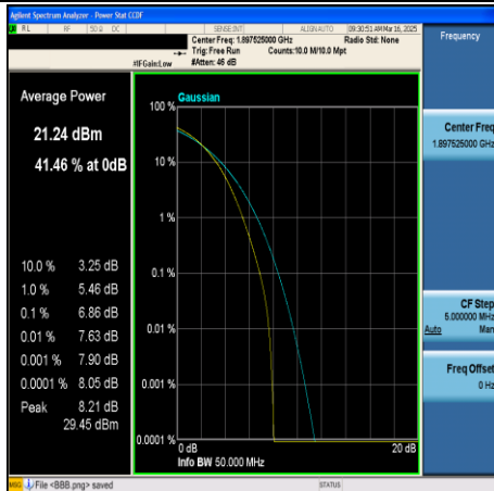
CA_2C-5MHz+20MHz-16QAM-18983+19100- 25RB#0+100RB#0-PASS
