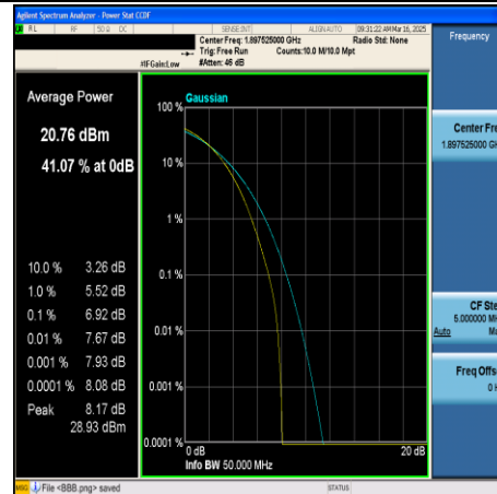
CA_2C-5MHz+20MHz-64QAM-18983+19100- 25RB#0+100RB#0-PASS
