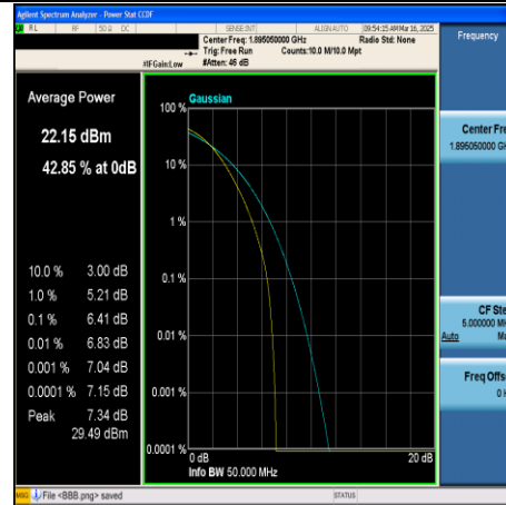
CA_2C-10MHz+20MHz-64QAM-18956+19100- 50RB#0+100RB#0-PASS
