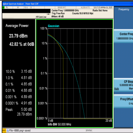
CA_2C-20MHz+20MHz-64QAM-18801+18999- 1RB#99+1RB#0-PASS
