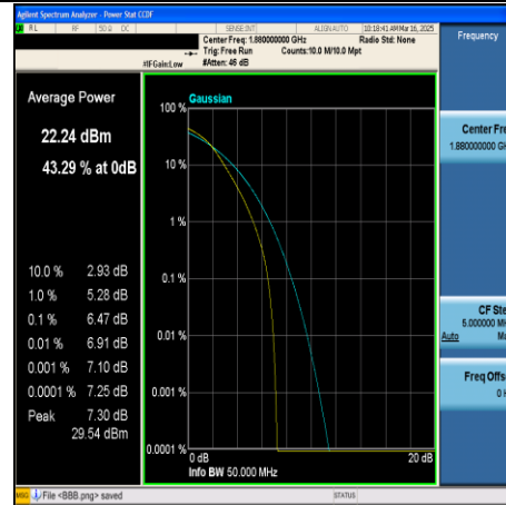
CA_2C-20MHz+20MHz-64QAM-18801+18999- 100RB#0+100RB#0-PASS
