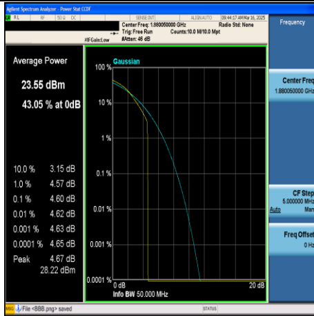
CA_2C-10MHz+20MHz-64QAM-18806+18950- 1RB#49+1RB#0-PASS
