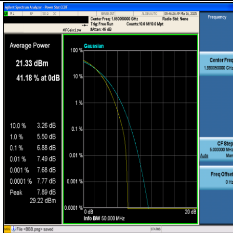
CA_2C-10MHz+20MHz-16QAM-18806+18950- 50RB#0+100RB#0-PASS
