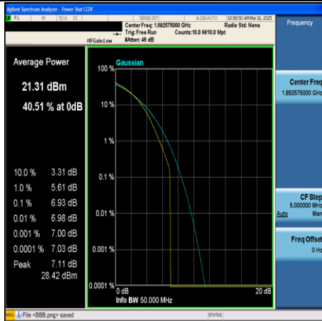
CA_2C-15MHz+20MHz-16QAM-18929+19100- 75RB#0+100RB#0-PASS
