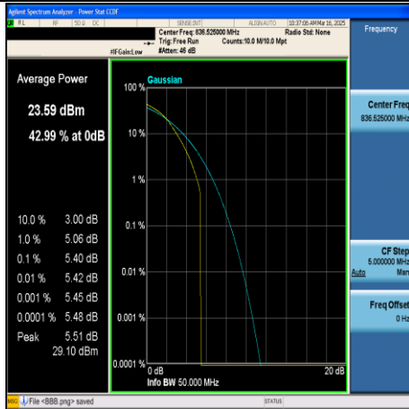
CA_5B-5MHz+10MHz-64QAM-20478+20550- 1RB#24+1RB#0-PASS
