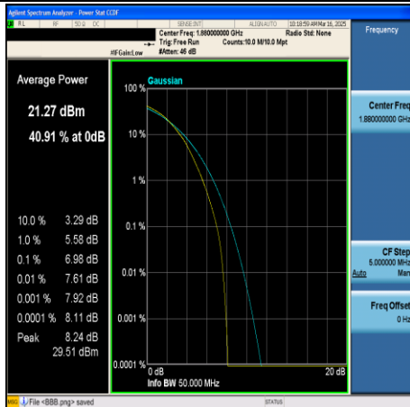
CA_2C-20MHz+20MHz-16QAM-18801+18999- 100RB#0+100RB#0-PASS
