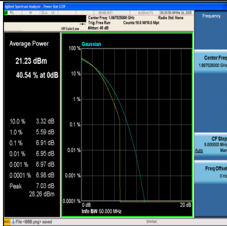
CA_2C-5MHz+20MHz-16QAM-18983+19100- 25RB#0+100RB#0-PASS
