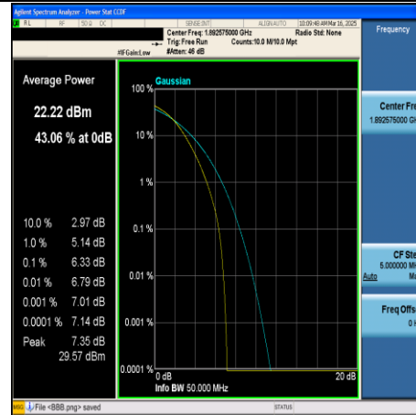
CA_2C-15MHz+20MHz-64QAM-18929+19100- 75RB#0+100RB#0-PASS
