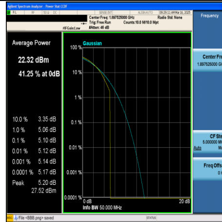
CA_2C-5MHz+20MHz-QPSK-18983+19100- 25RB#0+100RB#0-PASS
