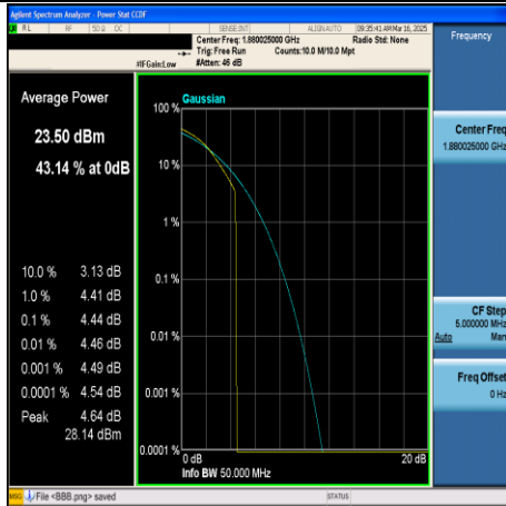
CA_2C-5MHz+20MHz-64QAM-18808+18925- 1RB#24+1RB#0-PASS
