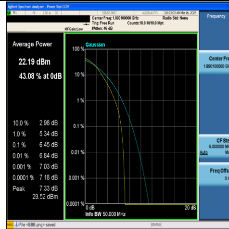
CA_2C-20MHz+20MHz-64QAM-18902+19100- 100RB#0+100RB#0-PASS
