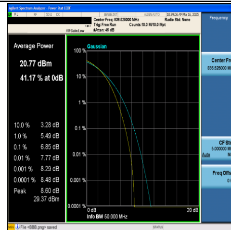
CA_5B-5MHz+10MHz-64QAM-20478+20550- 25RB#0+50RB#0-PASS
