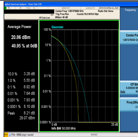
CA_2C-15MHz+20MHz-64QAM-18678+18849- 75RB#0+100RB#0-PASS
