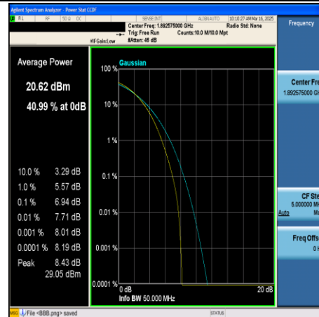
CA_2C-15MHz+20MHz-64QAM-18929+19100- 75RB#0+100RB#0-PASS
