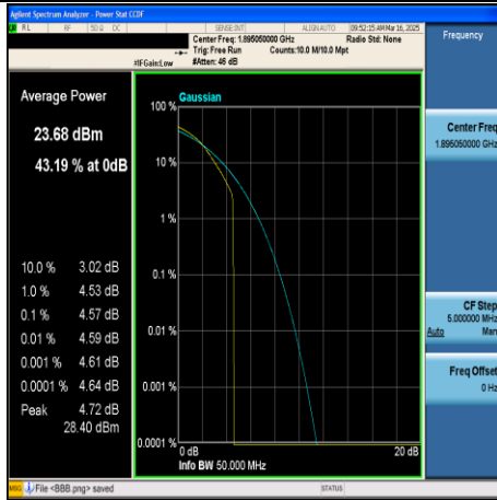
CA_2C-10MHz+20MHz-64QAM-18956+19100- 1RB#49+1RB#0-PASS
