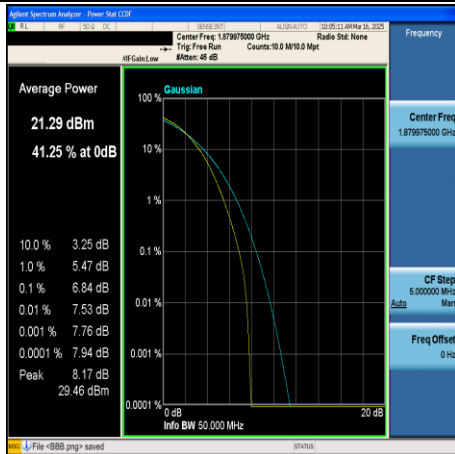
CA_2C-15MHz+20MHz-16QAM-18803+18974- 75RB#0+100RB#0-PASS
