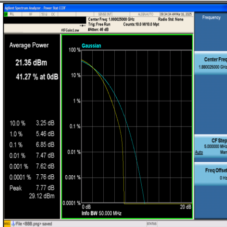
CA_2C-5MHz+20MHz-16QAM-18808+18925- 25RB#0+100RB#0-PASS
