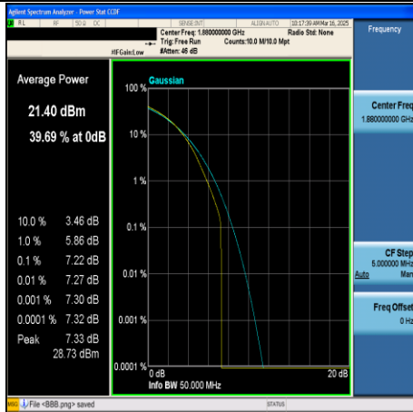
CA_2C-20MHz+20MHz-16QAM-18801+18999- 100RB#0+100RB#0-PASS
