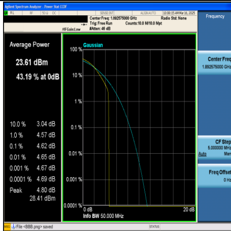
CA_2C-15MHz+20MHz-64QAM-18929+19100- 1RB#74+1RB#0-PASS
