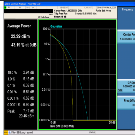
CA_2C-10MHz+20MHz-64QAM-18806+18950- 50RB#0+100RB#0-PASS
