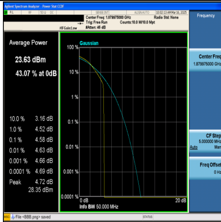
CA_2C-15MHz+20MHz-64QAM-18803+18974- 1RB#74+1RB#0-PASS
