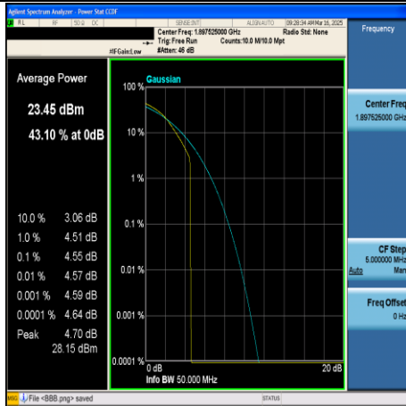
CA_2C-5MHz+20MHz-64QAM-18983+19100- 1RB#24+1RB#0-PASS
