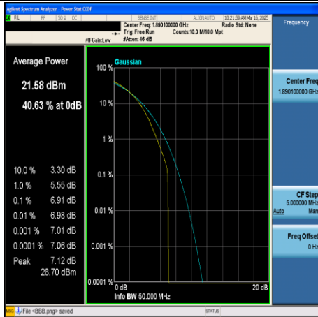
CA_2C-20MHz+20MHz-16QAM-18902+19100- 100RB#0+100RB#0-PASS
