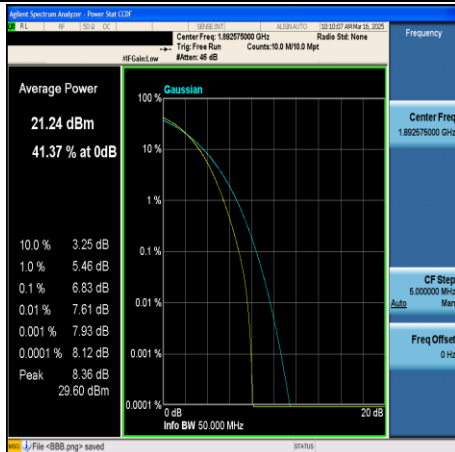
CA_2C-15MHz+20MHz-16QAM-18929+19100- 75RB#0+100RB#0-PASS
