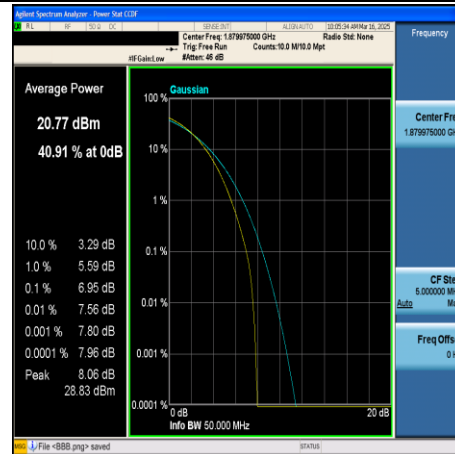
CA_2C-15MHz+20MHz-64QAM-18803+18974- 75RB#0+100RB#0-PASS
