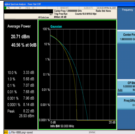
CA_2C-20MHz+20MHz-64QAM-18801+18999- 100RB#0+100RB#0-PASS
