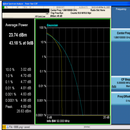
CA_2C-20MHz+20MHz-64QAM-18902+19100- 1RB#99+1RB#0-PASS
