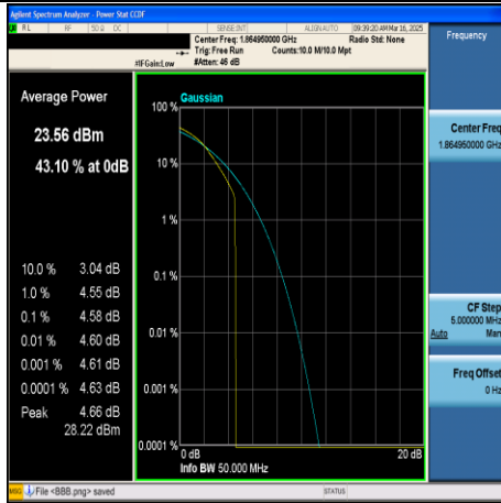
CA_2C-10MHz+20MHz-64QAM-18655+18799- 1RB#49+1RB#0-PASS
