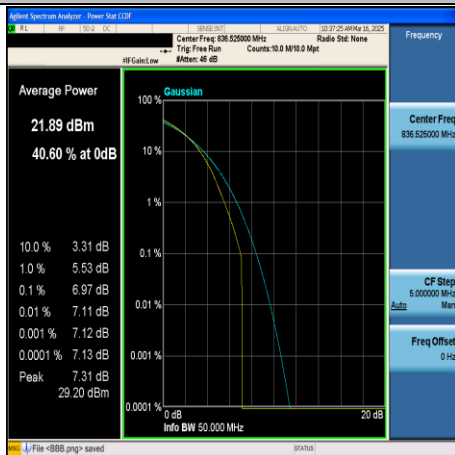
CA_5B-5MHz+10MHz-16QAM-20478+20550- 25RB#0+50RB#0-PASS
