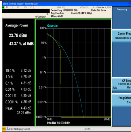
CA_2C-20MHz+20MHz-64QAM-18700+18898- 1RB#99+1RB#0-PASS
