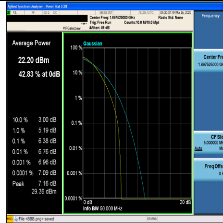
CA_2C-5MHz+20MHz-64QAM-18983+19100- 25RB#0+100RB#0-PASS
