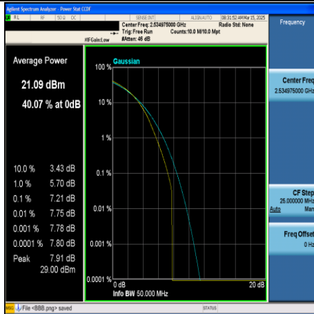
CA_7C-15MHz+20MHz-16QAM-21003+21174- 75RB#0+100RB#0-PASS
