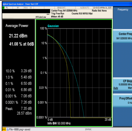
CA_5B-5MHz+10MHz-16QAM-20528+20600- 25RB#0+50RB#0-PASS
