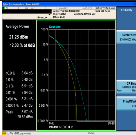
CA_5B-10MHz+10MHz-16QAM-20501+20600- 50RB#0+50RB#0-PASS
