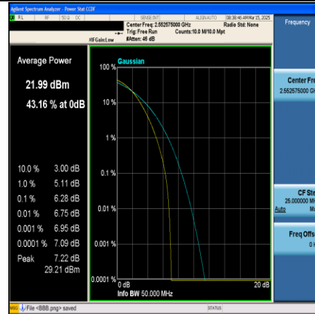
CA_7C-15MHz+20MHz-64QAM-21179+21350- 75RB#0+100RB#0-PASS
