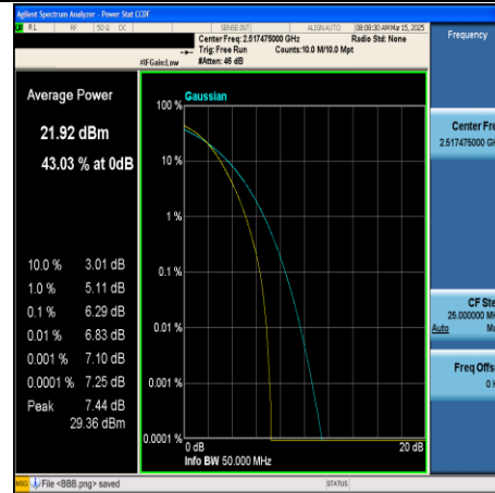
CA_7C-15MHz+20MHz-64QAM-20828+20999- 75RB#0+100RB#0-PASS
