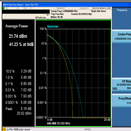
CA_7C-10MHz+20MHz-16QAM-21206+21350- 50RB#0+100RB#0-PASS
