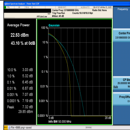
CA_7C-20MHz+20MHz-64QAM-20850+21048- 100RB#0+100RB#0-PASS
