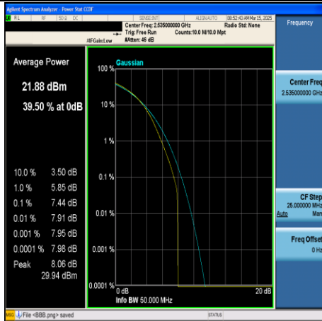
CA_7C-20MHz+20MHz-16QAM-21001+21199- 100RB#0+100RB#0-PASS
