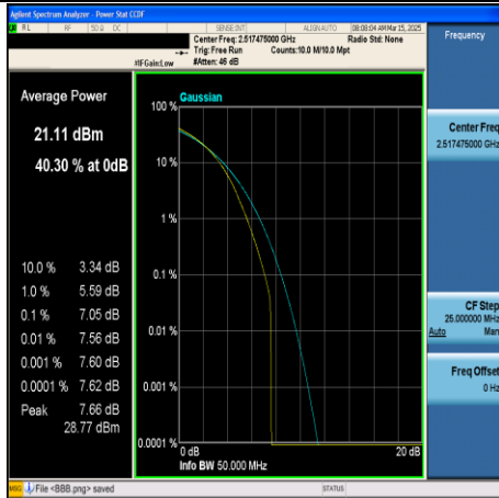
CA_7C-15MHz+20MHz-16QAM-20828+20999- 75RB#0+100RB#0-PASS
