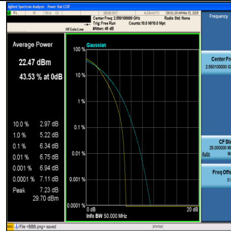
CA_7C-20MHz+20MHz-64QAM-21152+21350- 100RB#0+100RB#0-PASS
