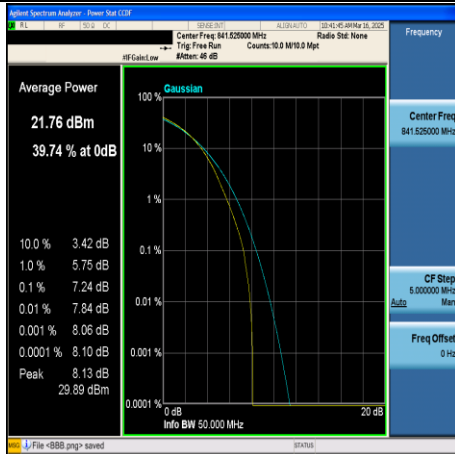
CA_5B-5MHz+10MHz-16QAM-20528+20600- 25RB#0+50RB#0-PASS
