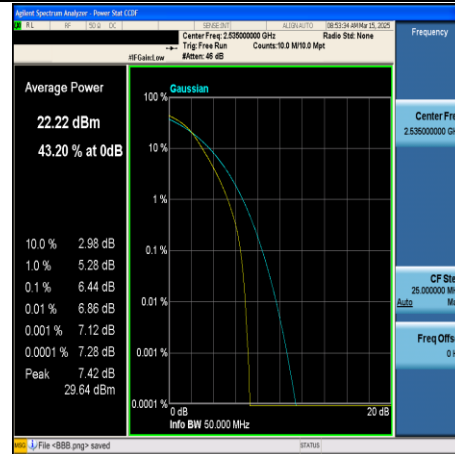
CA_7C-20MHz+20MHz-64QAM-21001+21199- 100RB#0+100RB#0-PASS
