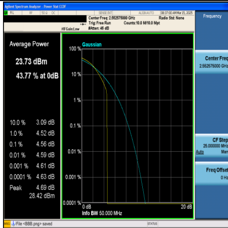
CA_7C-15MHz+20MHz-64QAM-21179+21350- 1RB#74+1RB#0-PASS
