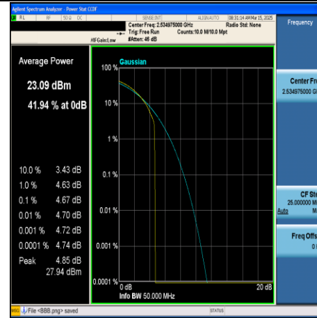
CA_7C-15MHz+20MHz-QPSK-21003+21174- 75RB#0+100RB#0-PASS
