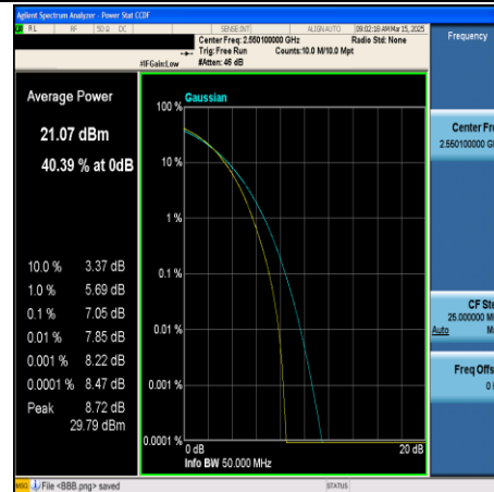
CA_7C-20MHz+20MHz-64QAM-21152+21350- 100RB#0+100RB#0-PASS
