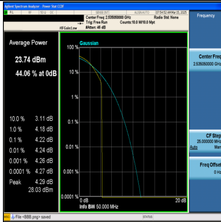
CA_7C-10MHz+20MHz-64QAM-21006+21150- 1RB#49+1RB#0-PASS
