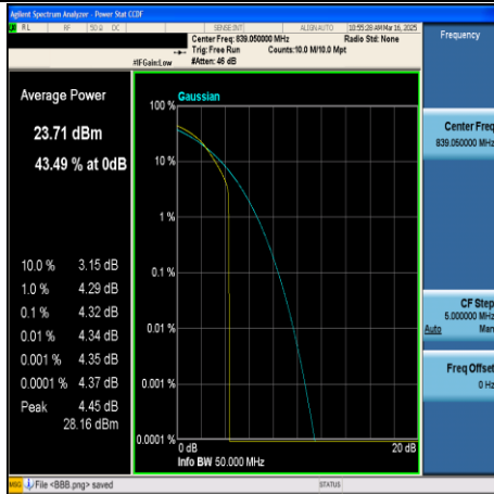
CA_5B-10MHz+10MHz-64QAM-20501+20600- 1RB#49+1RB#0-PASS
