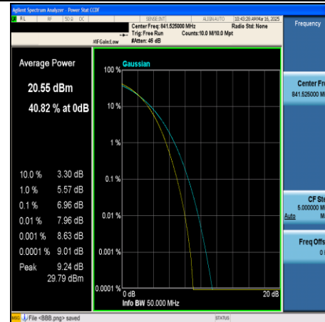
CA_5B-5MHz+10MHz-64QAM-20528+20600- 25RB#0+50RB#0-PASS
