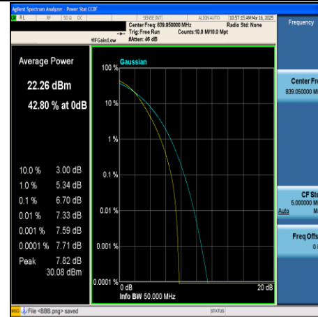
CA_5B-10MHz+10MHz-64QAM-20501+20600- 50RB#0+50RB#0-PASS
