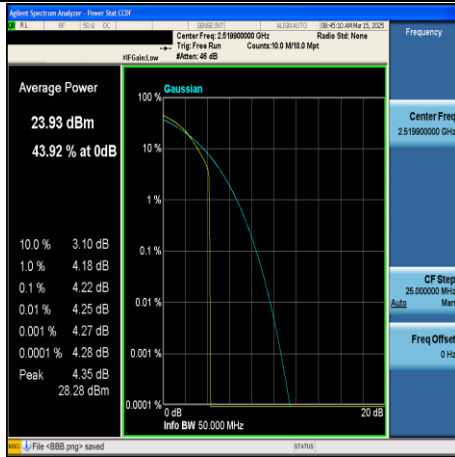
CA_7C-20MHz+20MHz-64QAM-20850+21048- 1RB#99+1RB#0-PASS
