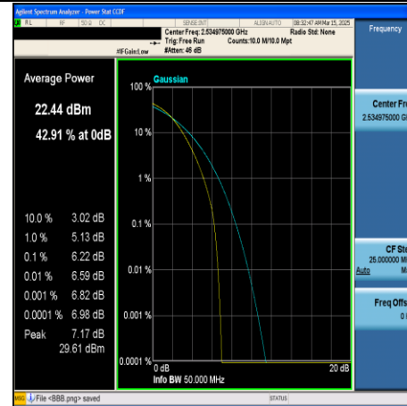
CA_7C-15MHz+20MHz-64QAM-21003+21174- 75RB#0+100RB#0-PASS
