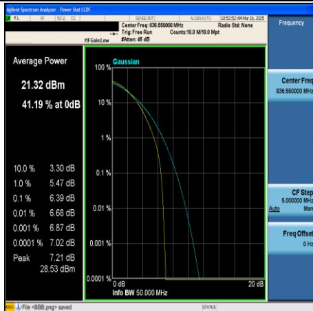
CA_5B-10MHz+10MHz-16QAM-20476+20575- 50RB#0+50RB#0-PASS
