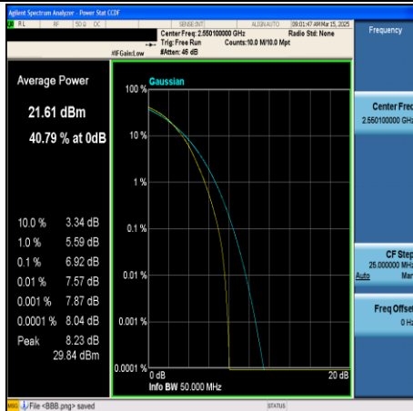
CA_7C-20MHz+20MHz-16QAM-21152+21350- 100RB#0+100RB#0-PASS
