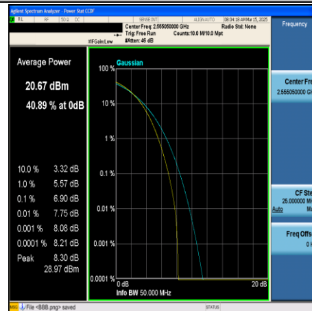
CA_7C-10MHz+20MHz-64QAM-21206+21350- 50RB#0+100RB#0-PASS
