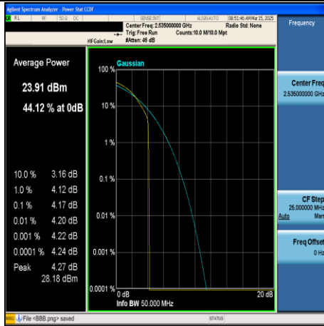
CA_7C-20MHz+20MHz-64QAM-21001+21199- 1RB#99+1RB#0-PASS
