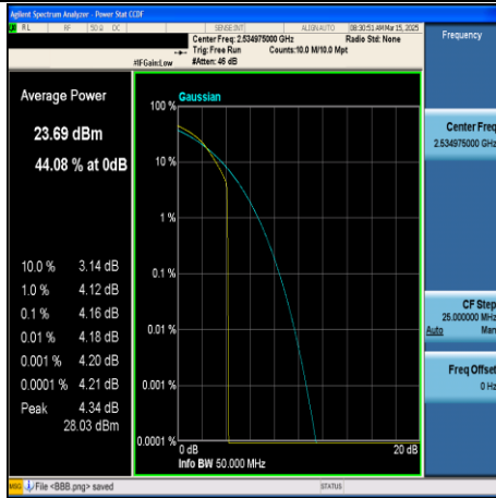
CA_7C-15MHz+20MHz-64QAM-21003+21174- 1RB#74+1RB#0-PASS
