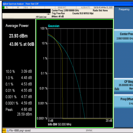
CA_7C-20MHz+20MHz-64QAM-21152+21350- 1RB#99+1RB#0-PASS
