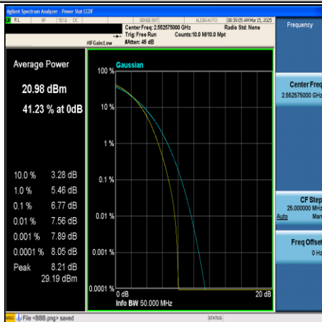
CA_7C-15MHz+20MHz-16QAM-21179+21350- 75RB#0+100RB#0-PASS
