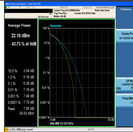
CA_5B-5MHz+10MHz-64QAM-20528+20600- 25RB#0+50RB#0-PASS
