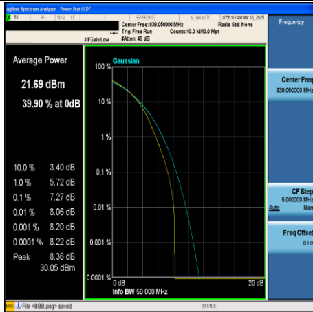
CA_5B-10MHz+10MHz-16QAM-20501+20600- 50RB#0+50RB#0-PASS
