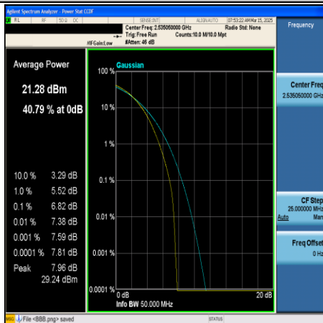
CA_7C-10MHz+20MHz-16QAM-21006+21150- 50RB#0+100RB#0-PASS
