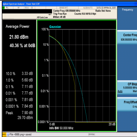
CA_5B-10MHz+10MHz-16QAM-20476+20575- 50RB#0+50RB#0-PASS
