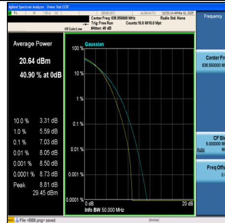
CA_5B-10MHz+10MHz-64QAM-20476+20575- 50RB#0+50RB#0-PASS
