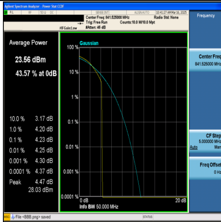
CA_5B-5MHz+10MHz-64QAM-20528+20600- 1RB#24+1RB#0-PASS
