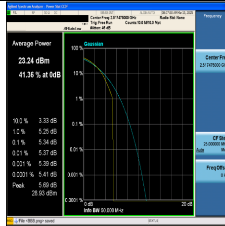
CA_7C-15MHz+20MHz-QPSK-20828+20999- 75RB#0+100RB#0-PASS
