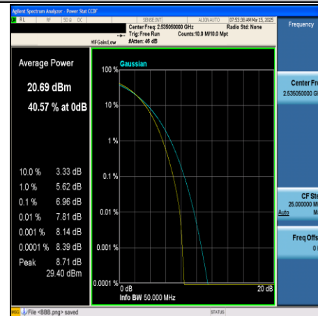
CA_7C-10MHz+20MHz-64QAM-21006+21150- 50RB#0+100RB#0-PASS
