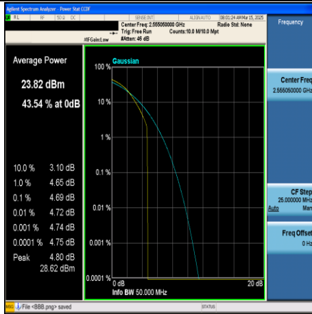
CA_7C-10MHz+20MHz-64QAM-21206+21350- 1RB#49+1RB#0-PASS
