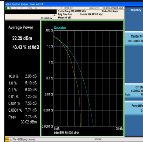
CA_5B-10MHz+10MHz-64QAM-20476+20575- 50RB#0+50RB#0-PASS
