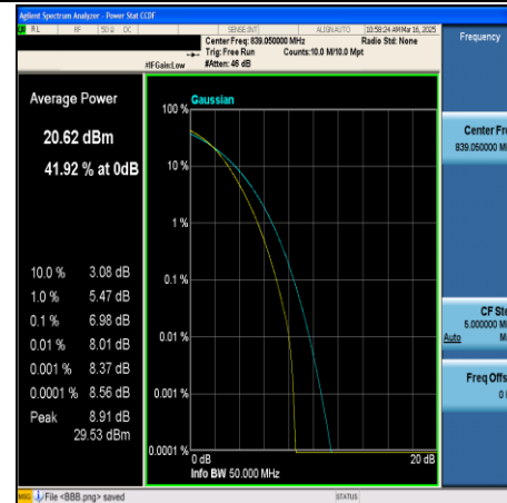
CA_5B-10MHz+10MHz-64QAM-20501+20600- 50RB#0+50RB#0-PASS
