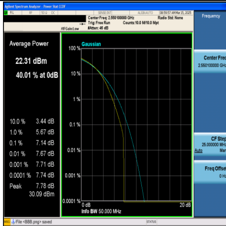
CA_7C-20MHz+20MHz-16QAM-21152+21350- 100RB#0+100RB#0-PASS
