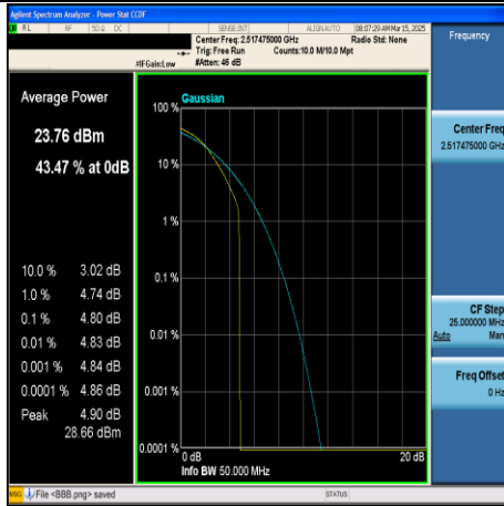
CA_7C-15MHz+20MHz-64QAM-20828+20999- 1RB#74+1RB#0-PASS
