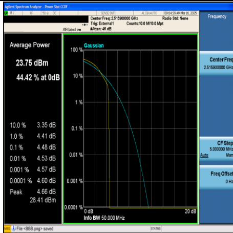
CA_41C-20MHz+20MHz-64QAM-39750+39948- 1RB#99+1RB#0-PASS
