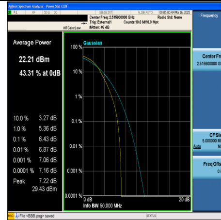
CA_41C-20MHz+20MHz-64QAM-39750+39948- 100RB#0+100RB#0-PASS
