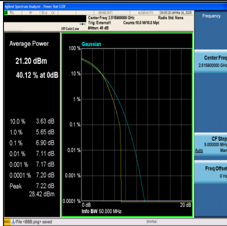
CA_41C-20MHz+20MHz-16QAM-39750+39948- 100RB#0+100RB#0-PASS
