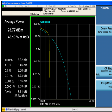
CA_41C-20MHz+20MHz-64QAM-41292+41490- 1RB#99+1RB#0-PASS
