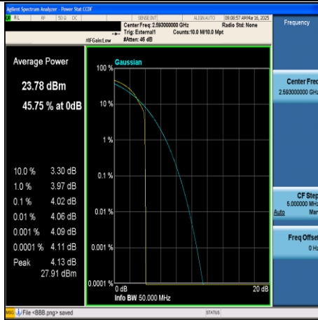
CA_41C-20MHz+20MHz-64QAM-40521+40719- 1RB#99+1RB#0-PASS
