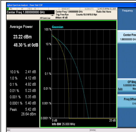
Band2-15MHz-64QAM-18900-1RB#0-PASS
