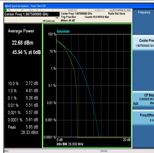
Band2-5MHz-QPSK-19175-25RB#0-PASS
