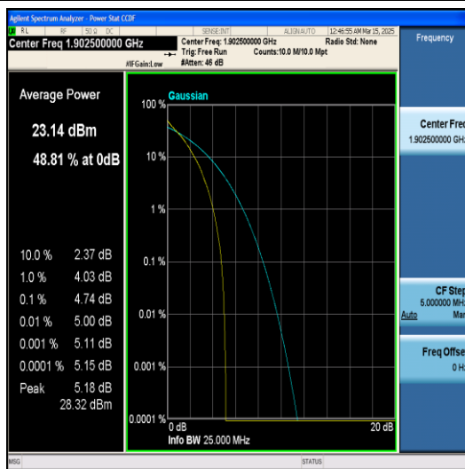
Band2-15MHz-64QAM-19125-1RB#0-PASS
