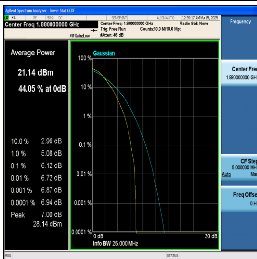
Band2-10MHz-64QAM-18900-1RB#0-PASS
