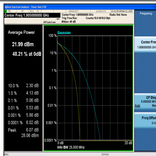
Band2-10MHz-QPSK-19150-50RB#0-PASS
