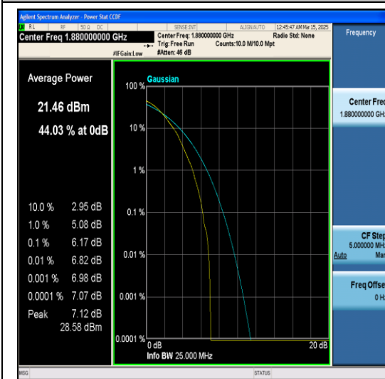
Band2-15MHz-64QAM-18900-1RB#0-PASS
