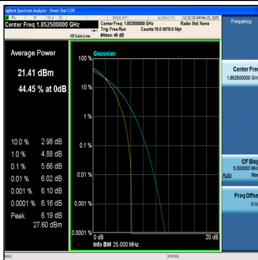
Band2-5MHz-64QAM-18625-1RB#0-PASS
