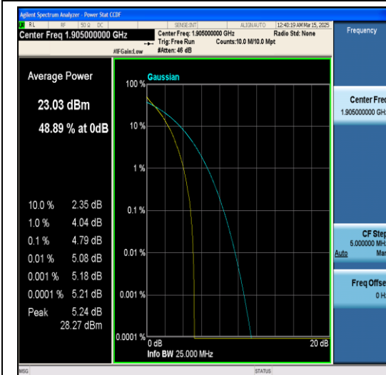
Band2-10MHz-64QAM-19150-1RB#0-PASS
