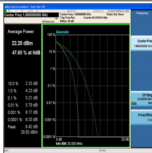
Band2-15MHz-QPSK-18900-75RB#0-PASS
