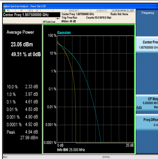
Band2-5MHz-64QAM-19175-1RB#0-PASS
