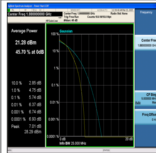
Band2-10MHz-QPSK-19150-1RB#0-PASS
