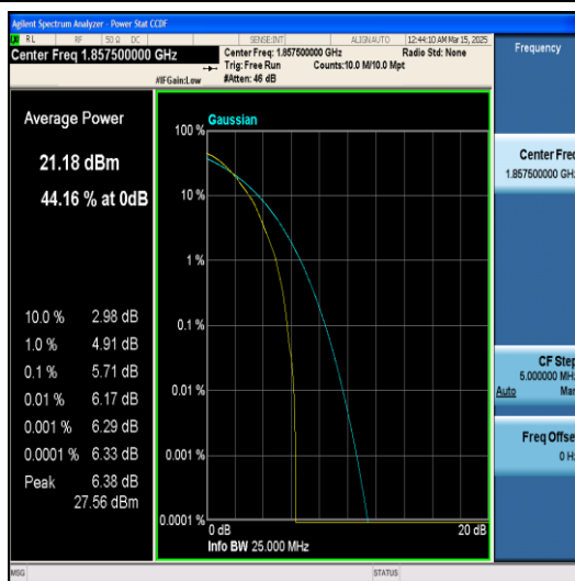
Band2-15MHz-64QAM-18675-1RB#0-PASS
