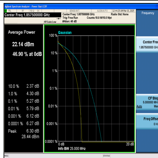
Band2-15MHz-QPSK-18675-75RB#0-PASS
