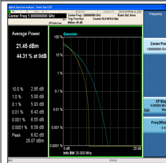
Band2-20MHz-64QAM-19100-1RB#0-PASS
