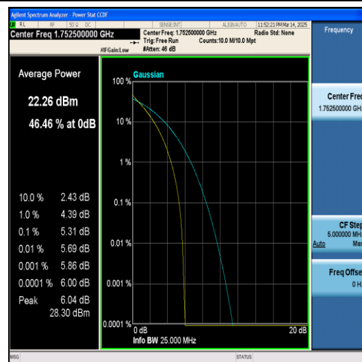
Band4-5MHz-QPSK-20375-25RB#0-PASS
