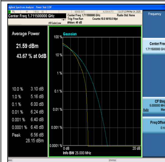
Band4-3MHz-64QAM-19965-1RB#0-PASS
