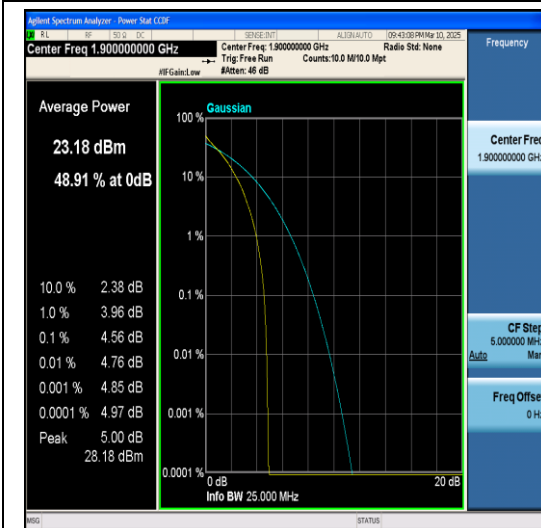
Band2-20MHz-64QAM-19100-1RB#0-PASS
