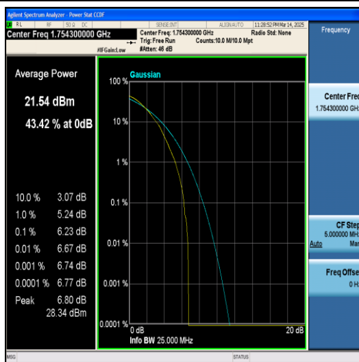
Band4-1.4MHz-64QAM-20393-1RB#0-PASS
