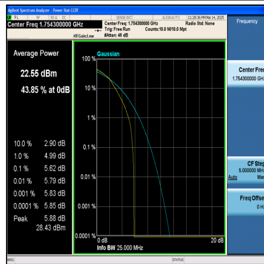
Band4-1.4MHz-QPSK-20393-6RB#0-PASS
