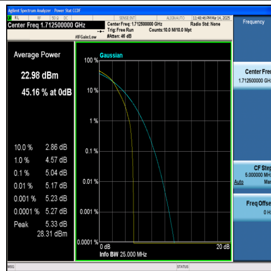
Band4-5MHz-QPSK-19975-25RB#0-PASS
