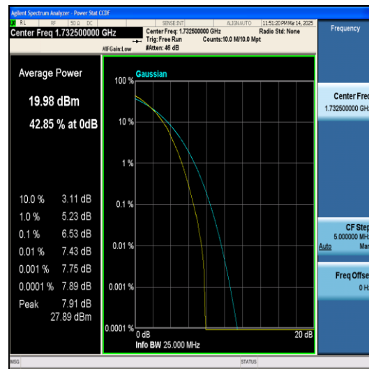
Band4-5MHz-16QAM-20375-1RB#0-PASS
