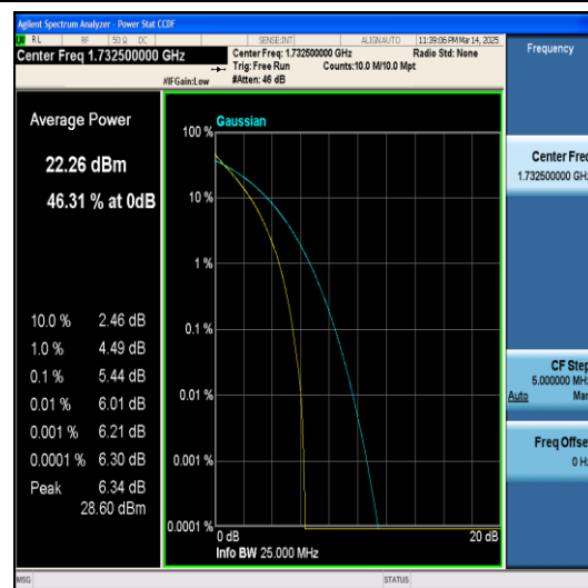
Band4-3MHz-QPSK-20175-15RB#0-PASS
