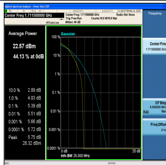
Band4-3MHz-QPSK-19965-15RB#0-PASS
