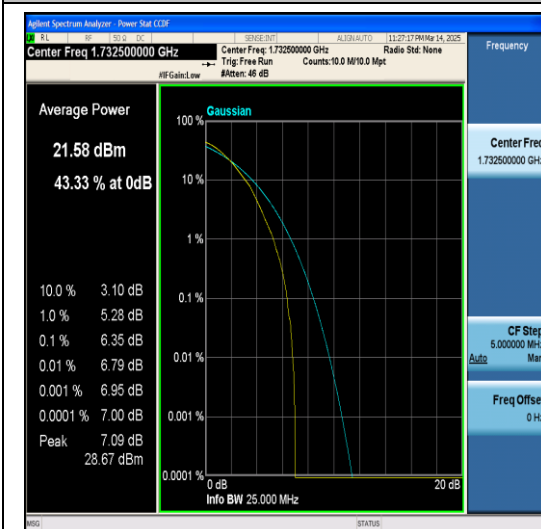
Band4-1.4MHz-64QAM-20175-1RB#0-PASS
