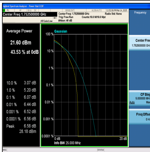
Band4-5MHz-64QAM-20375-1RB#0-PASS
