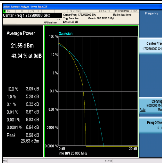
Band4-3MHz-64QAM-20175-1RB#0-PASS
