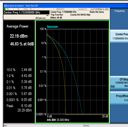
Band4-1.4MHz-QPSK-20175-6RB#0-PASS
