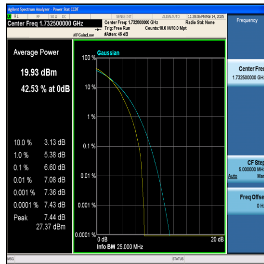
Band4-1.4MHz-16QAM-20393-1RB#0-PASS
