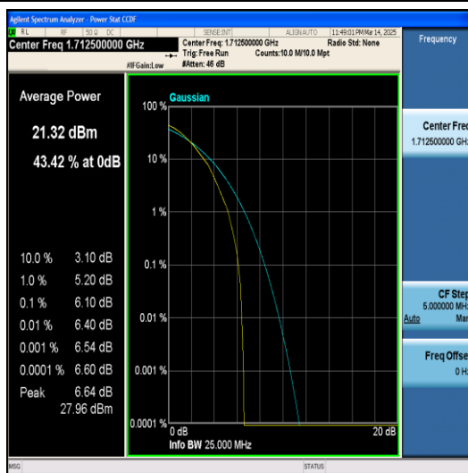
Band4-5MHz-64QAM-19975-1RB#0-PASS
