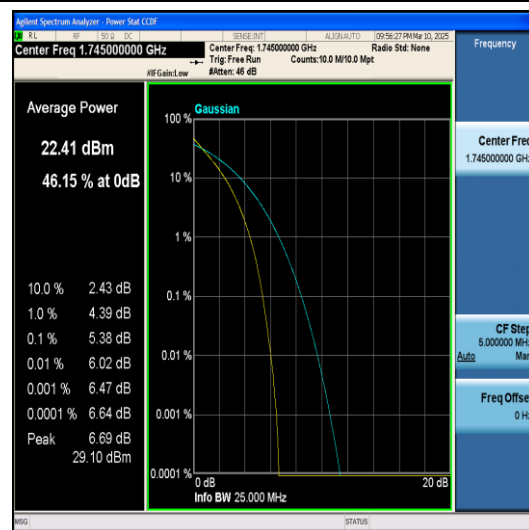
Band4-20MHz-QPSK-20300-100RB#0-PASS
