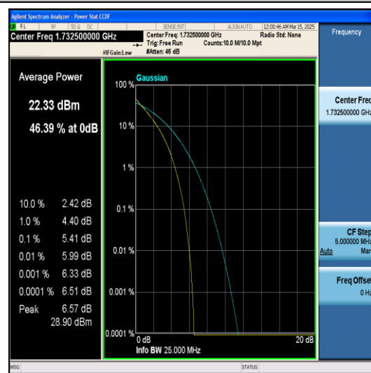
Band4-15MHz-QPSK-20175-75RB#0-PASS
