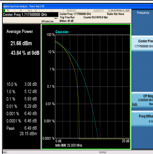
Band4-15MHz-64QAM-20025-1RB#0-PASS
