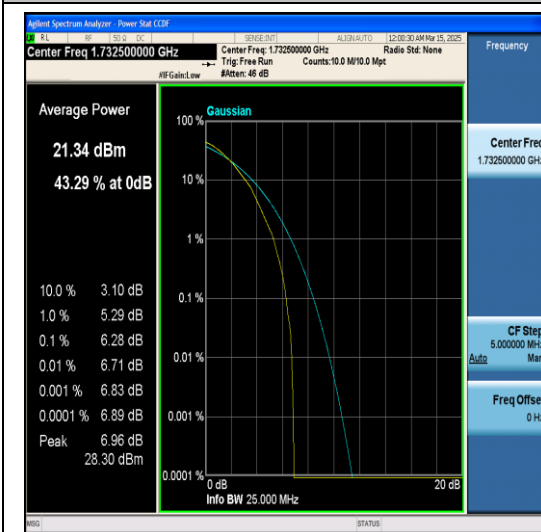
Band4-15MHz-64QAM-20175-1RB#0-PASS
