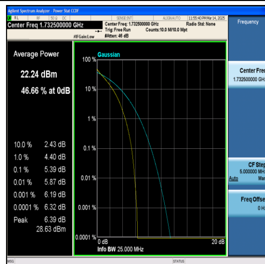
Band4-10MHz-QPSK-20175-50RB#0-PASS
