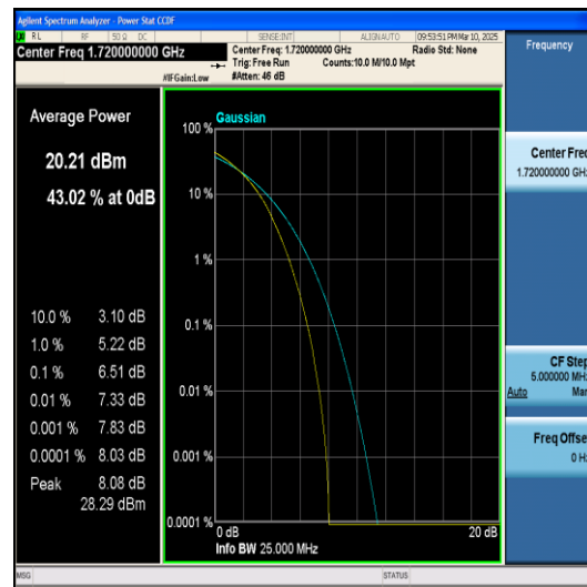
Band4-20MHz-16QAM-20175-1RB#0-PASS
