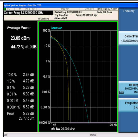
Band4-15MHz-QPSK-20175-75RB#0-PASS
