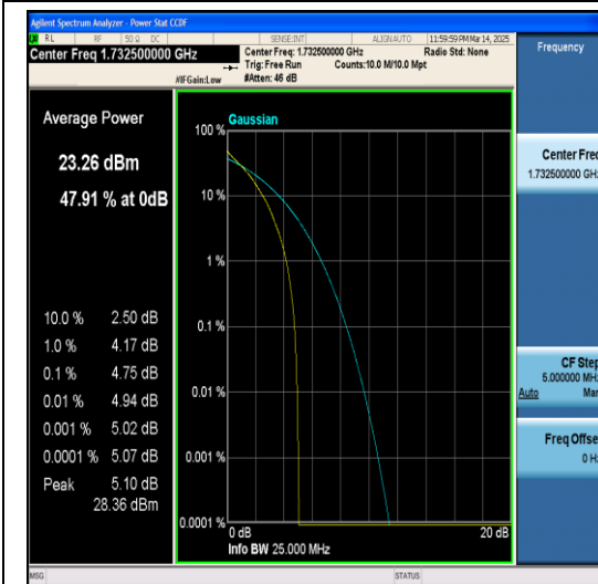
Band4-15MHz-64QAM-20175-1RB#0-PASS
