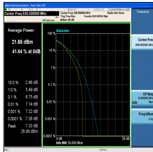
Band5-1.4MHz-QPSK-20525-6RB#0-PASS
