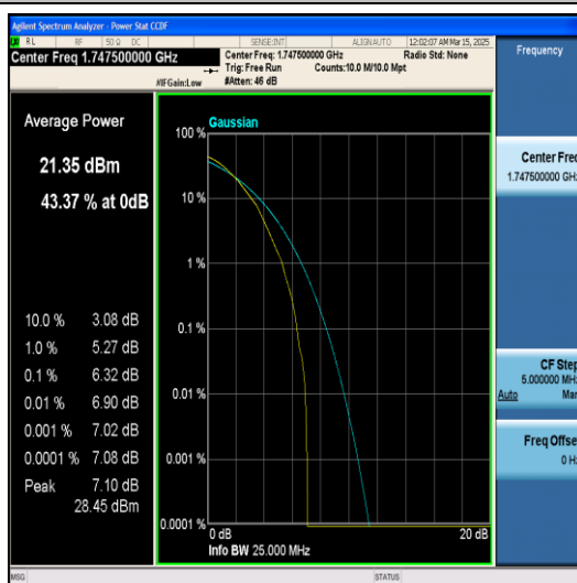
Band4-15MHz-64QAM-20325-1RB#0-PASS
