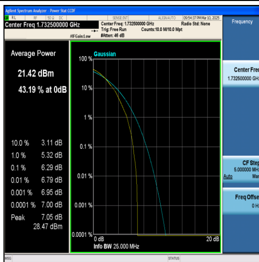
Band4-20MHz-64QAM-20175-1RB#0-PASS
