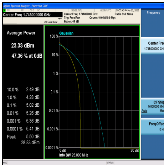
Band4-20MHz-64QAM-20300-1RB#0-PASS
