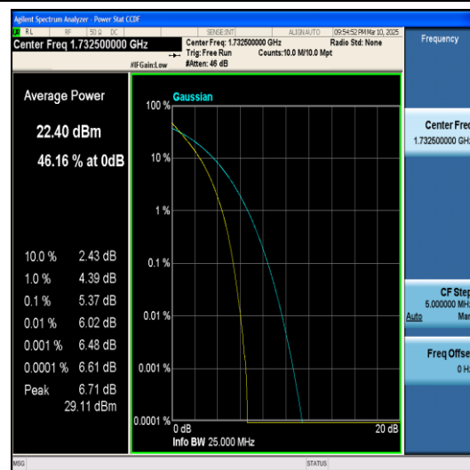
Band4-20MHz-QPSK-20175-100RB#0-PASS
