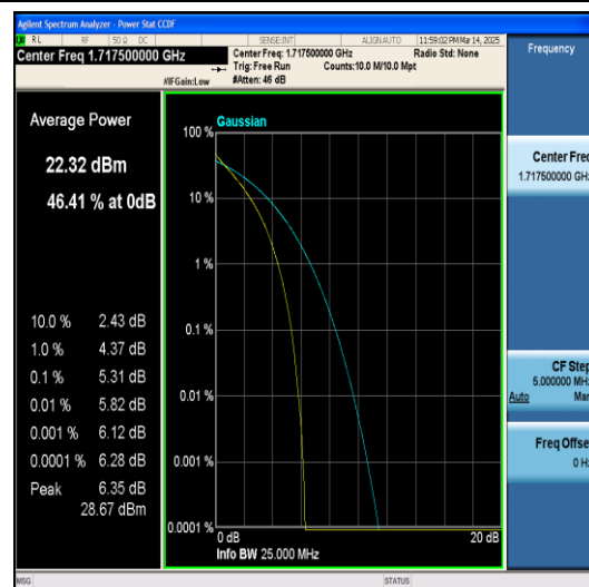
Band4-15MHz-QPSK-20025-75RB#0-PASS
