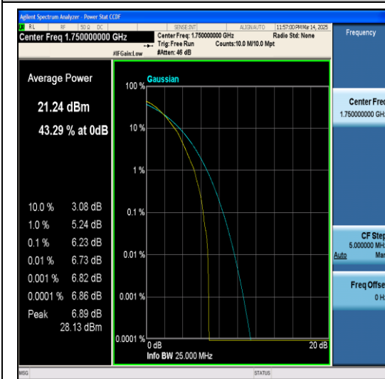
Band4-10MHz-64QAM-20350-1RB#0-PASS
