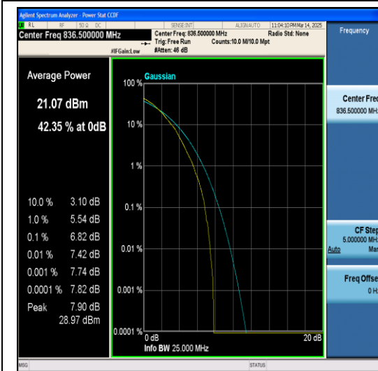
Band5-1.4MHz-64QAM-20525-1RB#0-PASS
