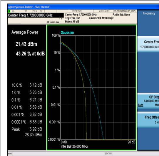
Band4-20MHz-64QAM-20050-1RB#0-PASS
