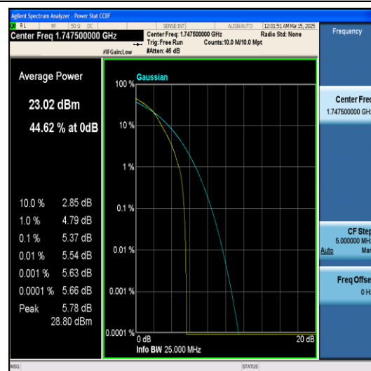
Band4-15MHz-QPSK-20325-75RB#0-PASS
