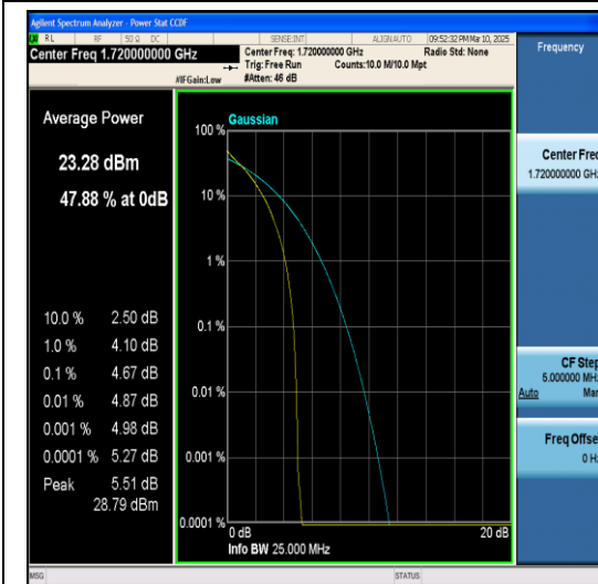
Band4-20MHz-64QAM-20050-1RB#0-PASS
