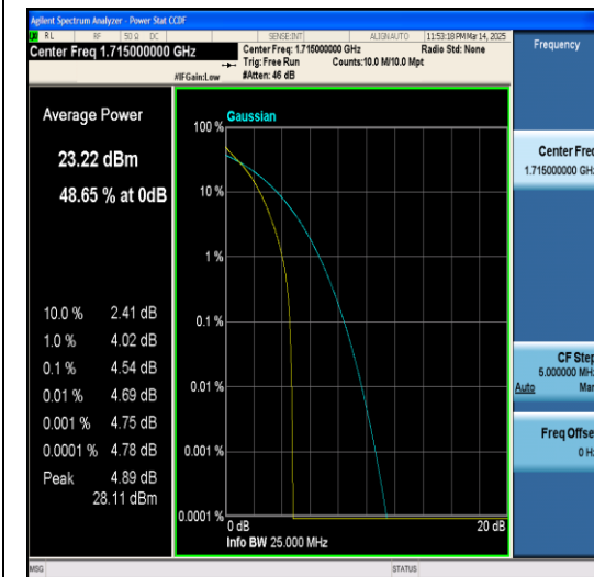
Band4-10MHz-64QAM-20000-1RB#0-PASS
