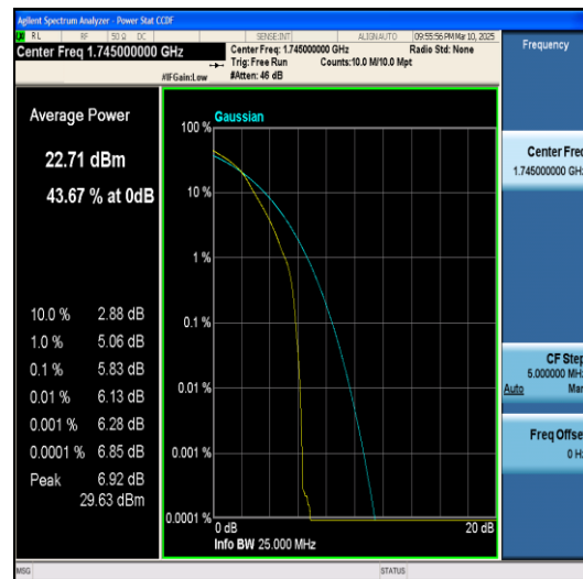
Band4-20MHz-QPSK-20300-100RB#0-PASS
