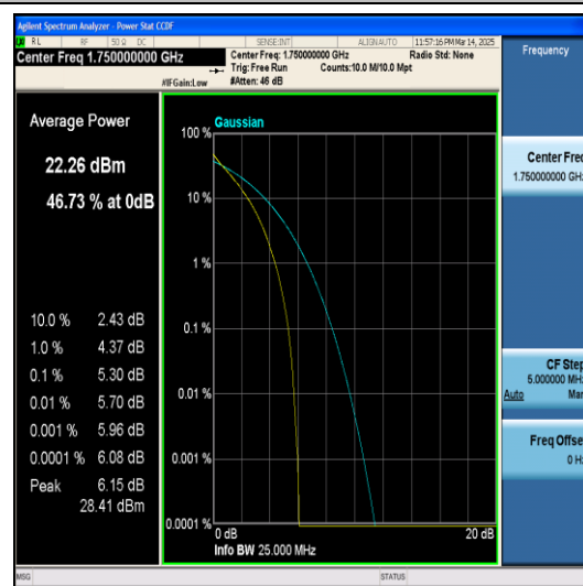
Band4-10MHz-QPSK-20350-50RB#0-PASS
