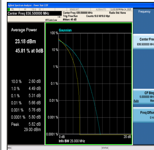
Band5-1.4MHz-64QAM-20525-1RB#0-PASS
