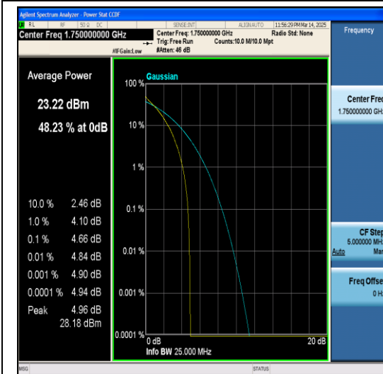
Band4-10MHz-64QAM-20350-1RB#0-PASS
