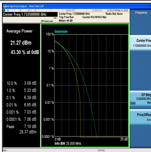
Band4-10MHz-64QAM-20175-1RB#0-PASS
