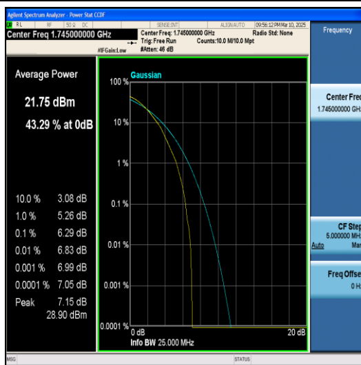
Band4-20MHz-64QAM-20300-1RB#0-PASS
