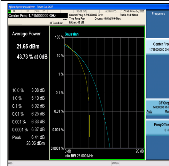
Band4-10MHz-64QAM-20000-1RB#0-PASS
