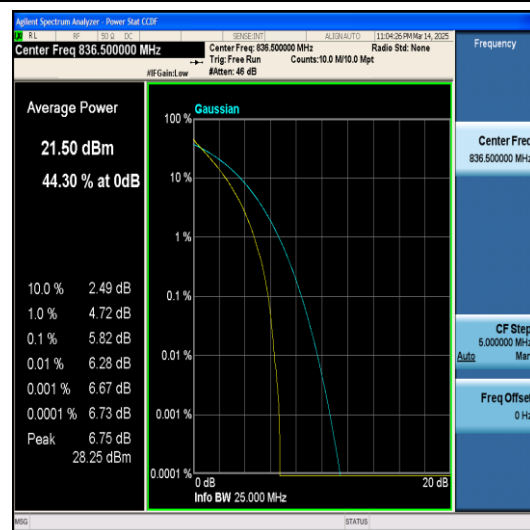
Band5-1.4MHz-QPSK-20525-6RB#0-PASS
