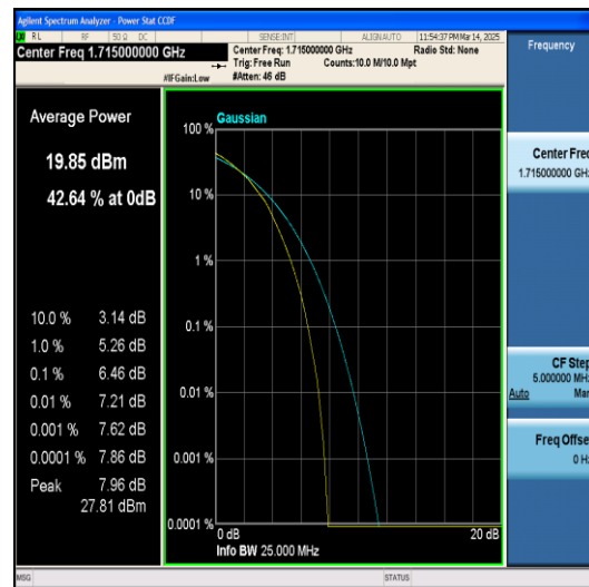
Band4-10MHz-16QAM-20175-1RB#0-PASS
