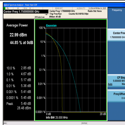
Band4-10MHz-QPSK-20350-50RB#0-PASS
