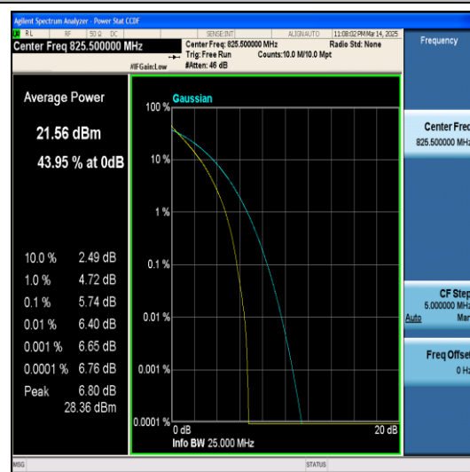
Band5-3MHz-QPSK-20415-15RB#0-PASS
