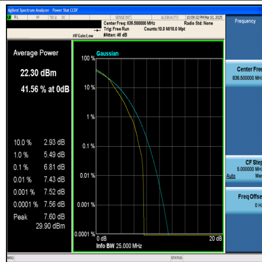
Band5-10MHz-QPSK-20525-50RB#0-PASS
