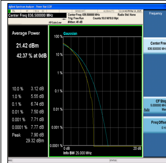
Band5-5MHz-64QAM-20525-1RB#0-PASS
