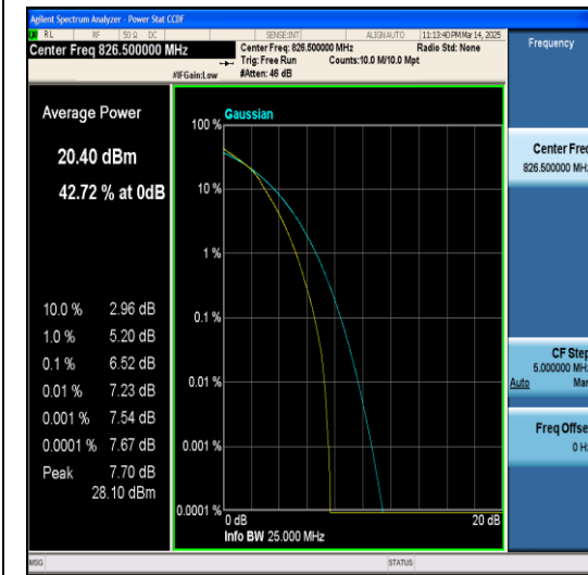
Band5-5MHz-QPSK-20525-1RB#0-PASS
