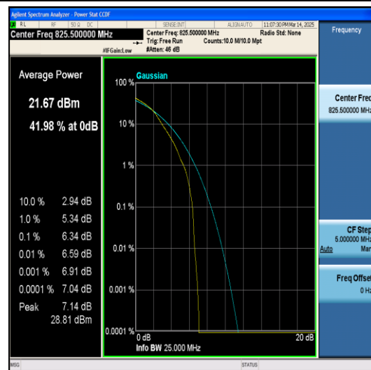
Band5-3MHz-QPSK-20415-15RB#0-PASS
