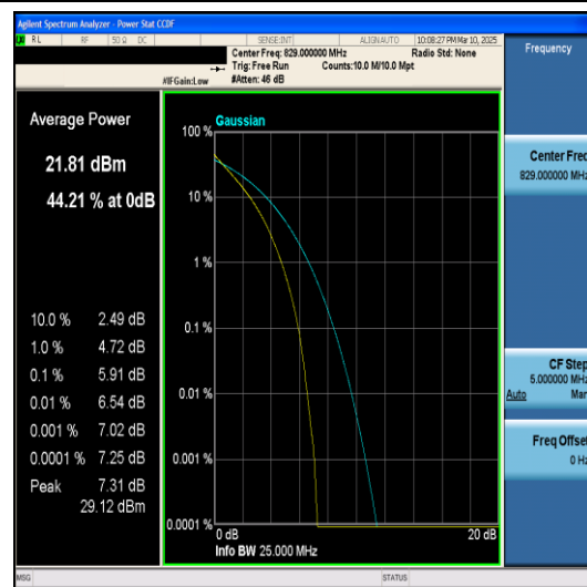
Band5-10MHz-QPSK-20450-50RB#0-PASS
