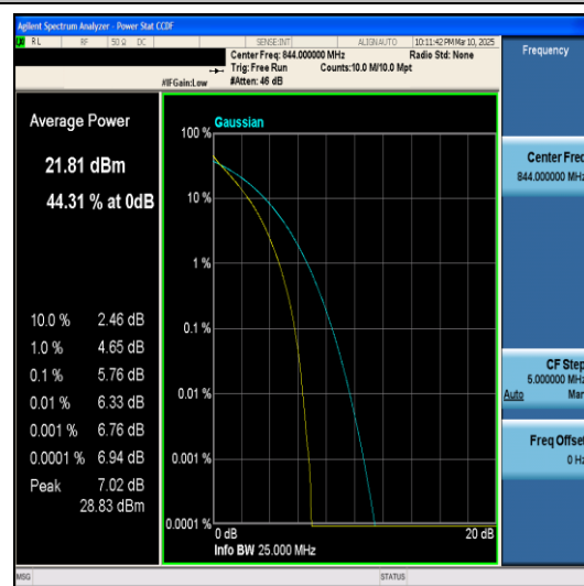
Band5-10MHz-QPSK-20600-50RB#0-PASS
