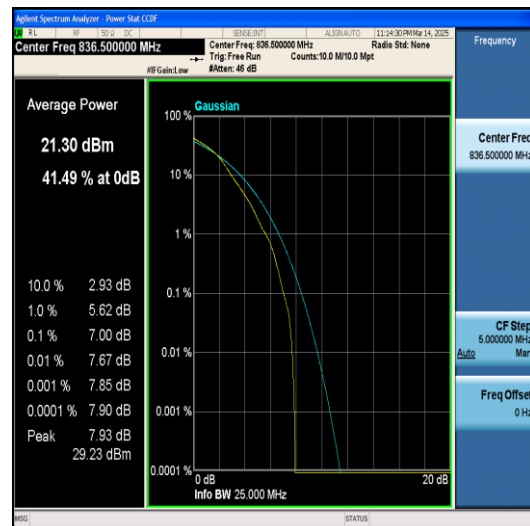
Band5-5MHz-QPSK-20525-25RB#0-PASS
