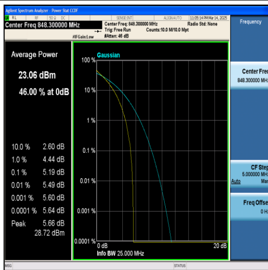
Band5-1.4MHz-64QAM-20643-1RB#0-PASS
