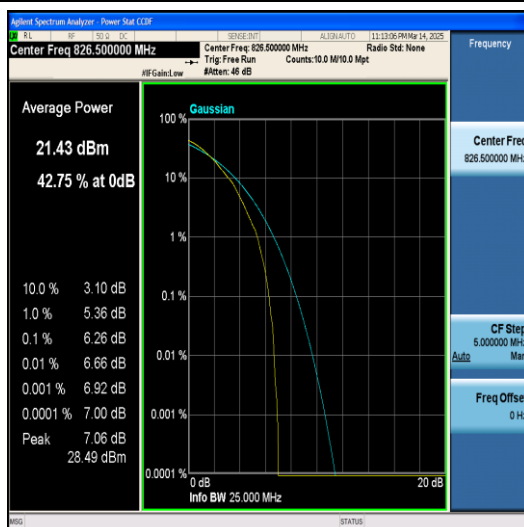
Band5-5MHz-64QAM-20425-1RB#0-PASS
