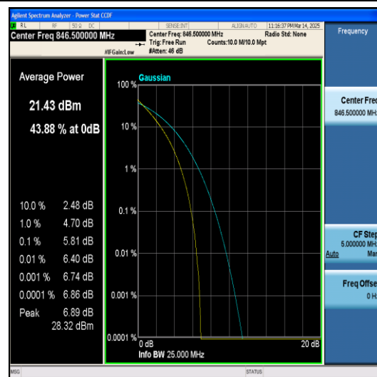
Band5-5MHz-QPSK-20625-25RB#0-PASS
