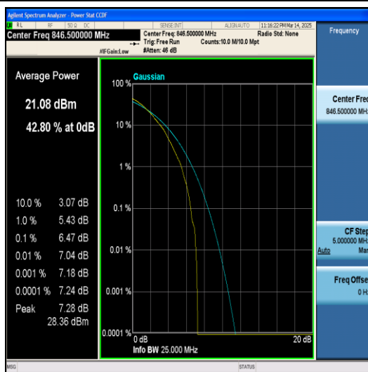
Band5-5MHz-64QAM-20625-1RB#0-PASS
