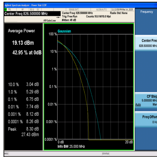
Band5-5MHz-16QAM-20525-1RB#0-PASS
