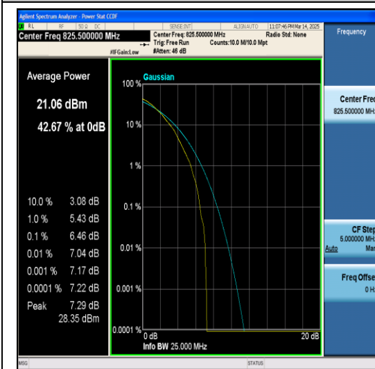
Band5-3MHz-64QAM-20415-1RB#0-PASS
