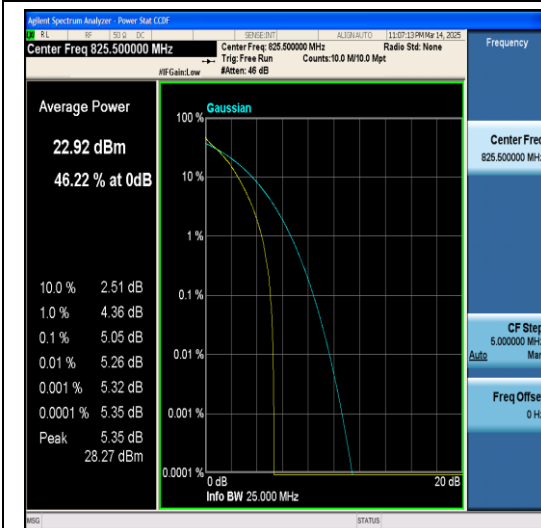
Band5-3MHz-64QAM-20415-1RB#0-PASS
