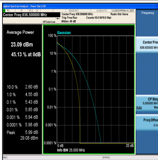
Band5-3MHz-64QAM-20525-1RB#0-PASS
