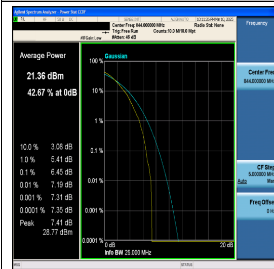
Band5-10MHz-64QAM-20600-1RB#0-PASS
