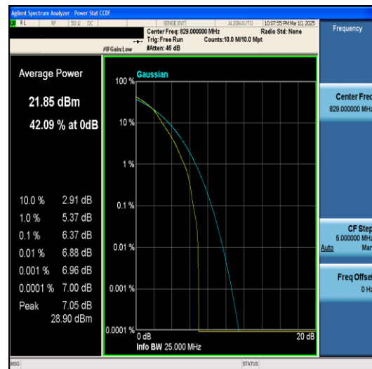
Band5-10MHz-QPSK-20450-50RB#0-PASS
