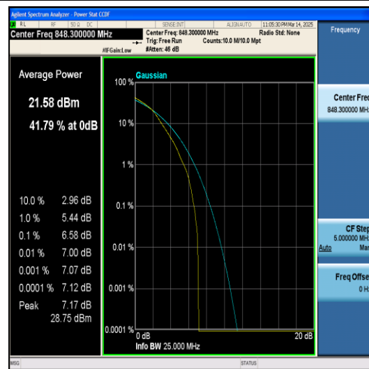
Band5-1.4MHz-QPSK-20643-6RB#0-PASS
