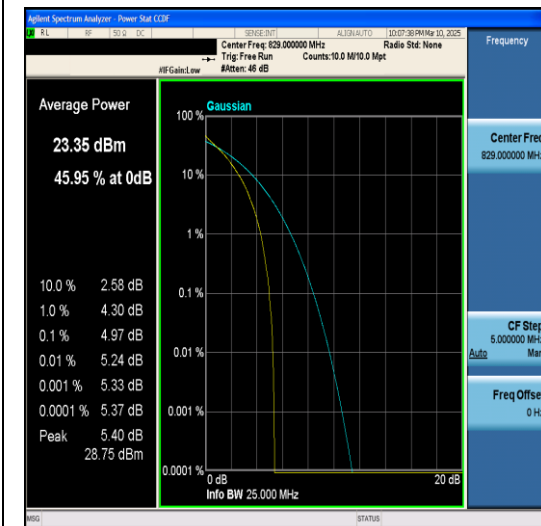
Band5-10MHz-64QAM-20450-1RB#0-PASS
