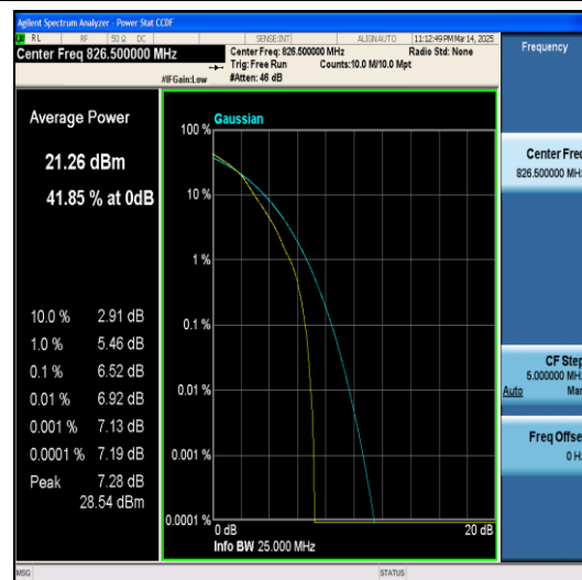
Band5-5MHz-QPSK-20425-25RB#0-PASS
