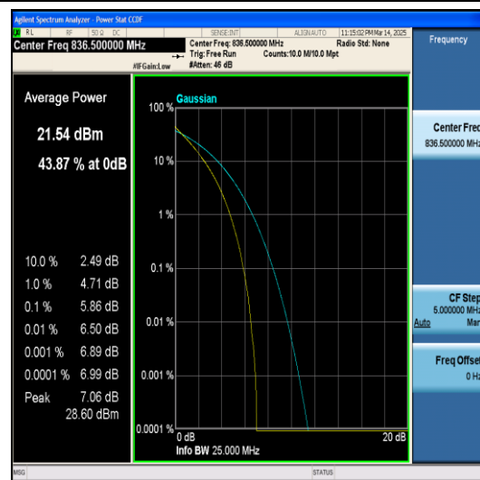
Band5-5MHz-QPSK-20525-25RB#0-PASS
