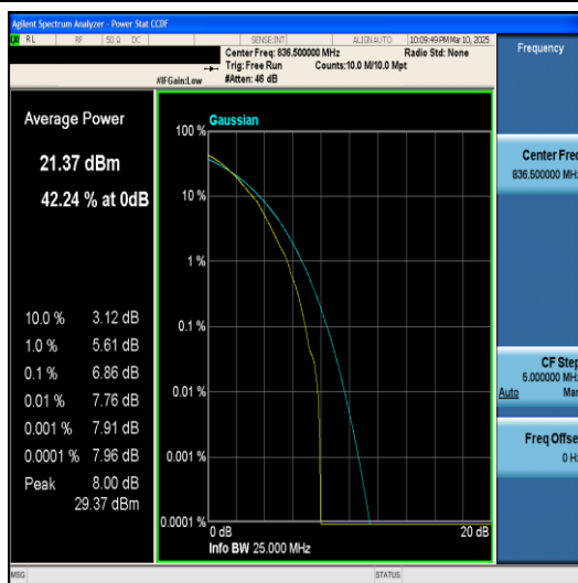
Band5-10MHz-64QAM-20525-1RB#0-PASS
