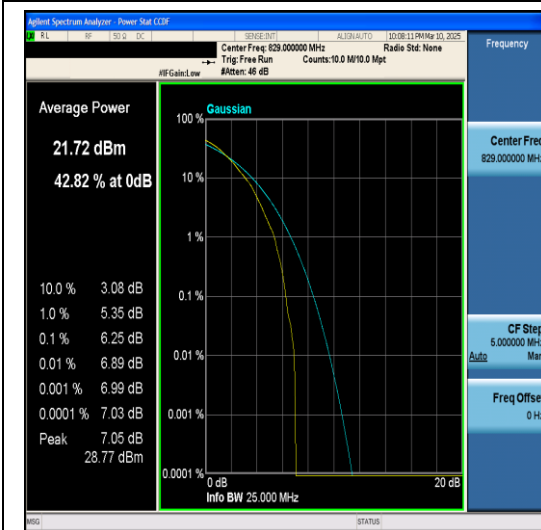
Band5-10MHz-64QAM-20450-1RB#0-PASS
