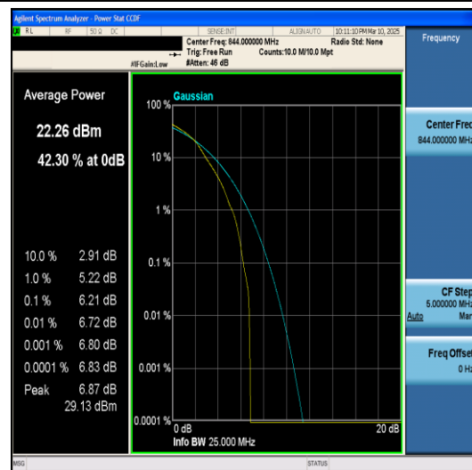
Band5-10MHz-QPSK-20600-50RB#0-PASS
