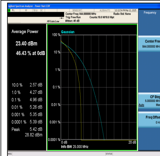
Band5-10MHz-64QAM-20600-1RB#0-PASS
