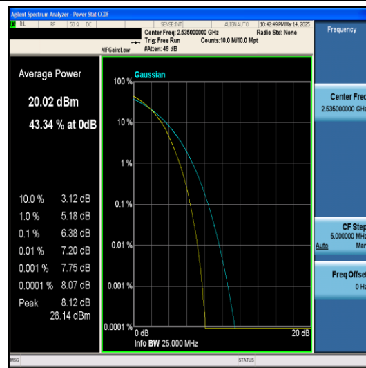
Band7-10MHz-16QAM-21400-1RB#0-PASS
