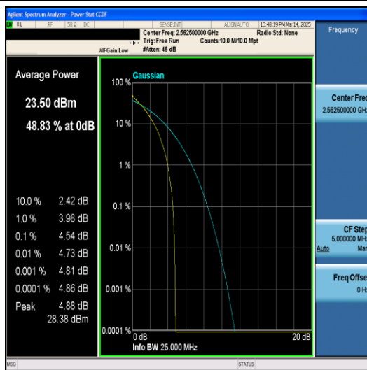
Band7-15MHz-64QAM-21375-1RB#0-PASS
