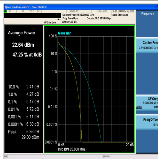
Band7-20MHz-QPSK-20850-100RB#0-PASS
