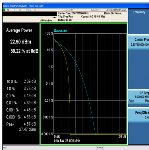
Band7-15MHz-64QAM-20825-1RB#0-PASS
