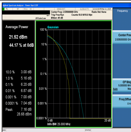
Band7-10MHz-64QAM-21100-1RB#0-PASS
