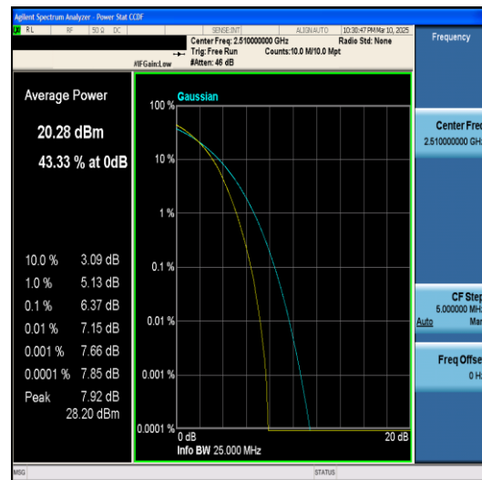
Band7-20MHz-16QAM-21100-1RB#0-PASS
