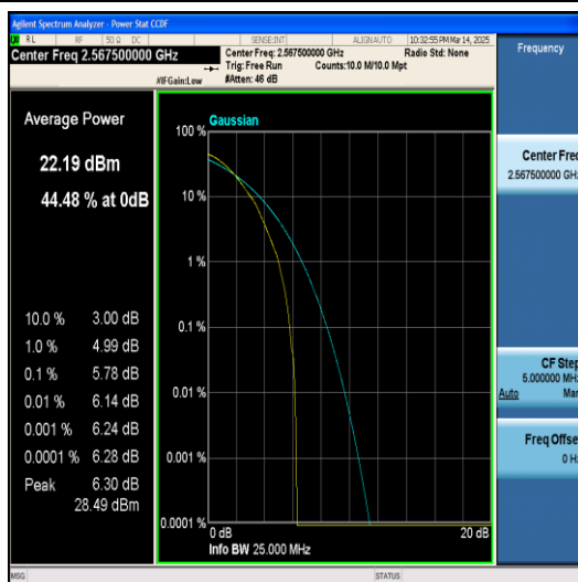
Band7-5MHz-64QAM-21425-1RB#0-PASS
