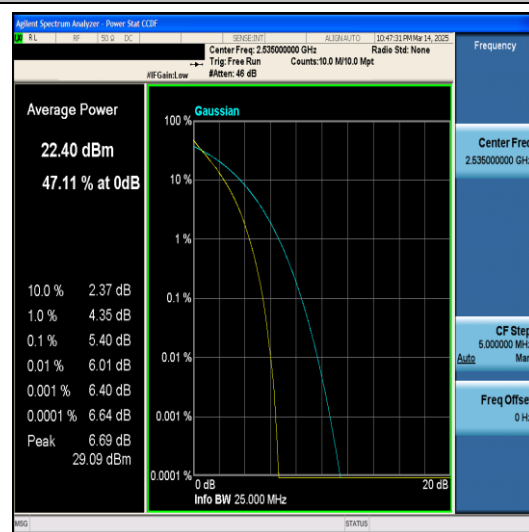
Band7-15MHz-QPSK-21100-75RB#0-PASS
