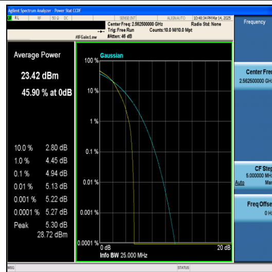
Band7-15MHz-QPSK-21375-75RB#0-PASS
