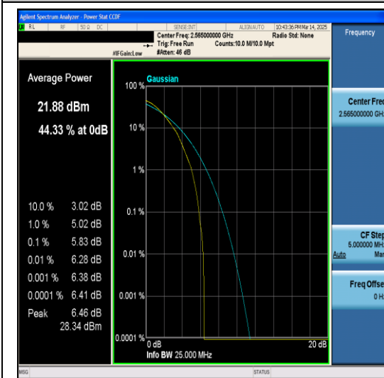
Band7-10MHz-64QAM-21400-1RB#0-PASS
