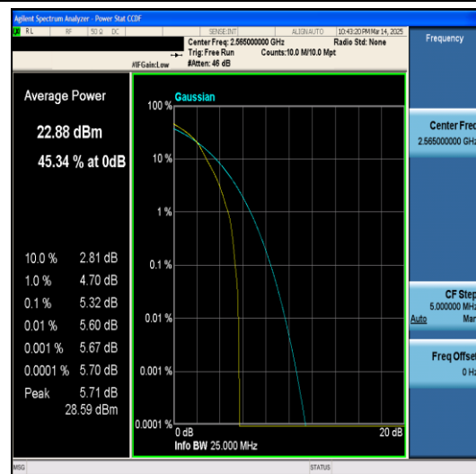
Band7-10MHz-QPSK-21400-50RB#0-PASS
