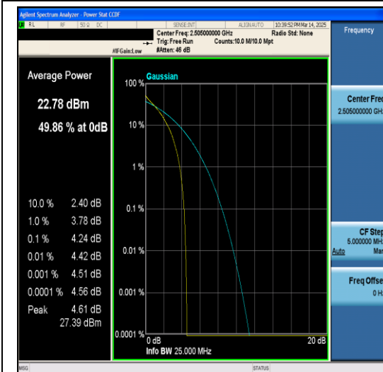
Band7-10MHz-64QAM-20800-1RB#0-PASS
