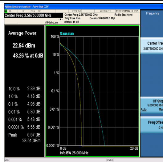
Band7-5MHz-QPSK-21425-25RB#0-PASS
