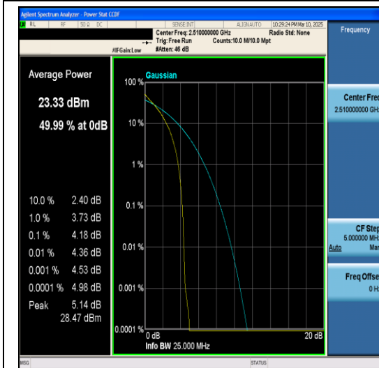
Band7-20MHz-64QAM-20850-1RB#0-PASS
