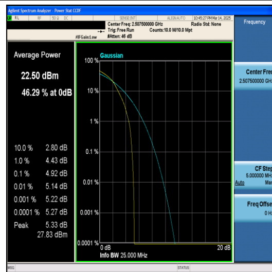
Band7-15MHz-QPSK-20825-75RB#0-PASS
