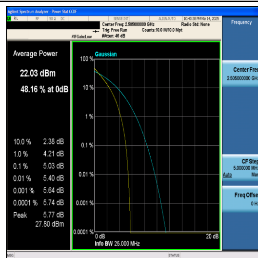
Band7-10MHz-QPSK-20800-50RB#0-PASS
