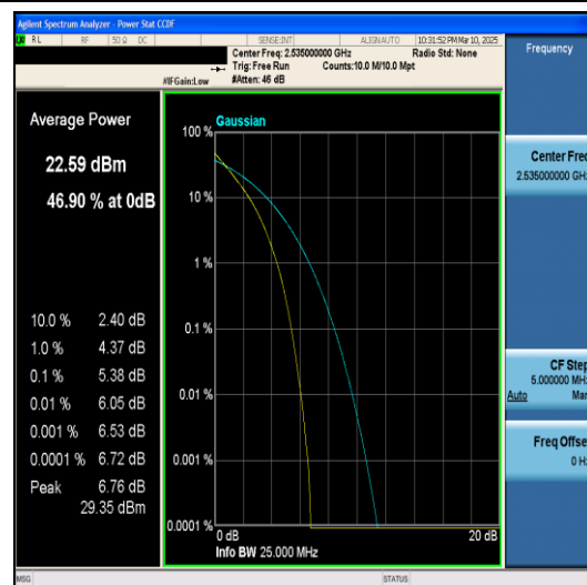
Band7-20MHz-QPSK-21100-100RB#0-PASS
