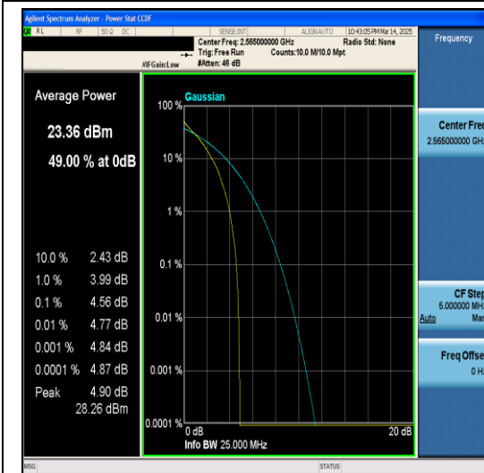
Band7-10MHz-64QAM-21400-1RB#0-PASS
