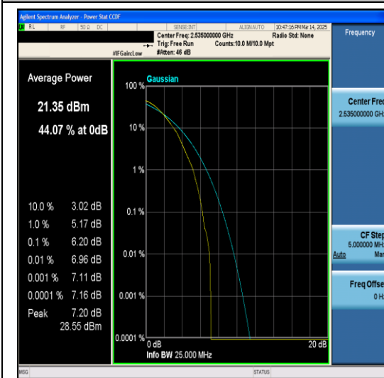
Band7-15MHz-64QAM-21100-1RB#0-PASS
