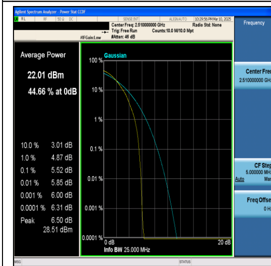
Band7-20MHz-64QAM-20850-1RB#0-PASS
