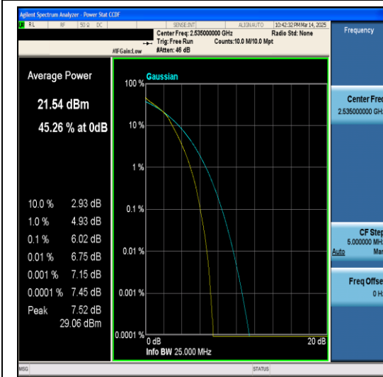
Band7-10MHz-QPSK-21400-1RB#0-PASS
