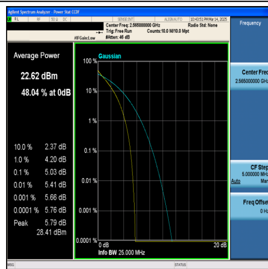
Band7-10MHz-QPSK-21400-50RB#0-PASS
