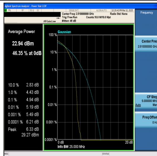
Band7-20MHz-QPSK-20850-100RB#0-PASS
