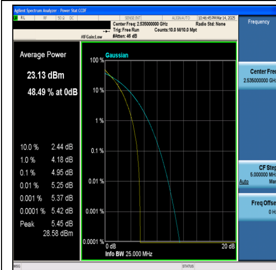
Band7-15MHz-64QAM-21100-1RB#0-PASS
