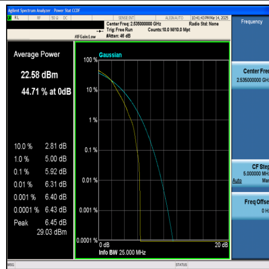
Band7-10MHz-QPSK-21100-50RB#0-PASS
